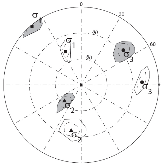
FIGURE 2.2.11: Principal stress directions determined with Julien and Cornet's method using the reduced dataset. Two minima are found. The solution A yields the principal stress directions with the confidence regions unfilled and the solution B yields the principal stress directions with the confidence regions in grey. See figure 2.2.7 for a description of the figure.
