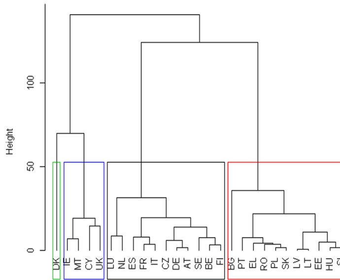
Cluster Dendrogram
