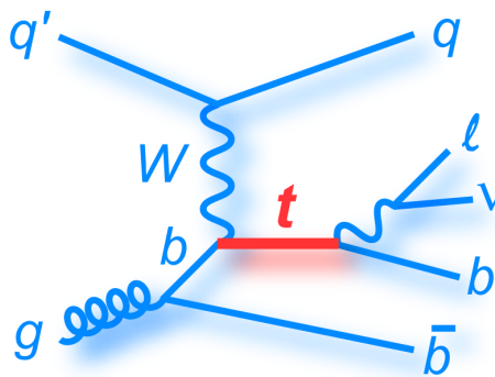
Figure 6-1: Feynman diagram ( 2 \rightarrow 3 process) for single top quark t -channel production and leptonic decay.
