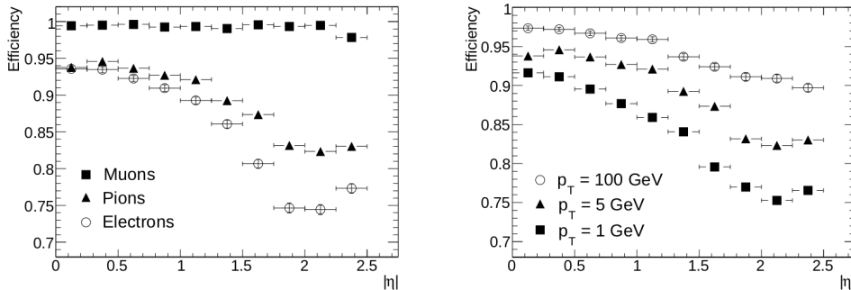
Figure 4-8: The track efficiencies of the inner detector. On the left, track reconstruction efficiencies as a function of |\eta| for muons, pions and electrons with p_T = 5 \text{ GeV} . The inefficiencies for pions and electrons reflect the shape of the amount of material in the inner detector as a function of |\eta| . On the right, Track reconstruction efficiencies as a function of |\eta| for pions with p_T = 1, 5 and 100 \text{ GeV} .
