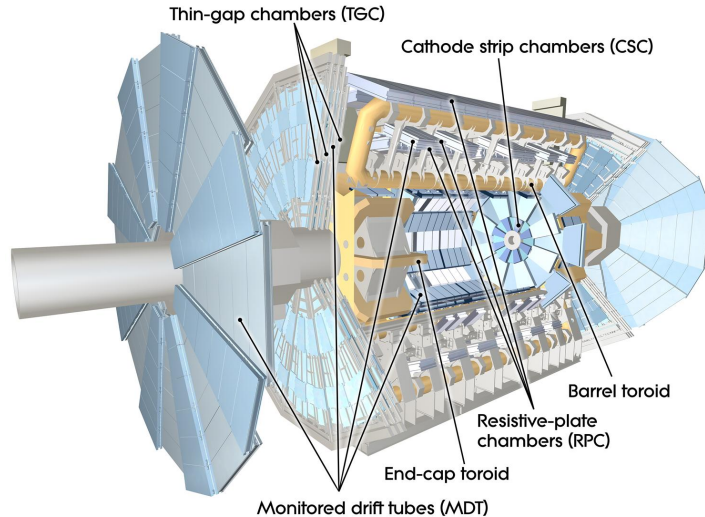
Figure 4-14: The ATLAS muon spectrometer
