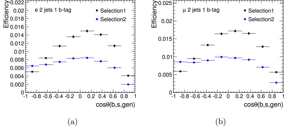
Figure 9-10: Efficiency curves, \epsilon(\cos\theta_{parton})=N_{reco}/N_{parton} , calculated with the AC-ERMC generator as a function of the parton-level angle of the b -quark jet in the spectator basis for the (a) electron and (b) muon channels. The events are selected with the SELECTION-1 (black points) and SELECTION-2 (blue points) cuts. The efficiency curves are defined using eight angular bins.
