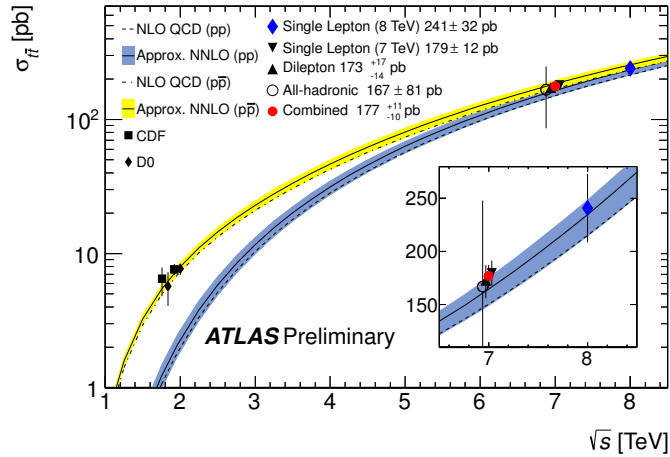
Figure 3-6: Measured cross sections for top quark pair production in hadron colliders (Tevatron and LHC) as a function of the center of mass energy with comparison to theoretical calculations [50].
