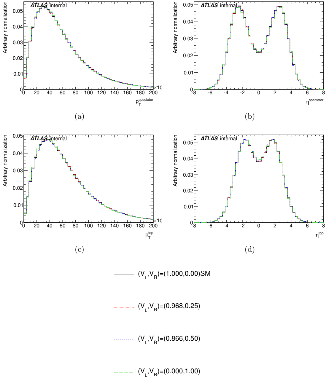
Figure 7-7: Comparison of the parton-level kinematic distributions for PROTON events produced with the Standard Model (black solid lines) and anomalous (colored dashed lines) couplings configured in both production and decay vertices (a) spectator quark transverse momentum, (b) spectator quark pseudorapidity, (c) top quark transverse momentum and (d) top quark pseudorapidity. The color code with the corresponding anomalous configurations are given in the legend. The distributions are shown for the electron channel.
