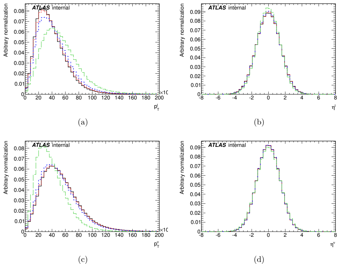
Figure 7-9: Comparison of the parton-level kinematic distributions of the W boson decay products for PROTOS events produced with the Standard Model (black solid lines) and anomalous (colored dashed lines) couplings configured in both production and decay vertices. (a) lepton transverse momentum, (b) lepton pseudorapidity, (c) neutrino transverse momentum and (d) neutrino pseudorapidity. The color code and the corresponding anomalous configurations are the same than in Figure 7-8. The distributions are shown for the electron channel.
