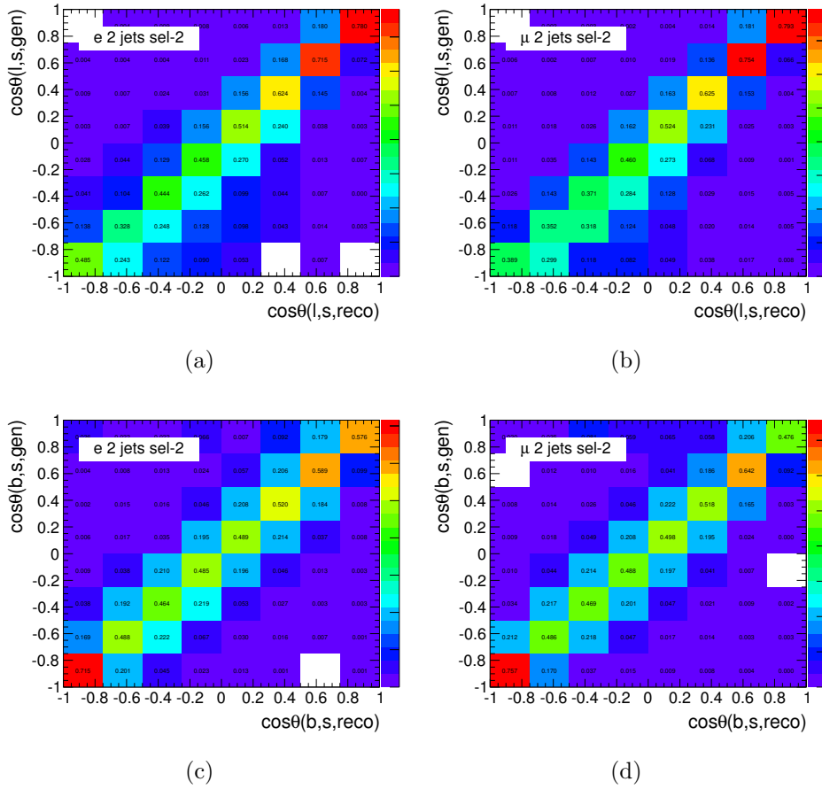
Figure 9-8: Migration matrices R(\cos \theta_{reco}, \cos \theta_{parton}) calculated with the ACERMC generator in the spectator basis for events selected with the SELECTION-2 cuts (a) charged lepton in the electron channel, (b) charged lepton in the muon channel, (c) b -quark jet in the electron channel and (d) b -quark jet in the muon channel. The migration matrices are defined using eight angular bins.
