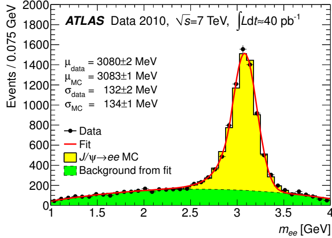
Figure 5-9: Reconstructed dielectron invariant mass distribution for J/\psi \rightarrow ee events after applying the baseline energy calibration. The data are compared to the sum of the Monte Carlo signal (light filled histogram) and background contributions (darker filled histogram) modelled by a Chebyshev polynomial. The mean value and the Gaussian width of the fitted Crystal Ball function are given for both data and MC [106].
