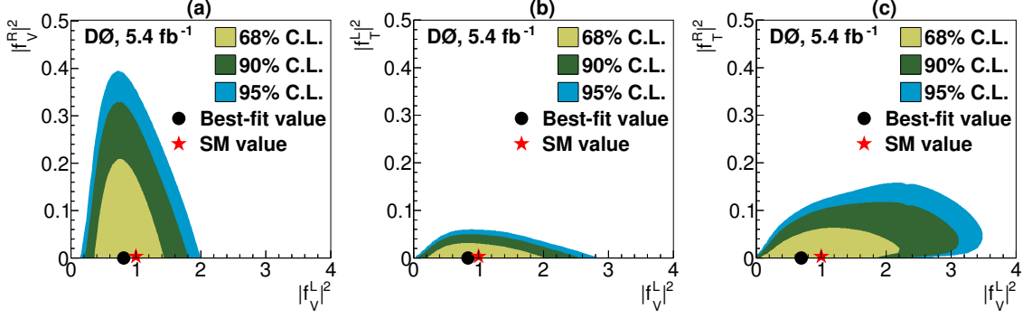
Figure 3-14: Two-dimensional posterior probability density distributions for the anomalous coupling configurations (V_L, V_R) , (V_L, g_L) , (V_L, g_R) extracted from the combination of the single top quark cross section measurements and the W boson helicity fractions measurements in t\bar{t} production. The points represent the data and the red stars the Standard Model predictions.
