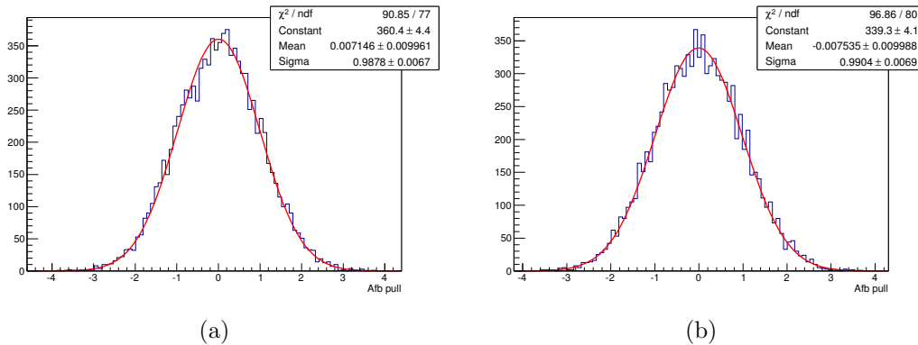
Figure 9-13: Pull distributions of the forward-backward asymmetries unfolded with a simple matrix inversion for (a) the lepton and (b) the b -quark jet spin analyzers.
