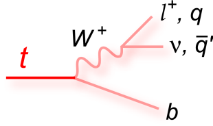
Figure 3-4: Feynman diagram for the electroweak top quark decay with the leptonic and hadronic decays of the W boson.
