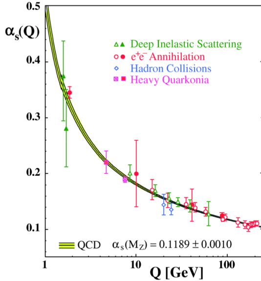
Figure 3-1: Measurements of the strong coupling constant \alpha_s as a function of the interaction energy scale Q . Open symbols indicate resummed NLO and filled symbols NNLO QCD calculations used in the various measurements. The curves correspond to the QCD predictions for the combined world average value of \alpha_s at the Z -pole mass [33].
