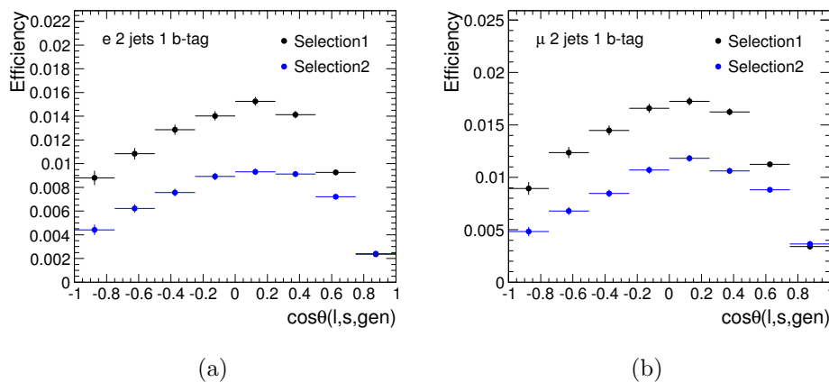
Figure 9-9: Efficiency curves, \epsilon(\cos\theta_{parton})=N_{reco}/N_{parton} , calculated with the ACERMC generator as a function of the parton-level angle of the charged lepton in the spectator basis for the (a) electron and (b) muon channels. The events are selected with the SELECTION-1 (black points) and SELECTION-2 (blue points) cuts. The efficiency curves are defined using eight angular bins.
