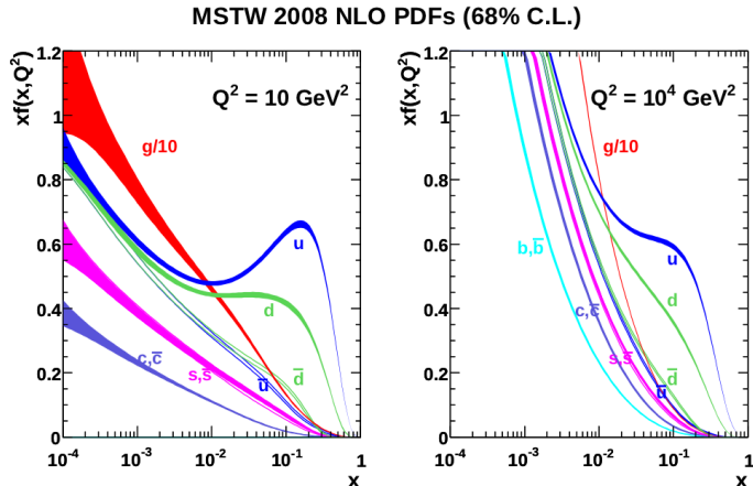
Figure 3-3: Parton distribution functions of the MSTW 2008 NLO set for the squared energy transfers Q^2 of 10 \text{ GeV}^2 and 10^4 \text{ GeV}^2 at the LHC.
