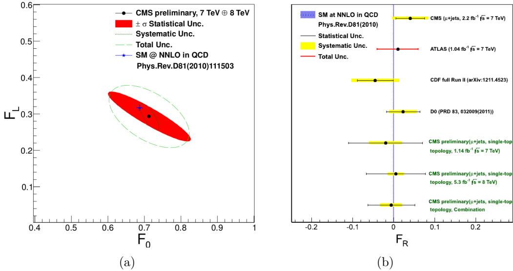
Figure 3-12: (a) W boson helicity fractions F_0 and F_L measured by the CMS collaboration from single top quark events by combining data recorded at 7\text{ TeV} and 8\text{ TeV} center-of-mass energies, (b) Comparison of the helicity fraction F_R measured by CMS from single top quark events with all measurements carried out at the Tevatron and at the LHC from top quark pair events.
