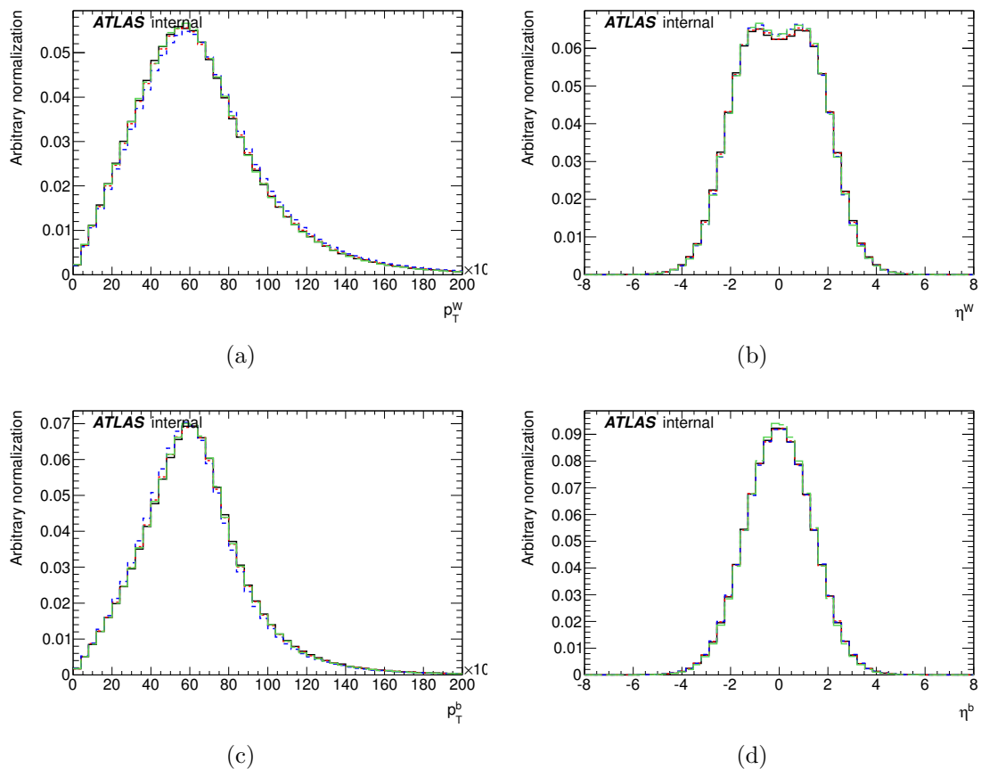
Figure 7-8: Comparison of the parton-level kinematic distributions of the top quark decay products for PROTOS events produced with the Standard Model (black solid lines) and anomalous (colored dashed lines) couplings configured in both production and decay vertices. (a) W boson transverse momentum, (b) W boson pseudorapidity, (c) b -quark transverse momentum and (d) b -quark pseudorapidity. The color code and the corresponding anomalous configurations are the same than in Figure 7-8. The distributions are shown for the electron channel.
