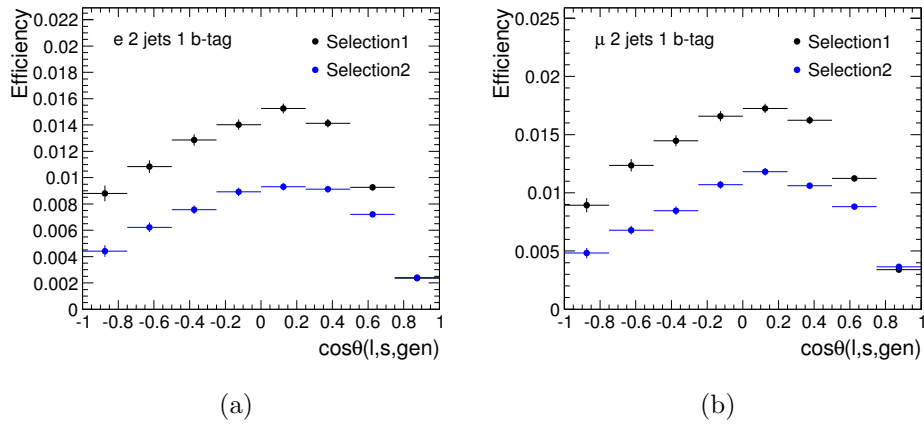
Figure 9-9: Efficiency curves, \epsilon(\cos\theta_{parton}) = N_{reco}/N_{parton} , calculated with the ACERMC generator as a function of the parton-level angle of the charged lepton in the spectator basis for the (a) electron and (b) muon channels. The events are selected with the SELECTION-1 (black points) and SELECTION-2 (blue points) cuts. The efficiency curves are defined using eight angular bins.
