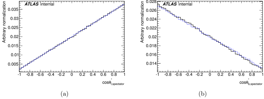
Figure 7-4: Comparison between the angular distributions calculated in the spectator basis for ACERMC (solid lines) and PROTOS (dashed lines) events in the electron channel (a) lepton spin analyzer and (b) b -quark spin analyzer. The spectator basis is defined along the spectator quark momentum. The spin analyzer and the spin basis are both boosted to the top quark rest frame. The PROTOS generator is configured using the Standard Model values for the Wtb couplings.
