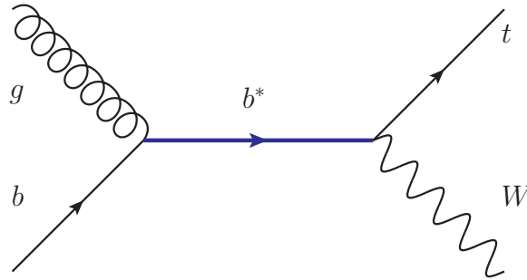
Figure 3-18: Feynman diagram for the production of an excited b^* -quark decaying into a W boson and a top quark.
