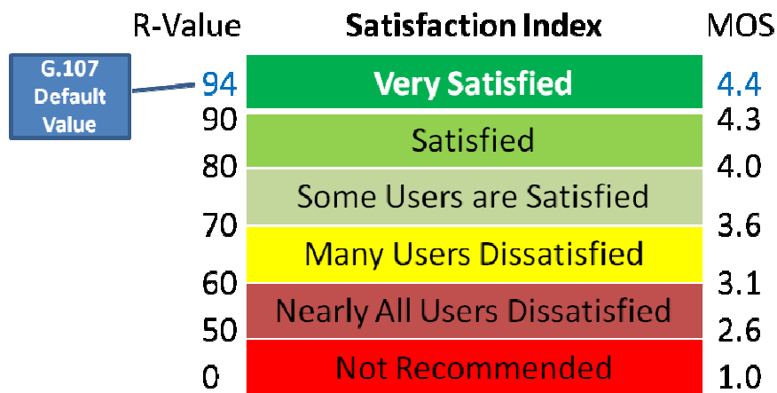
Figure 13: E-Model and R-factor [105]
