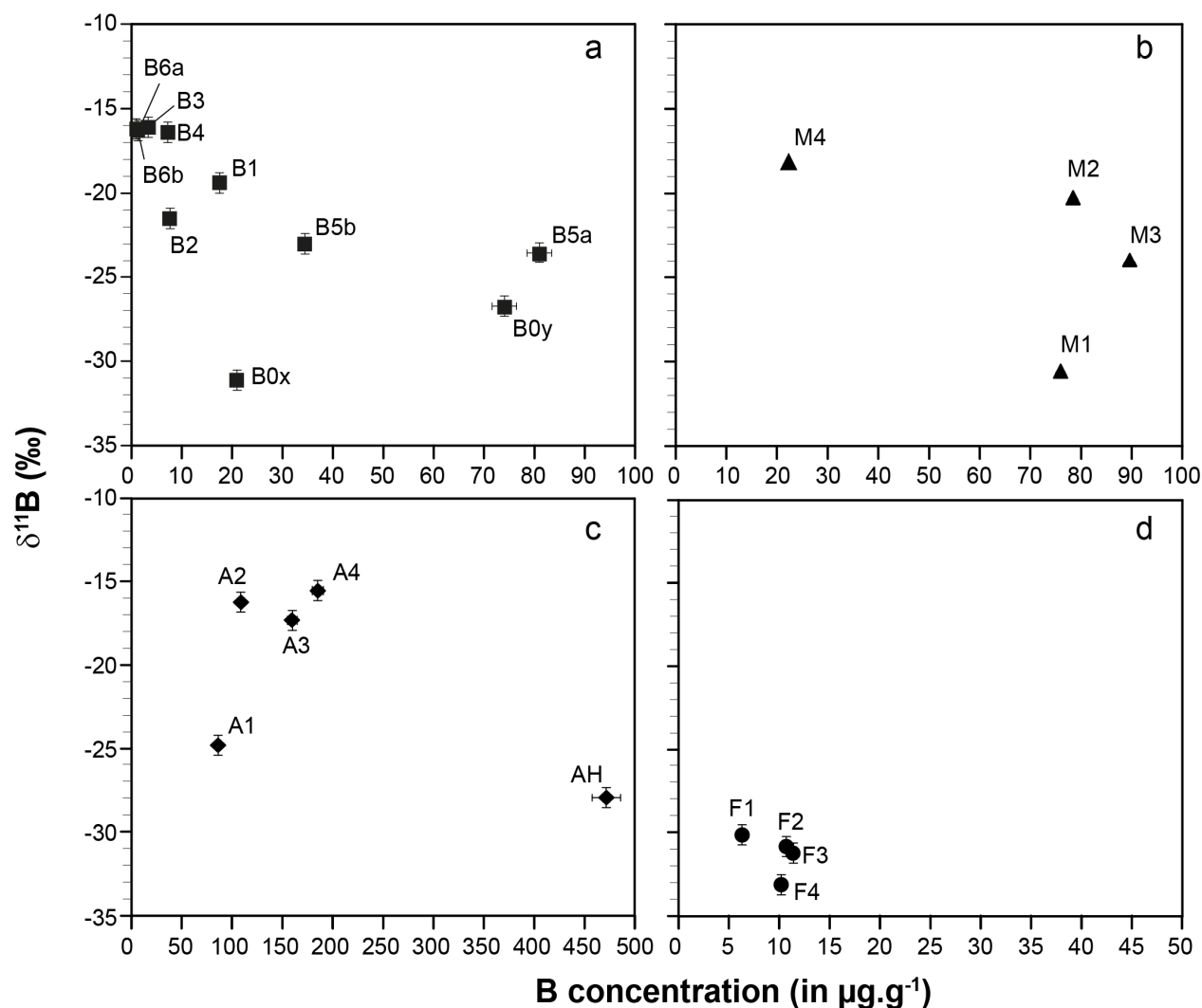
Figure IV-2: Boron chemical and isotopic compositions in the different mineral assemblages (see table IV-3 for abbreviations).
