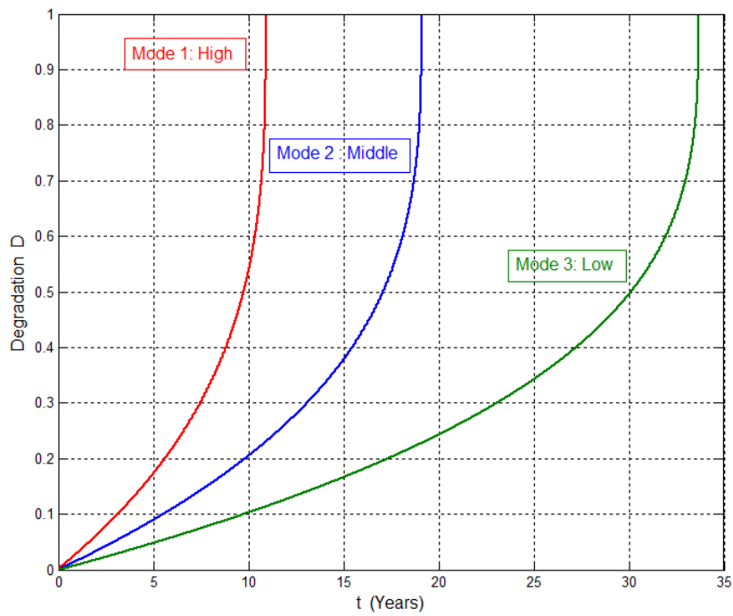
Figure 3.35 - Pipelines degradation under three modes of pressure for nonlinear law (offshore pipes).
