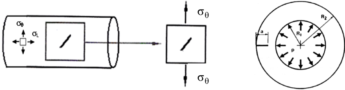
Figure 2.32 - Crack length in radial direction.
