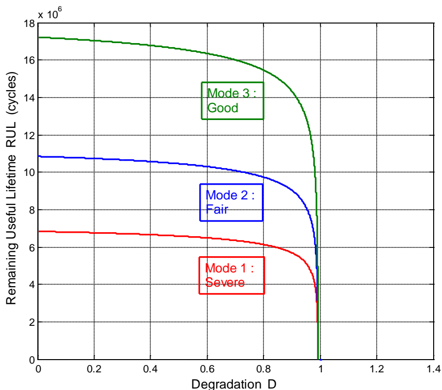
Figure 2.26 - Remaining Useful Lifetimes estimated by the prognostic model.
