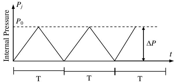
Figure 2.33 - Triangular simulation of internal pressure
