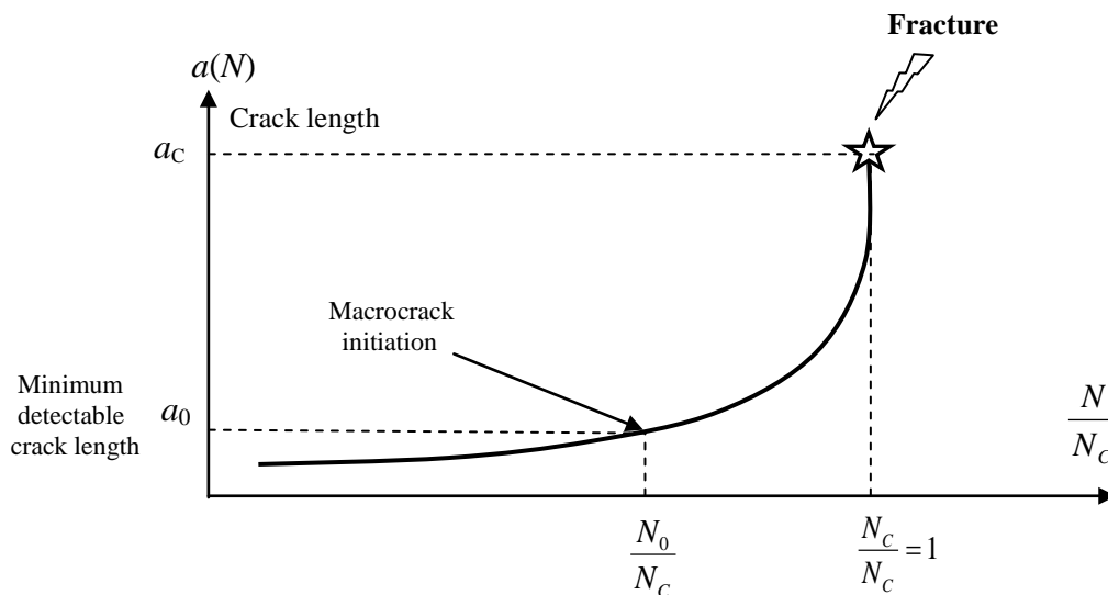
Figure 2.2 - Pre-Crack fatigue damage.
