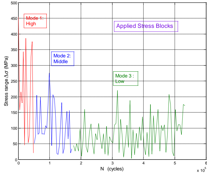
Figure 4.31 - Applied stress blocks on pipes for three modes of pressure.
