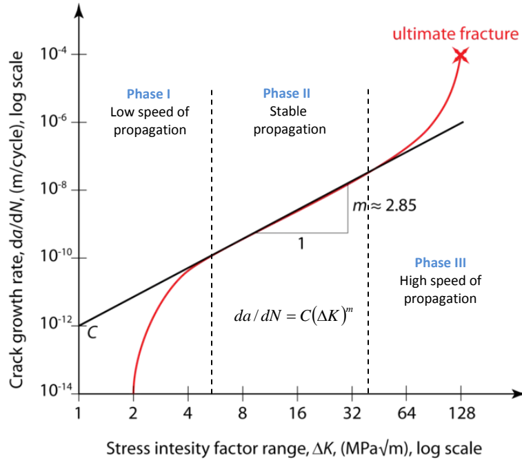
Figure 2.4 - The three phases of crack growth, Paris-Erdogan's law.
