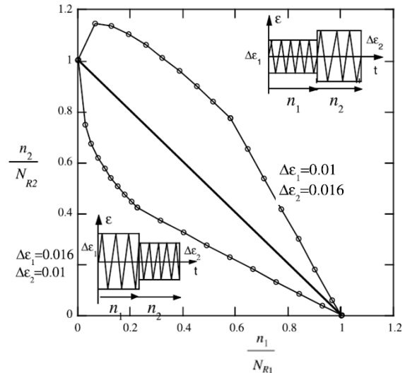
Figure 3.2 - Nonlinear damage accumulation.
