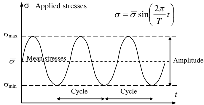
Figure 2.6 - Cyclic applied stresses.
