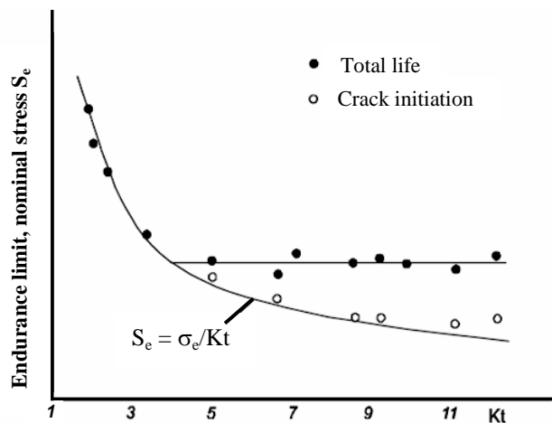
Figure 2.13 - Relationship between endurance limit stress \sigma_e and the stress concentration factor K_t for crack initiation and total life.
