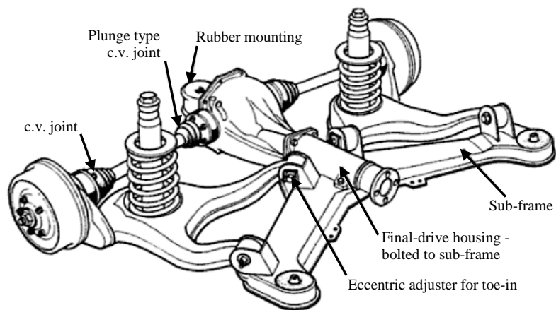
Figure 2.11 - Vehicle suspension system.
