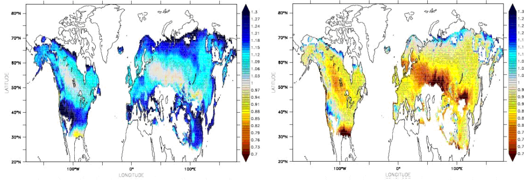
Figure 4.7: Evolution of wheat yield in % between the periods 2070-2100 and 2000-2030 with climate and CO 2 fertilisation (left graph) and climate only (right graph). Source: Viovy et al. (2010)
