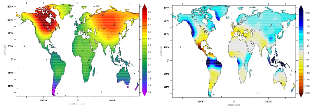
Figure 4.6: Evolution of temperatures (left graph in °C) and precipitations (right graph in mm/year) in the IPSL-CM4 A1B scenario
