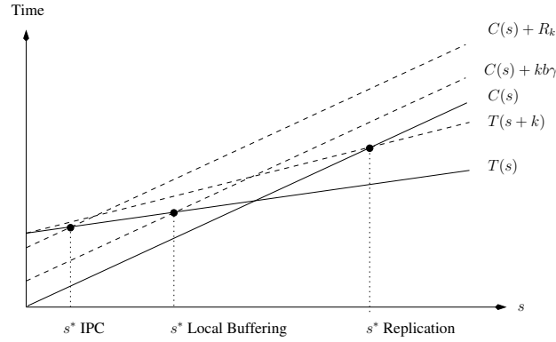
Figure 4.5: Comparing optimal granularity between strategies.
