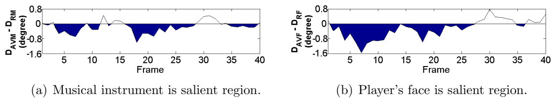
Figure 4.11: Average distance ((a) distance from Musical instrument ( D_{AVM}-D_{RM} ), and (b) distance from Face of the player ( D_{AVF}-D_{RF} )) for 4 clip snippets of music class over time.
