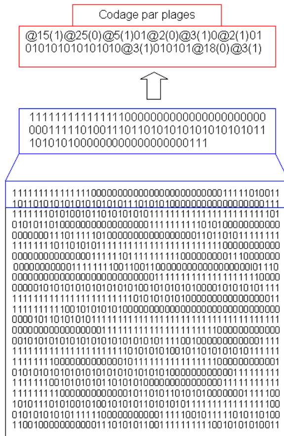
Figure 3.21 – Illustration du codage RLE
