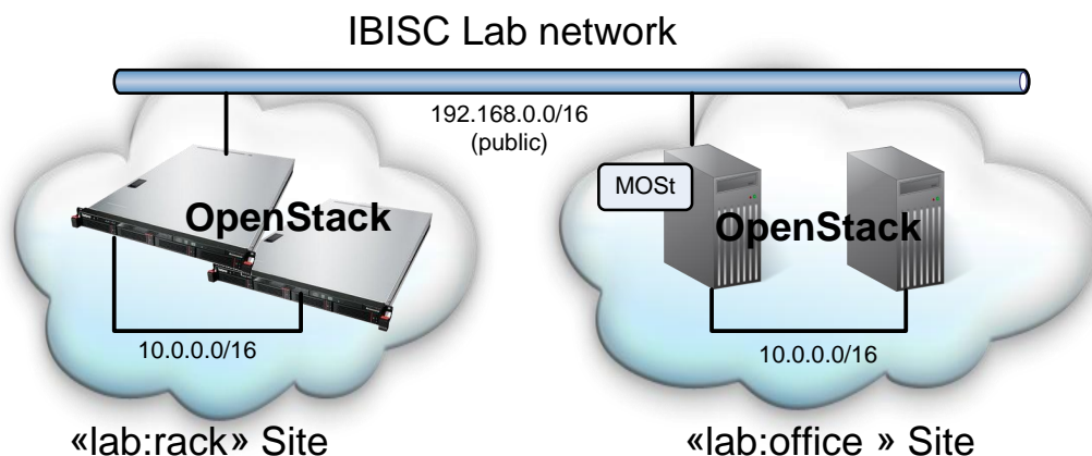
Figure 5.8: Testbed platform
