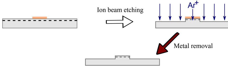
Figure 2.2: Description of an etching step. After deposition of a metal layer (Aluminium), the sample is etched using IBE (Ion Beam Etching). The metal acts as a mask and only the part of the surface not covered by the metal is etched. Afterwards the metal is removed.
