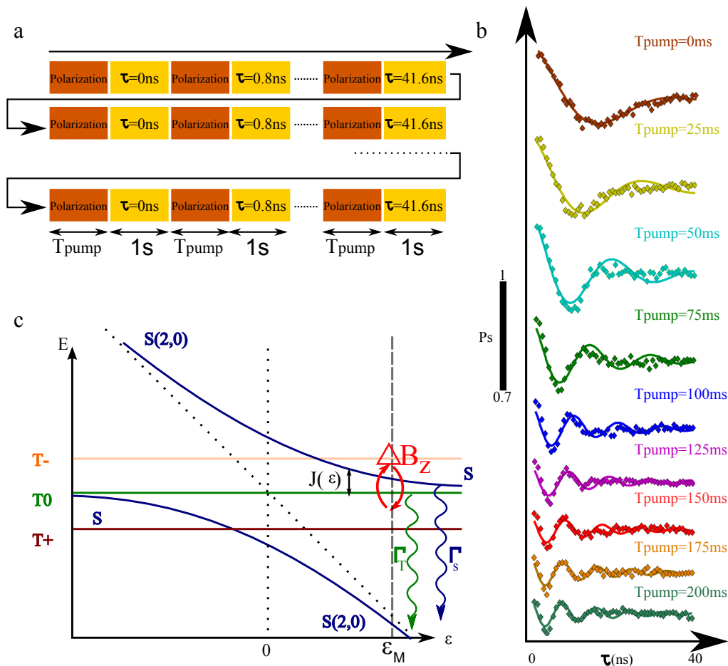
Figure 4.11: S - T_0 oscillations induced by a nuclear magnetic field gradient \Delta B_z . (a) Measurement scheme : Each measurement point of figure 4.11 (b) is an average over 1s, and it is preceded by a polarization pulse running for T_{pump} . In addition, in order to average the signal, this is repeated 50 times for a fixed value of T_{pump} . (b) S - T_0 coherent oscillations for different polarization times T_{pump} . The singlet probability is plotted with respect to \tau , the time spent in the \varepsilon \ll 0 region. (c) Relaxation at the measurement point induced by a finite gradient \Delta B_z . At the measurement point, the exchange energy can become smaller than the gradient \Delta B_z under polarization. This induces a mixing between the blockaded triplet |T_0\rangle and the singlet |S\rangle . Then the relaxation is possible via a spin conserving phonon emission. This relaxation is quite faster compared to the thermal relaxation through the reservoir.
