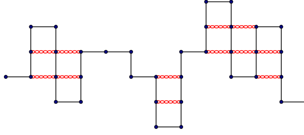
FIGURE 2.4 – A partially directed walk with 12 self-touchings represented by red bonds.
