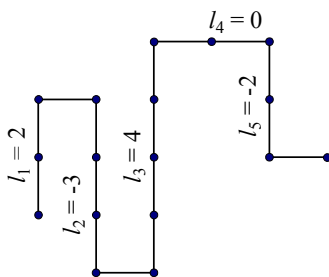
FIGURE 2.5 – An example trajectory with N = 5 vertical stretches and length L = 16 .
