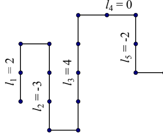
FIGURE 3.4 – An example of decomposition of w \in \mathcal{W}_{16} into 5 stretches.
