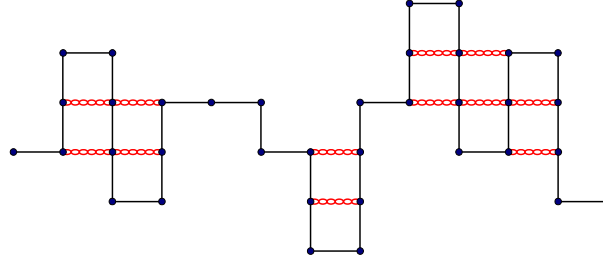
FIGURE 4.1 – Example of a trajectory with 12 self-touchings in light red.
