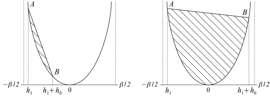
FIGURE 4.5 – The hatched domain corresponds to |\mathcal{A}(h_0, h_1)| .
