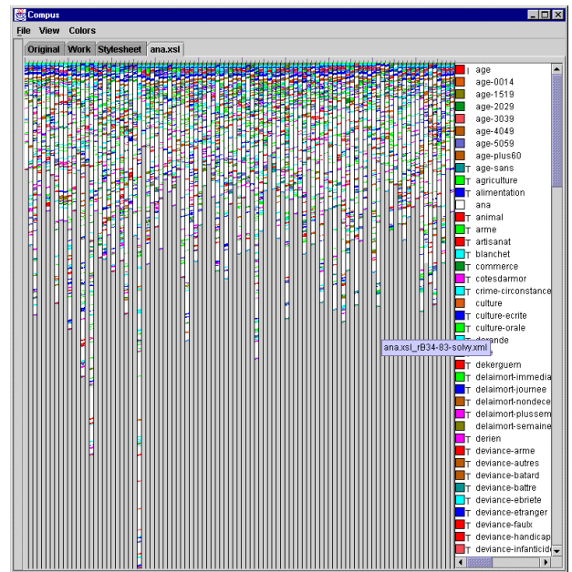
Figure 5: Visualization of the transformed corpus, i.e. analytical view of figure 2.
