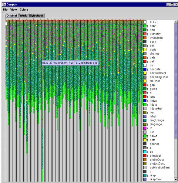
Figure 2: The Compus System showing a corpus of 100 structured documents.
