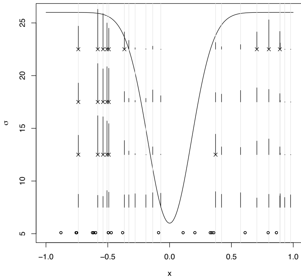
FIGURE 3.5 – Same as Figure 3.4, but for GP parameters following (3.10) and the solid line corresponds to the hidden true scale parameter \sigma(x) .
