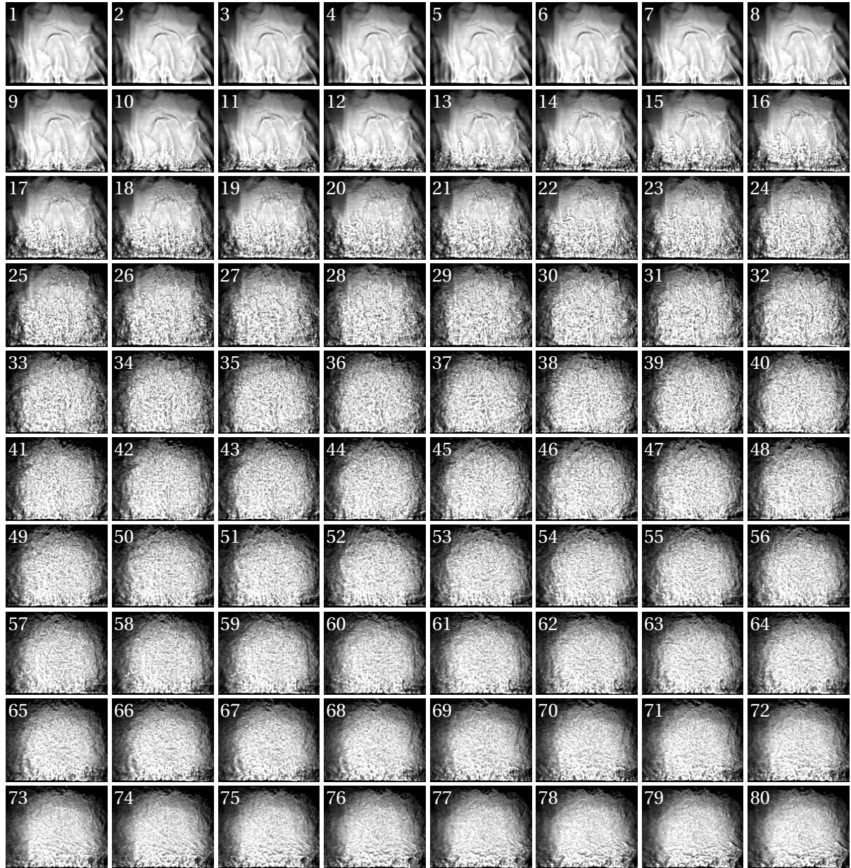
Figure 4.4: Detailed representation of the transient behaviour of convective structures after a 43 kV/cm electric field is applied ( \Delta T_W \approx 30 K, \Delta t = 3 ms between two images). Picture width is about 8 mm.
