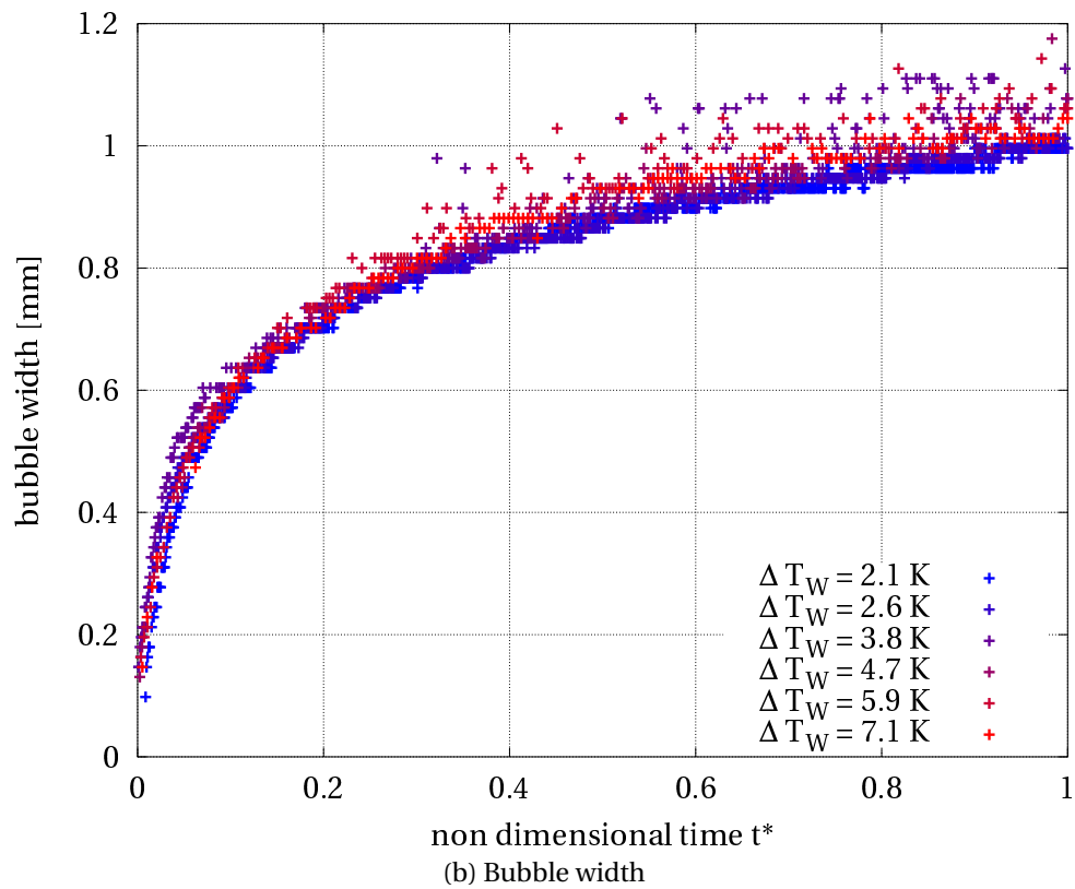
Figure 5.16: Bubble height and width for several wall superheat
