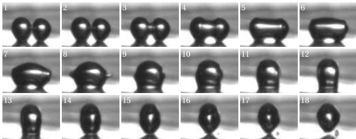
Figure 5.66: Photos of lateral coalescence between adjacent bubbles coming from neighbour nucleation sites, at a high wall superheat of \Delta T_W \approx 6.5\ \text{K} . Time difference between two photos is \Delta t \approx 0.19\ \text{ms} .
