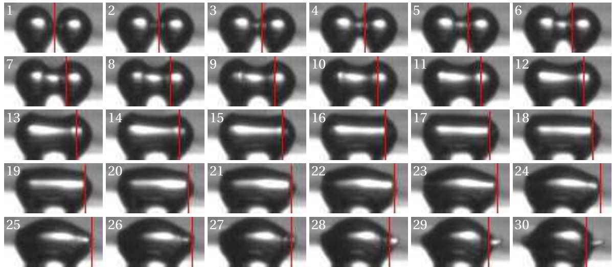
Figure 5.68: Photos of lateral coalescence between adjacent bubbles coming from neighbour nucleation sites, at a high wall superheat of \Delta T_W \approx 8.5 K. Time difference between two photos is \Delta t \approx 37 \mu\text{s} .
