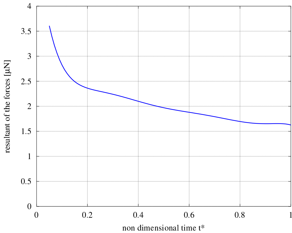
Figure 5.45: Resultant of the third buoyancy term acting on a bubble at \Delta T_W = 2.1 K.
