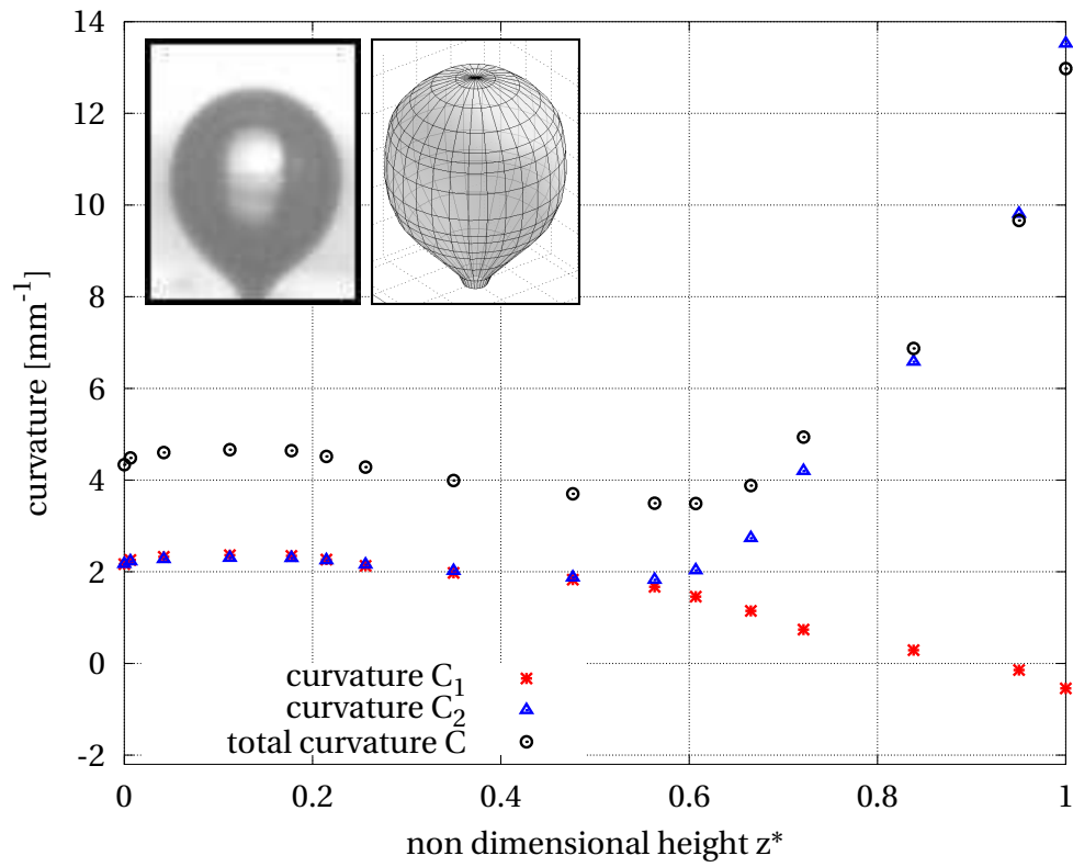
Figure 5.60: Curvature of the interface with \Delta T_W = 2.1 K and t^* = 99.9 %.
