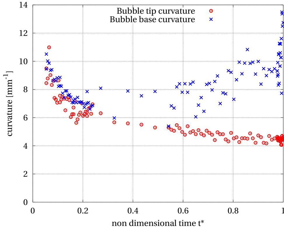
Figure 5.64: Bubble base and tip curvature during bubble growth with \Delta T_W = 2.1 K
