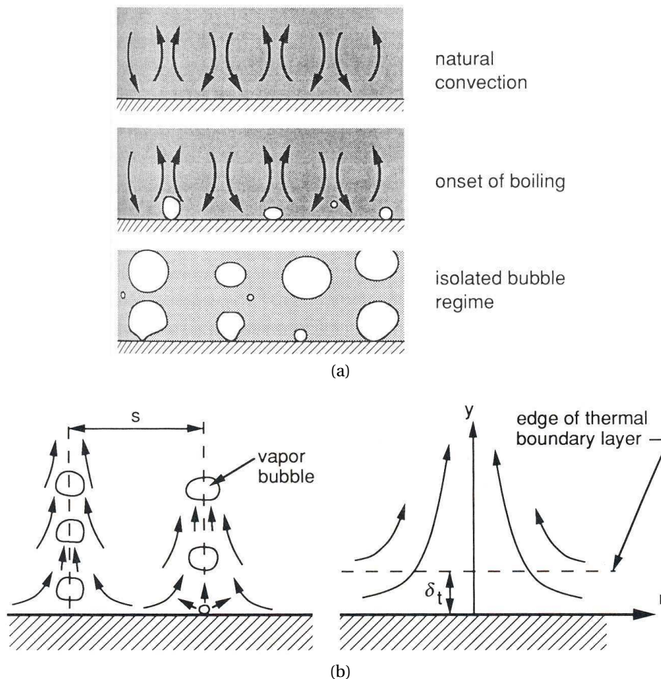
Figure 4.2: Schematic of boiling regimes (a) and fluid flows (b) at low superheat from (V.P. Carey [23])
