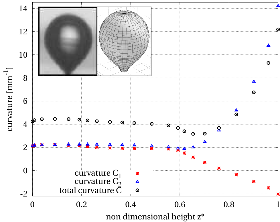
Figure 5.61: Curvature of the interface with \Delta T_W = 4.7 K and t^* = 99.9 %.
