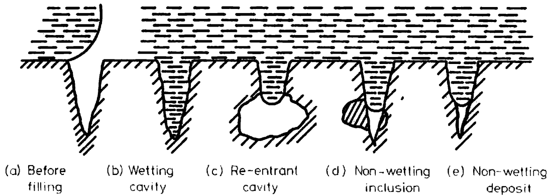
Figure 2.7: Formation of an active nucleation site in a real cavity. Illustration from Collier and Thome [41].
