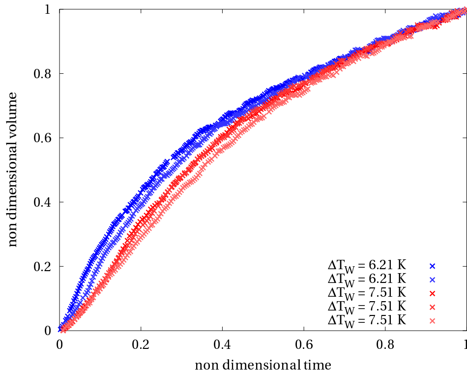
Figure G.2: Non dimensional bubble growth for different wall superheat conditions with an upper electrode voltage of 18 kV.
