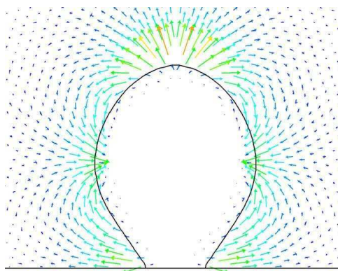
(a) Electric forces on the fluid particles
