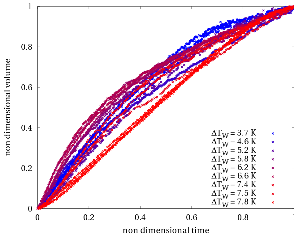
Figure 6.10: Non dimensional bubble growth in the presence of electric fields for different wall superheat conditions.
