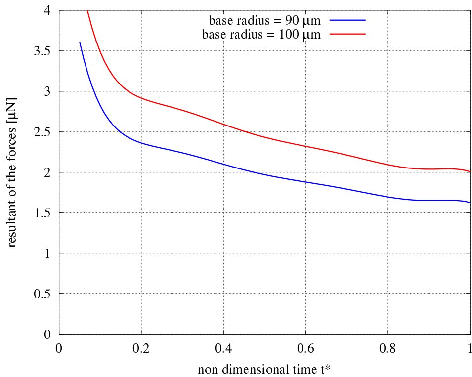
Figure 5.46: Resultant of the third buoyancy term acting on a bubble at \Delta T_W = 2.1 K, for two different base radii.
