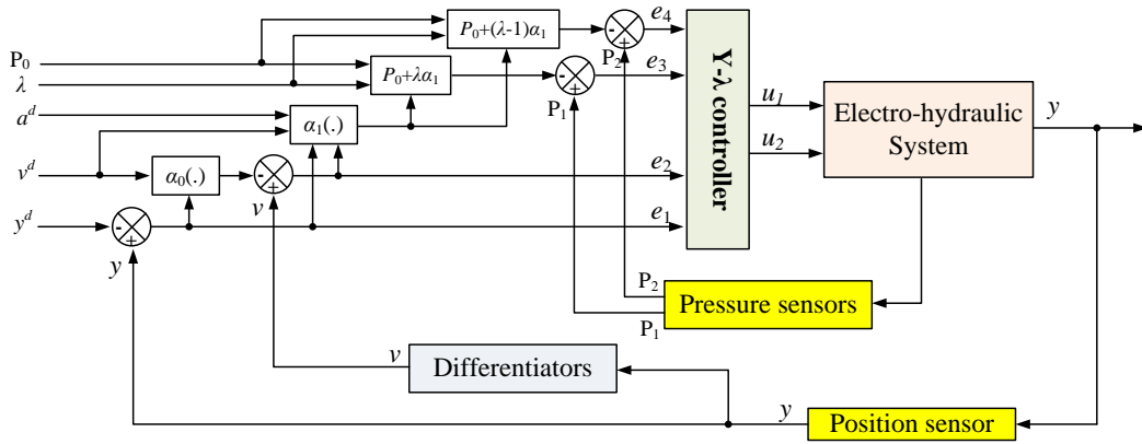
FIGURE 5.3: Schema of the Y-λ control law
