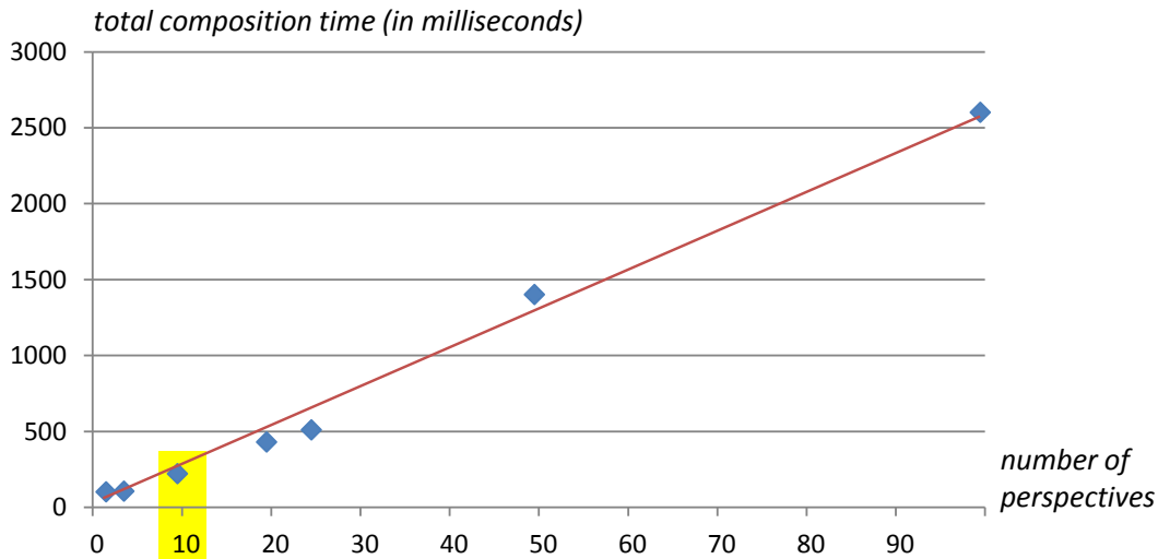
Figure 8-2. Total model composition time for 1 concept defined across 1 to 100 perspectives
