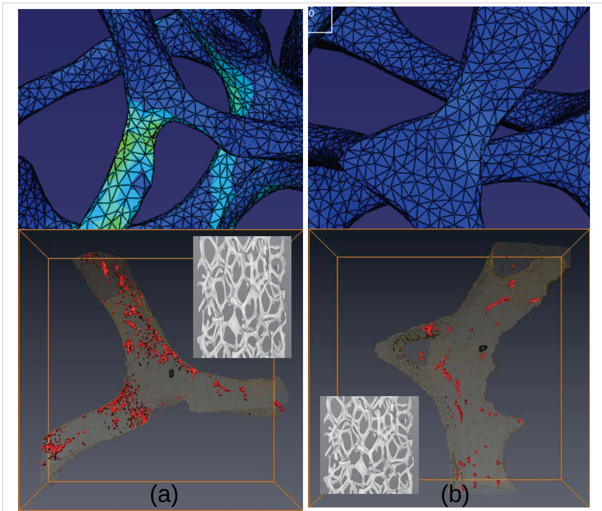
Fig. 7: Comparison between the FE calculation of the local stress and the internal distribution of inter-metallics and pores in moderately loaded struts (surrounded with a white circle in Fig. 6).
