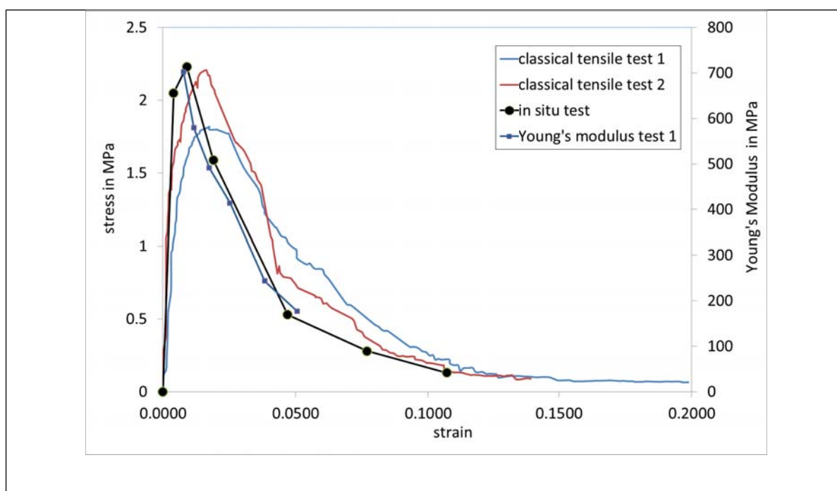
Figure 1a : stress-strain curve during classical tensile experiments of the random HS stacking and the curve recorded during the in situ experiments. The black points indicate strain where 3D images at low and high resolution were taken. Young’s modulus variation with strain is also plotted.
