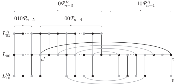
Figure 3.38: H. cycle in \Lambda_n - 10p'_{|V(\Gamma_{n-2})|}{}^{n-2} for n \equiv 2(\text{mod } 3)
