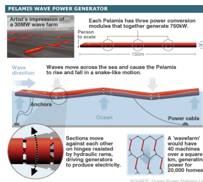
Figure 1.5. Pelamis – principe ©[PWP-09]
