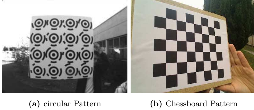
Figure 6.2: Patterns used for calibration of cameras.
