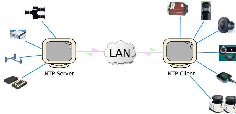
Figure 6.3: Two computers connected over LAN for synchronization using NTP and the sensors shared among them.
