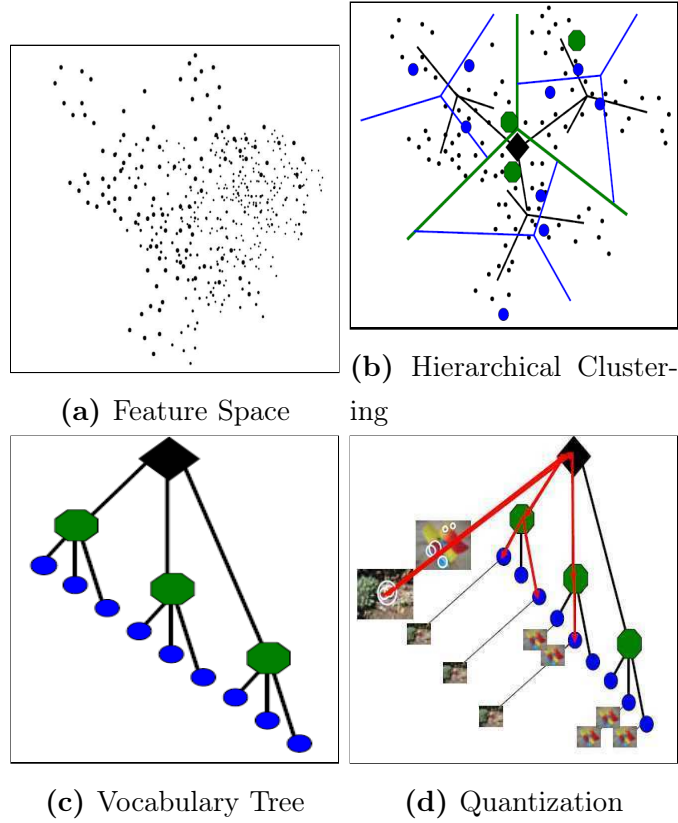
Figure 2.3: A toy example of vocabulary tree building. Figure 2.3a: A two dimensional feature descriptor space. Figure 2.3b: Hierarchical clustering of the feature space with two levels( l = 2 ) and a branching factor( k = 3 ). Top level clusters are represented by green circles and separated by green lines and similarly, the second level by blue. Figure 2.3c: A vocabulary tree representation of the hierarchical clusters. Figure 2.3d: Given query image patches, the leaf nodes to which the query patches are quantized is shown. (Figure courtesy of David Nister (NS06).)
