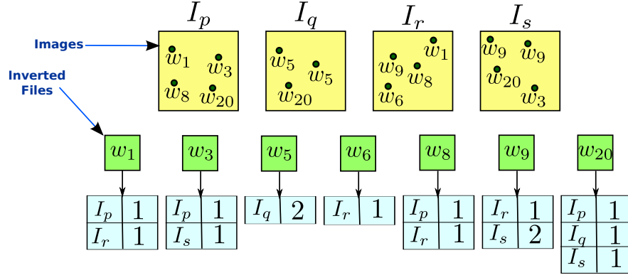
Figure 2.4: Inverted file representation for images. The first and second columns of a row of an inverted file contain the index of image in which the word occurred previously and the corresponding occurrence frequency respectively.
