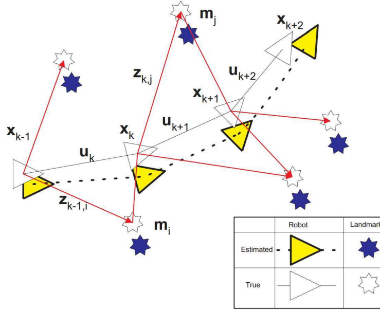
Figure 2.1: SLAM problem: Landmarks being observed at different positions along the robot's trajectory. Figure courtesy: Tim Bailey (DWB06)
