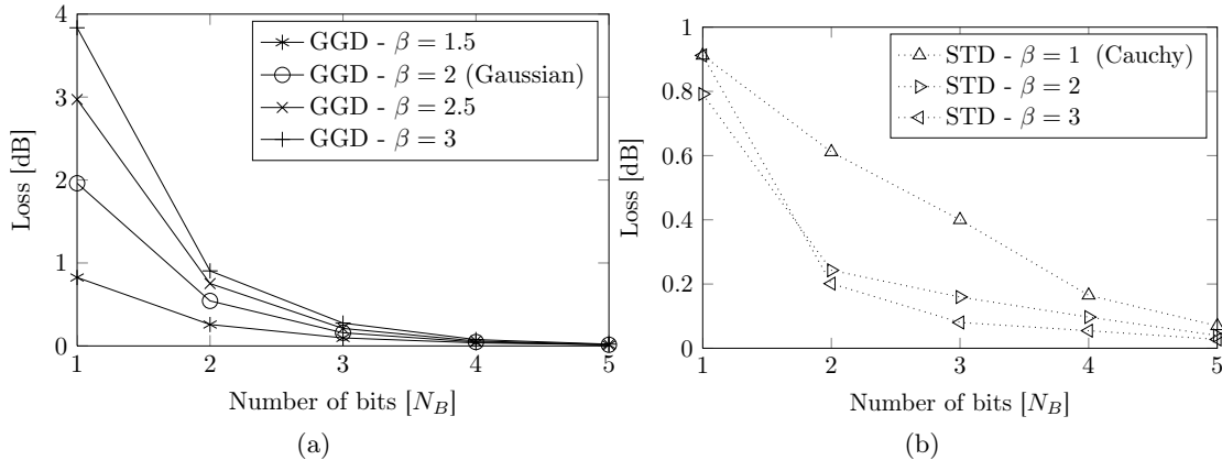
Figure 3.4: Adaptive algorithm loss of estimation performance due to quantization of measurements corresponding to the constant case L_q (theoretical). The loss is evaluated for different types of noise, GGD noise in (a) and STD noise in (b), and different numbers of quantization bits. For the other models of parameter studied here, the loss is proportional to L_q .
