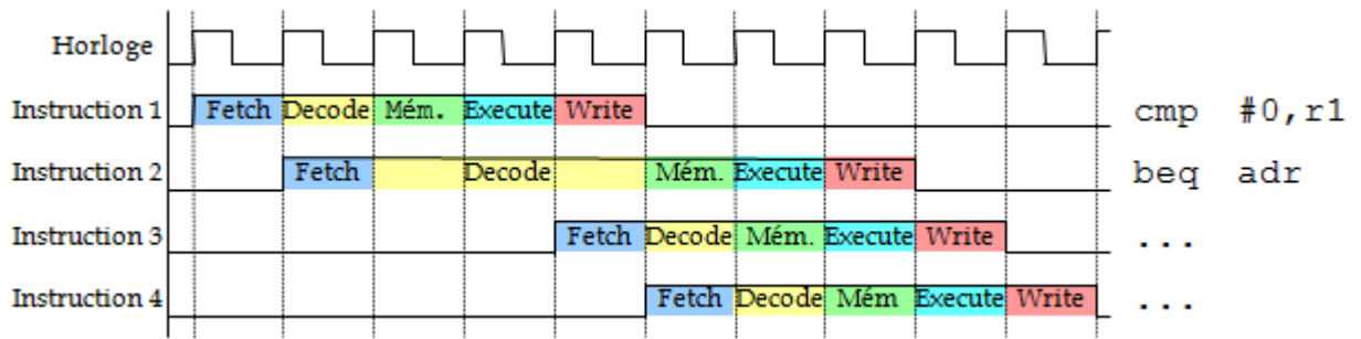
Figure 2-6 : Pipeline stall
