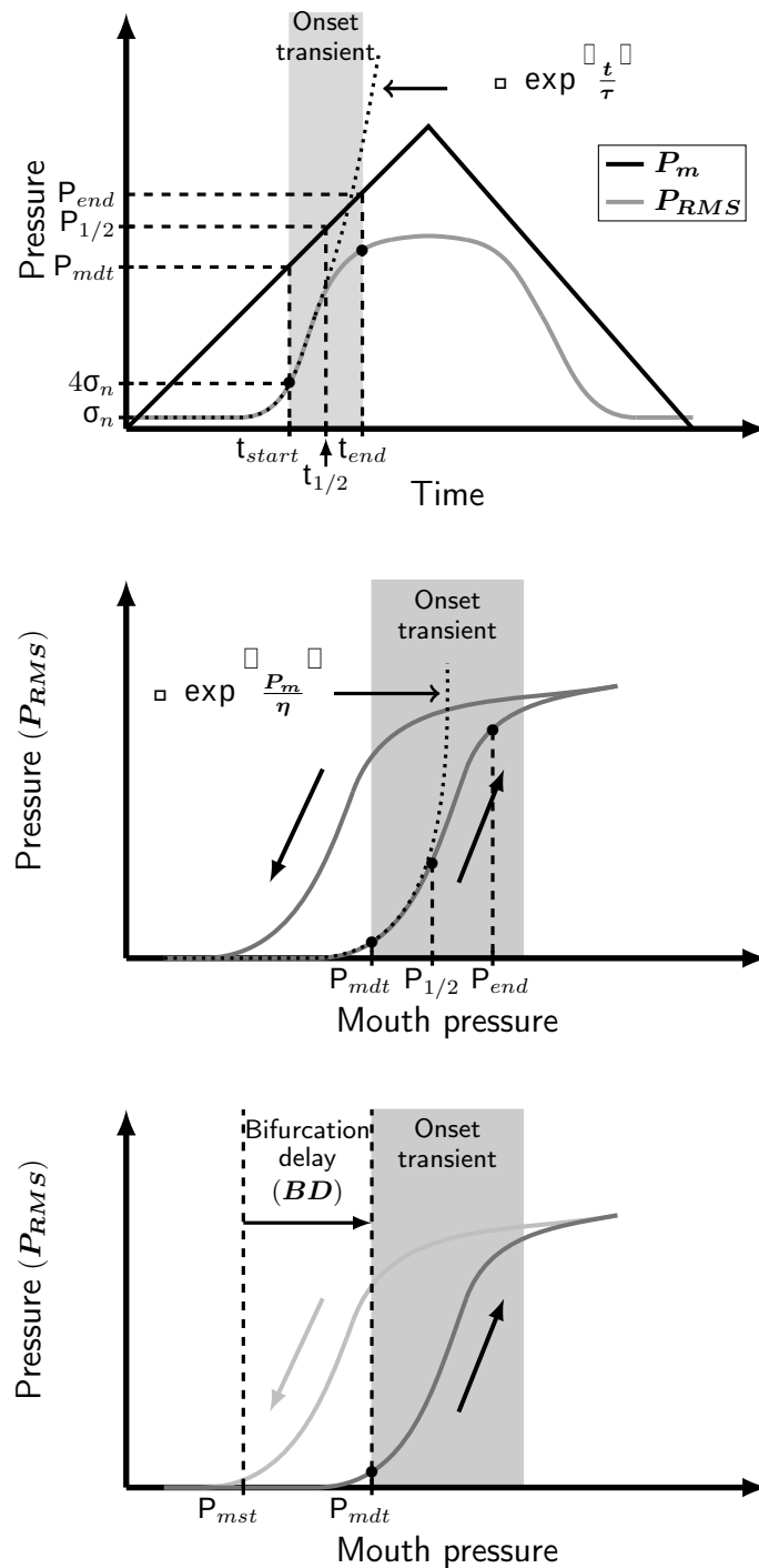
FIGURE 5.8 – Outline schematic showing the definition of the different indicators of the transient. At the top : blowing pressure P_m and of the RMS envelope P_{RMS} of the pressure inside the mouthpiece as functions of time. Illustrations of t_{start} , t_{end} , P_{mdt} , P_{end} and \tau . In the middle : P_{RMS} as a function of P_m . Illustration of \eta . At the bottom : illustration of the bifurcation delay (BD), corresponding to the pressure difference between the dynamic oscillation threshold P_{mdt} and the static oscillation threshold P_{mst} (see equation (5.16)).
