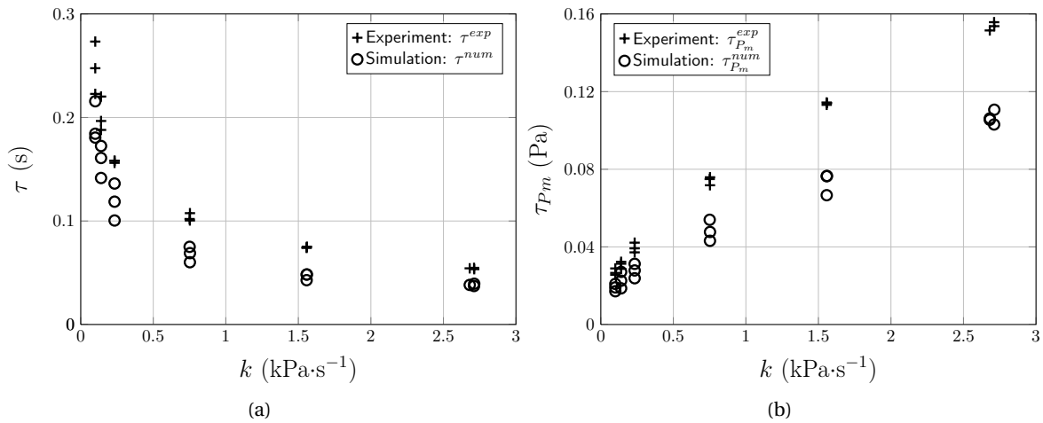
Figure 5.12 – Parameters \tau (a) and \tau P_m (b) as a function of the increase rate k of blowing pressure. (+) Experiment and (o) simulation.
