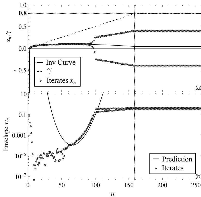
Figure 4.18 – Simulation and invariant curve and envelope predictions. Unlimited precision, \epsilon = .01 , \zeta = 1/2 , x_0 = 0.5 , \gamma_0 = 1/10 , \sigma = 10^{-4} .
