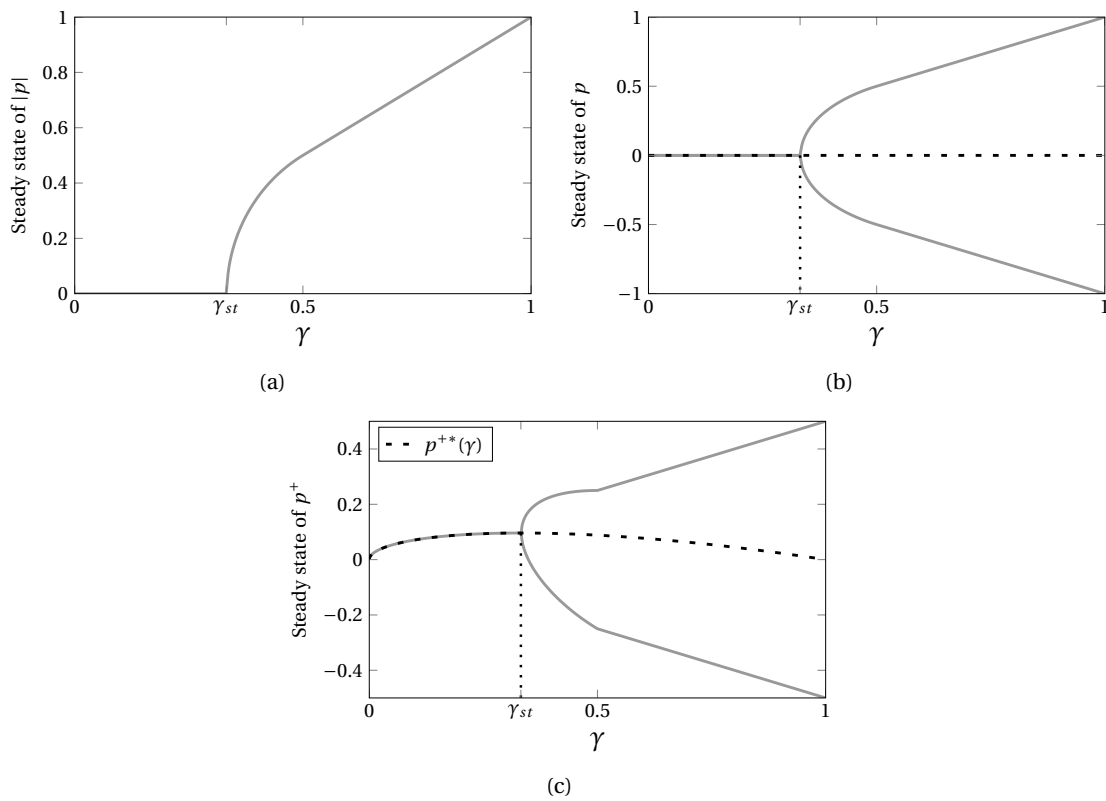
Figure 2.3 – Graphical representation of the static bifurcation diagrams for \zeta = 0.5 . Diagrams based on variables (a) |p| , (b) p and (c) p^+ . The dashed line represents the curve of the static regime, corresponding to the fixed point p^{+*}(\gamma) of the function G_\gamma when the diagram is base on variable p^+ .
