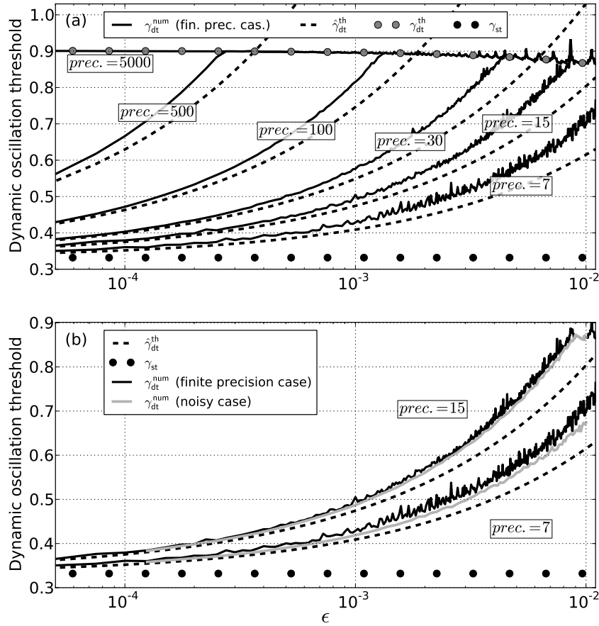
Figure 3.7 – Graphical representation of \gamma_{dt}^{num} for different precisions ( \text{prec.} = 7, 15, 30, 100, 500 and 5000 ) with respect to the slope \epsilon and for \gamma_0 = 0 . Results are also compared to analytical static and dynamic thresholds: \gamma_{st} , \gamma_{dt}^{th} and \hat{\gamma}_{dt}^{th} . (a) \gamma_{dt}^{num} and only finite precision cases are represented. (b) Both finite precision cases and noisy cases are represented for \text{prec.} = 7 and 15 .
