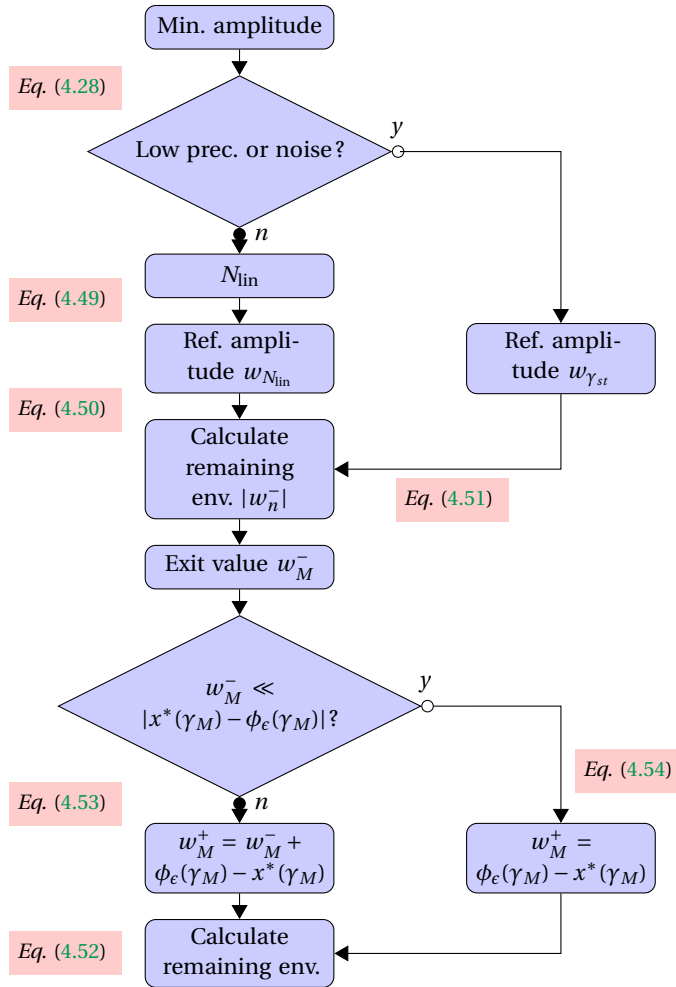
Figure 4.15 – Algorithm for determination of envelope
