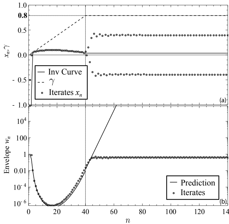
Figure 4.17 – Simulation and invariant curve and envelope predictions. Unlimited precision, \epsilon = .02 , \zeta = 1/2 , \gamma_M = 0.8 , x_0 = 0.5 , \gamma_0 = 1/100 .
