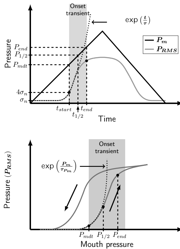
Figure 5.8 – Outline schematic showing the definition of the different indicators. At the top : schematic representation of the blowing pressure P_m and of the RMS envelope P_{RMS} of the pressure inside the mouthpiece as functions of time. Illustrations of t_{start} , t_{end} , P_{mdt} , P_{end} and \tau . At the bottom : schematic representation of P_{RMS} as a function of P_m . Illustration of \tau_{P_m} .
