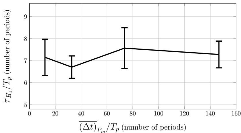
Figure 5.15 – Average plus or minus the standard deviation of the time growth constant \tau_{H_1} obtained for each value of (\Delta t)_{P_m} .
