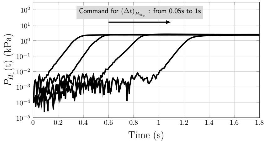
Figure 5.14 – Example of the time evolution P_{H_1}(t) for each value of (\Delta t)_{P_m} . A logarithmic scale is used for the ordinate axis.
