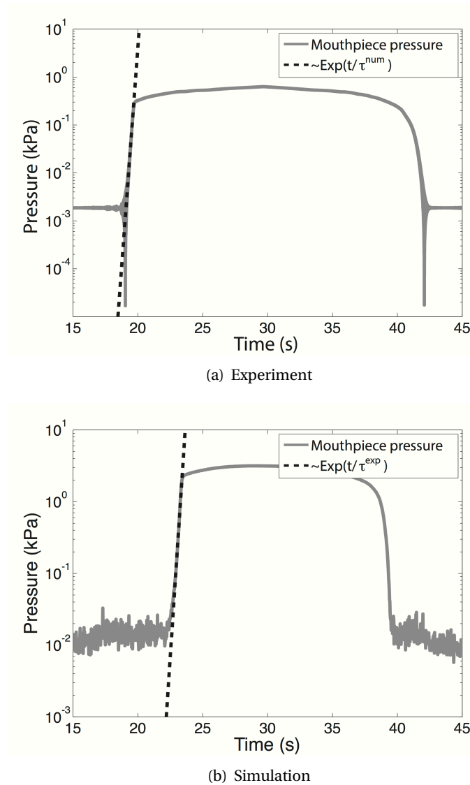
Figure 5.11 – Time profile of the RMS envelope P_{RMS}(t) (solid gray line) compared to its exponential fit during the onset transient (dashed black line). (a) Experimental signal and (b) simulated signal. k = 0.23\text{kPa/s} .
