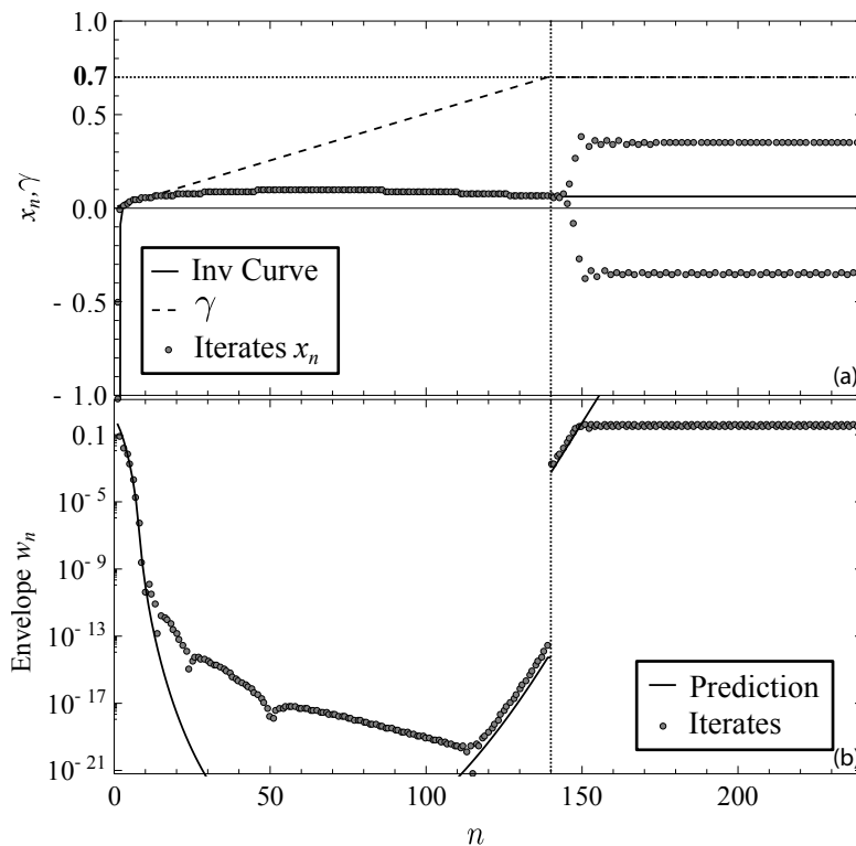
Figure 4.16 – Simulation and invariant curve and envelope predictions. Unlimited precision, \epsilon = 0.005 , \zeta = 1/2 , \gamma_M = 0.7 , \gamma_0 = 1/100 , x_0 = 0.5 .
