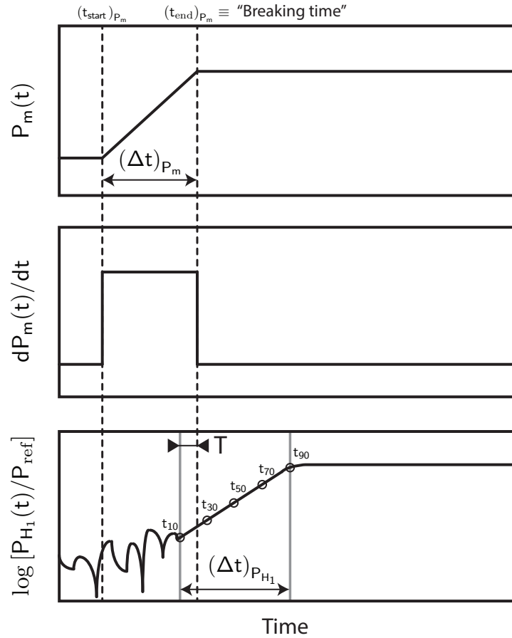
Figure 5.13 – Schematic representation of (a) the blowing pressure P_m and (b) its first time derivative. Dashed lines demarcate the duration (\Delta t)_{P_m} of the transient of P_m . (c) Schematic representation of \log[P_{H_1}(t)] . Gray lines depict the duration (\Delta t)_{P_{H_1}} of the onset transient of the pressure P inside the mouthpiece. The duration T , defined by equation (5.21), is also represented.
