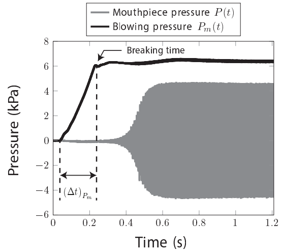
Figure 5.5 – Measured signals : the blowing pressure P_m(t) (solid black line) and the pressure inside the mouthpiece P(t) (solid gray line).
