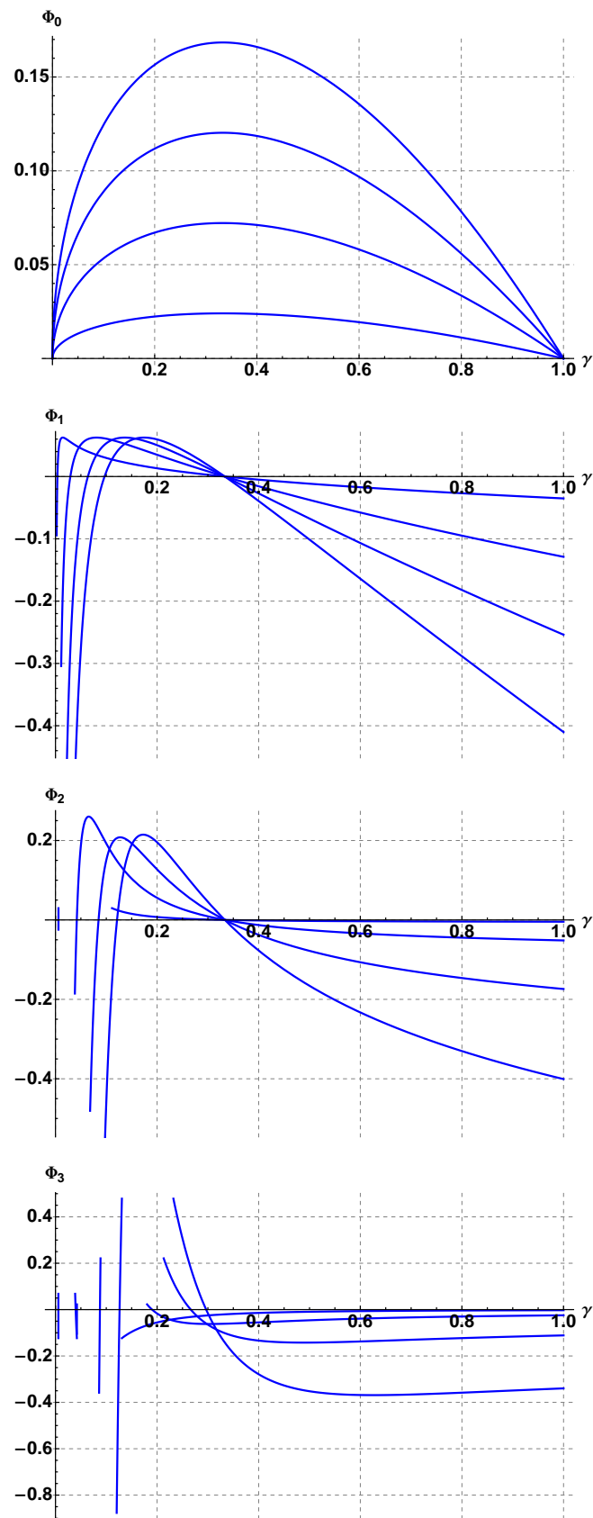
Figure 4.19 – First four terms of the perturbation approximation to the invariant curve, each plotted as a function of \gamma for four different values of \zeta ( 1/8 , 3/8 , 5/8 and 7/8 ).
