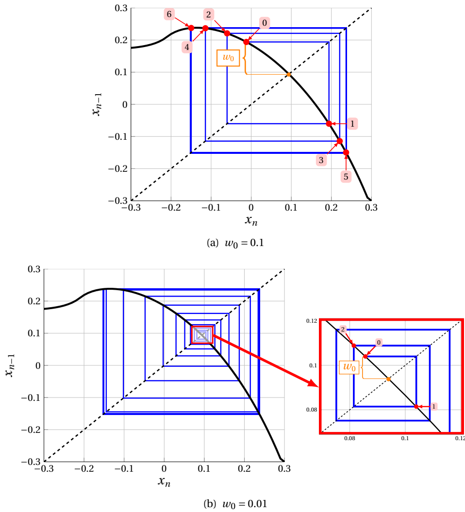
Figure 4.5 – Graphical solution of equation (4.9) for \gamma = 0.42 and \zeta = 0.5 . (—) Path of the successive iterates 0, 1, 2, etc ; (—) iterative function G and (- - -) identity y = x . (a) w_0 = 0.1 and (b) w_0 = 0.01 .
