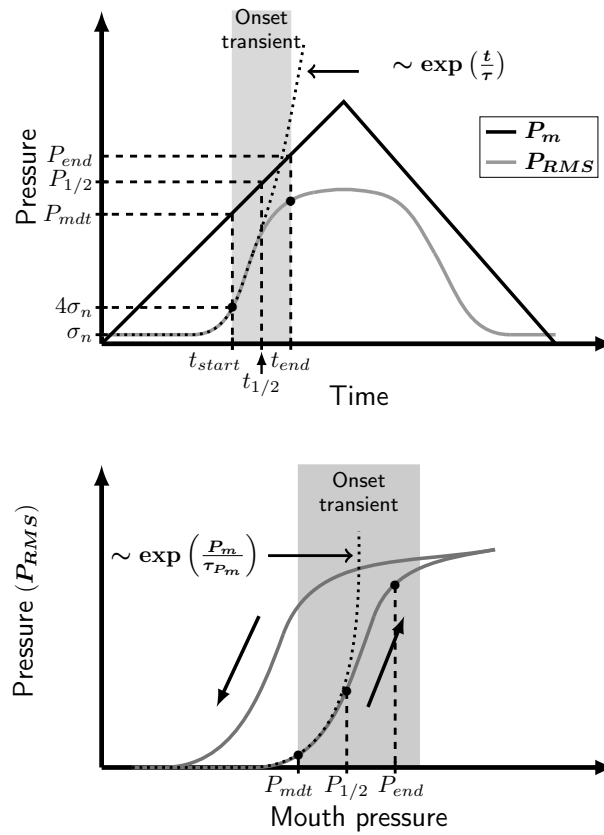
Figure 5.8 – Outline schematic showing the definition of the different indicators. At the top : schematic representation of the blowing pressure P_m and of the RMS envelope P_{RMS} of the pressure inside the mouthpiece as functions of time. Illustrations of t_{start} , t_{end} , P_{mdt} , P_{end} and \tau . At the bottom : schematic representation of P_{RMS} as a function of P_m . Illustration of \tau_{P_m} .
