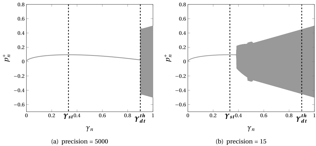
Figure 2.8 – Representation of the series p_n^+ for \zeta = 0.5 , \epsilon = 10^{-4} , \gamma_0 = 0 , p_0^+ = G(0, \gamma_0) and for two different values of the precision.
