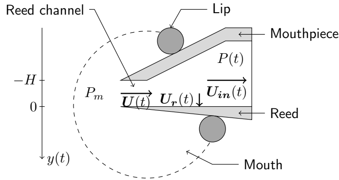
Figure 5.6 – View of the physical quantities used in the model.
