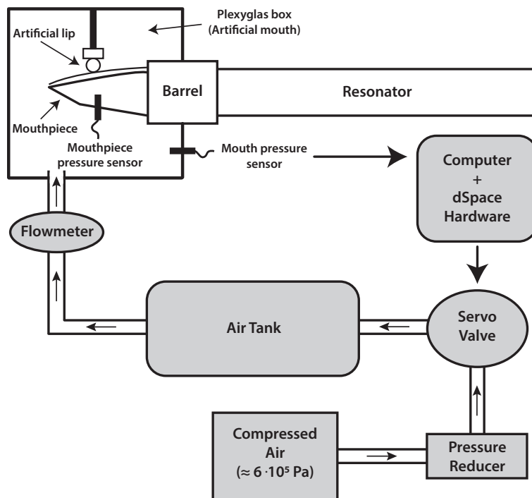
Figure 5.3 – Principle of the pressure controlled artificial mouth.
