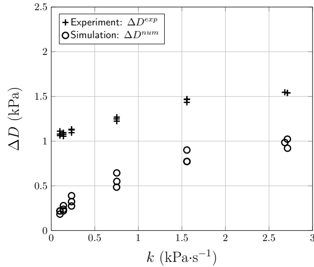
Figure 5.10 – Bifurcation delay estimated on experimental signals ( \Delta D^{exp} (+)) and on simulated signals ( \Delta D^{num} (o)) as functions of the slope k .
