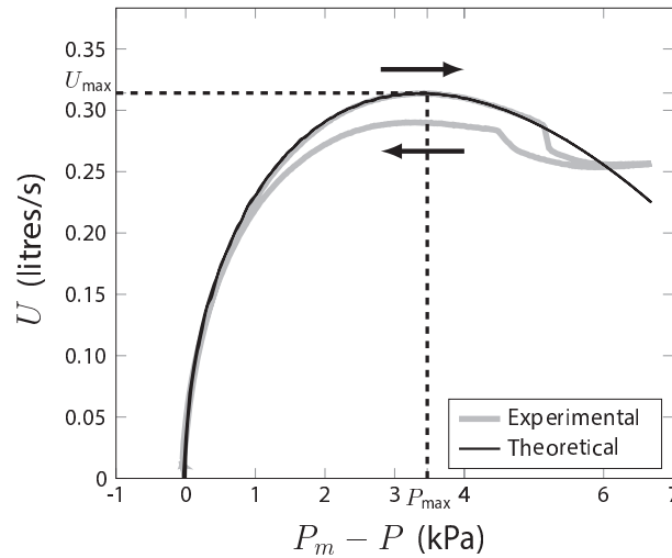
Figure 5.7 – Experimental nonlinear exciter characteristics (gray line) for increasing and decreasing blowing pressure and comparison with model (black line) for increasing blowing pressure. In this example the increase rate k of the blowing pressure is equal to 0.1kPa/s.
