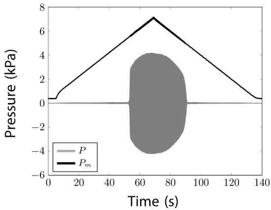
Figure 5.4 – Time evolution of the mouth pressure P_m , the pressure inside the mouthpiece P . The slope k of the mouth pressure is equal to 0.1 kPa/s.
