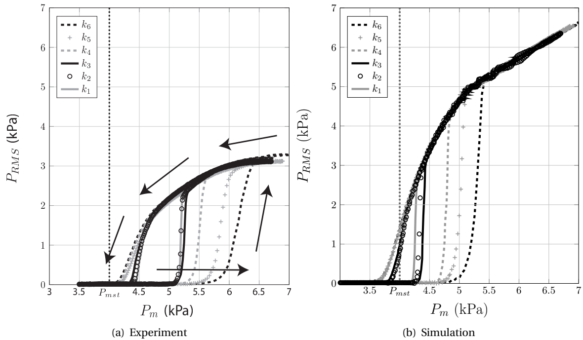
Figure 5.9 – P_{RMS} as a function of P_m for each value of the slope k . (a) Experimental signals, (b) signals generated by the numerical simulation of the model with parameters \zeta and P_M estimated experimentally (cf. section 5.2.4.1) as well as the measured blowing pressure signal P_m(t) . Arrows represent the direction of the mouth pressure time evolution and highlight an hysteresis cycle.
