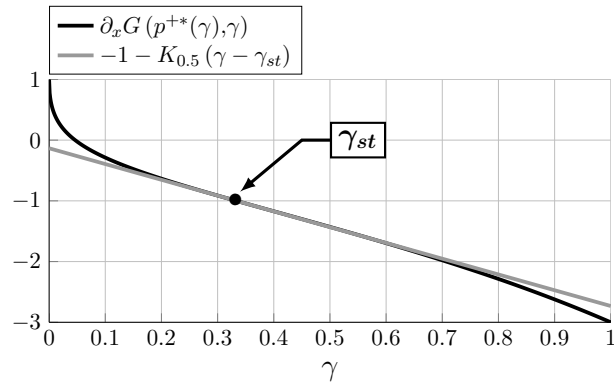
(b) \zeta = 0.5
