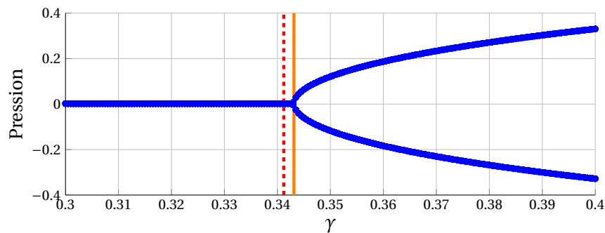
(c) \lambda = 0.98
