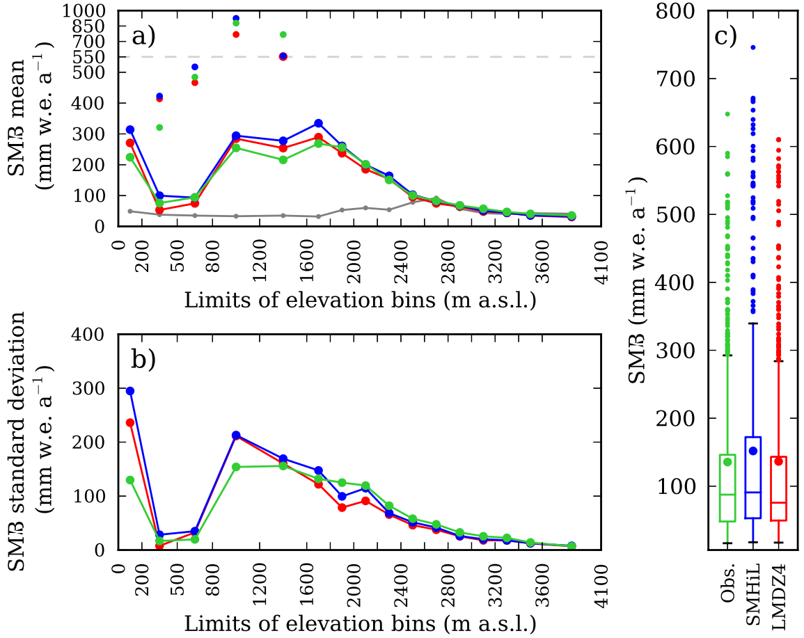
FIGURE 4.3 – Statistical analysis of observed and modeled SMB. Field data, displayed in green, are first averaged on the SMHiL grid cell in which they are included. LMDZ4, displayed in red, is interpolated on the SMHiL grid before averaging. SMHiL is in blue. a) Mean and b) standard deviation of SMB computed by elevation bins. Limits of elevations bins are displayed on the horizontal axis. The number of observations by bins (after average on SMHiL grid cells) is displayed in light grey on figure a). We separated SMB values from 200 m to 1600 m (a.s.l.) into two groups because very low SMB values measured in Ross ice shelf area where statistically distinct from high SMB values elsewhere (i.e. mainly in Adélie Land). c) Boxplot statistics of SMB values above 200m a.s.l. The box extends from the lower (Q1) to upper quartile (Q3) values of the data, with a line at the median. The whiskers extend from the box to the most extreme data point within 1.5(Q3-Q1) data range. They are close to the extreme range of a normally distributed population of same interquartile. Flier points (small dots) are values that past the end of the whiskers. Big dots are mean SMB.
