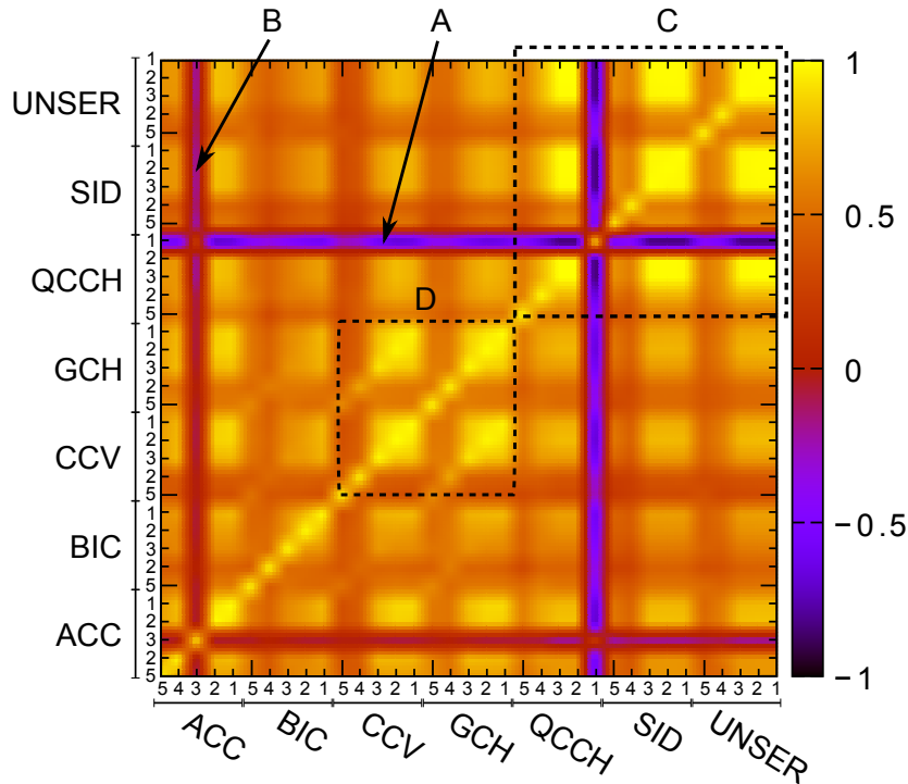
Figure 5.7: Complete correlation coefficients for each descriptors at the segmentation scales \lambda_1, \dots, \lambda_5 .
