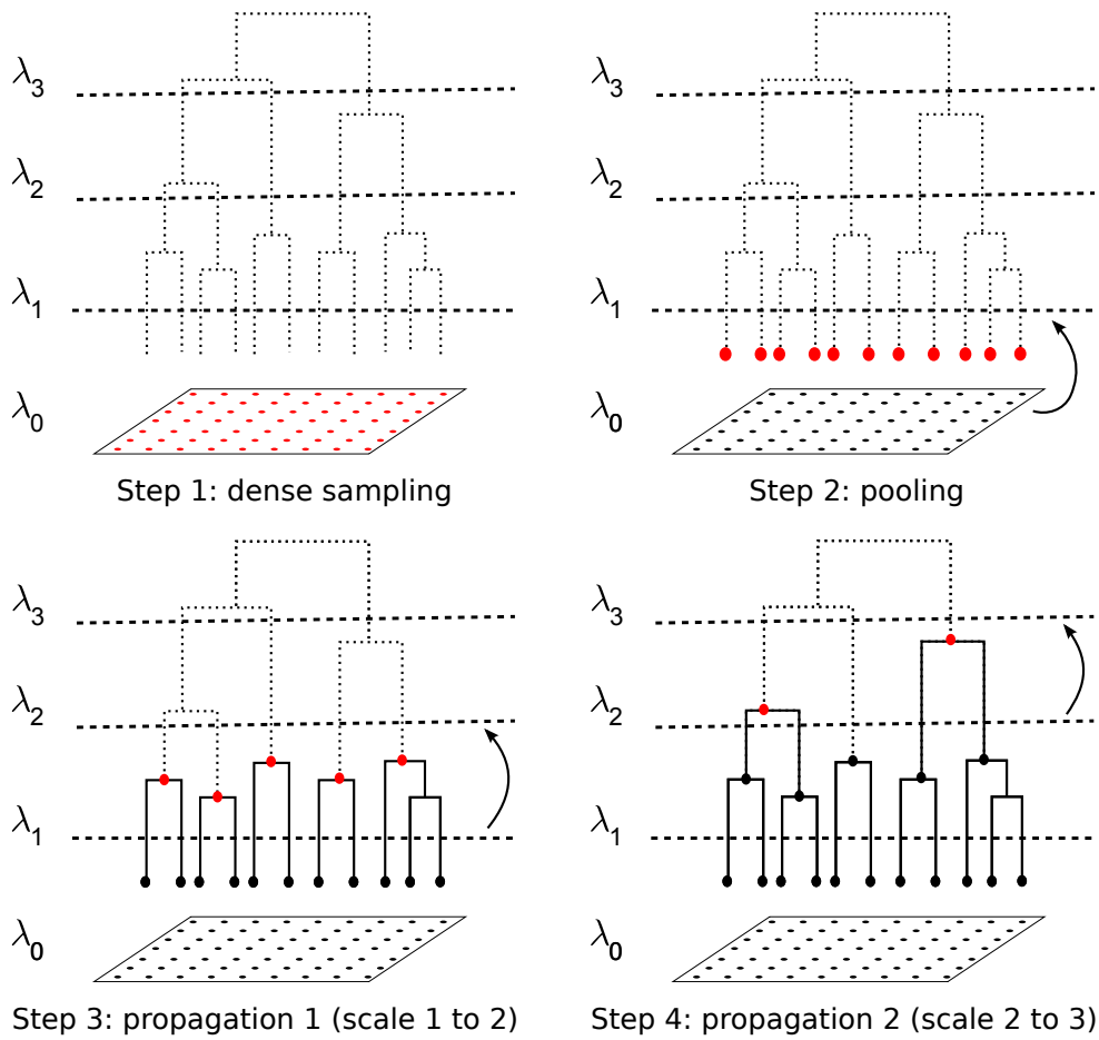
Figure 7.2: The BoW-propagation main steps. The process starts with the dense sampling in the pixel level (scale \lambda_0 ). Low-level features are extracted from each interest point. Then, in the second step, a feature histogram is created for each region R \in P_{\lambda_1} by pooling the features from the internal interest points. In the third step, the features are propagated from scale \lambda_1 to scale \lambda_2 . In the fourth step, the features are propagated from scale \lambda_2 to the coarsest considered scale ( \lambda_3 ). To obtain the feature histograms of a given scale, the propagation is performed by considering the histograms of the previous scale.
