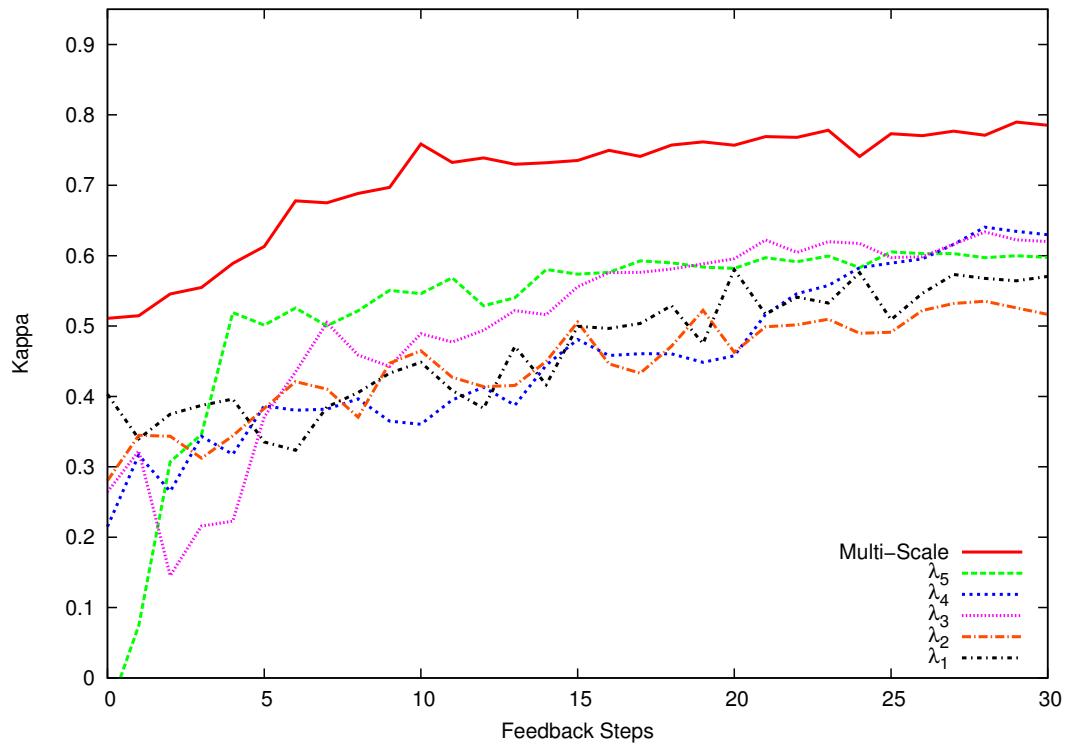
Figure 6.6: Kappa index for each iteration of feedback for the COFFEE dataset considering five scales and the multiscale classification approach.
