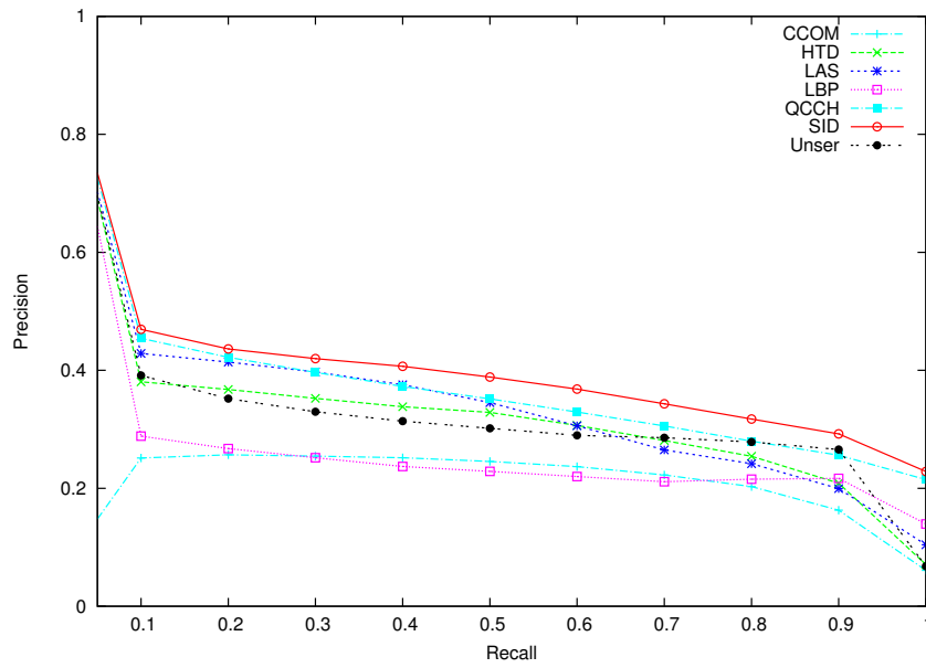
Figure 4.3: Precision \times Recall curves for texture descriptors, considering the PASTURE dataset.
