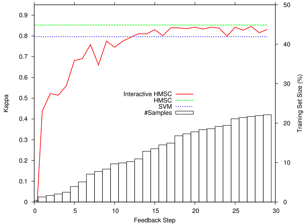
Figure 6.12: Kappa index for the HMSC and SVM and Kappa \times Feedback Steps curves for interactive HMSC using the URBAN dataset. The histogram represents the percentage of the training set used in the interactive method.
