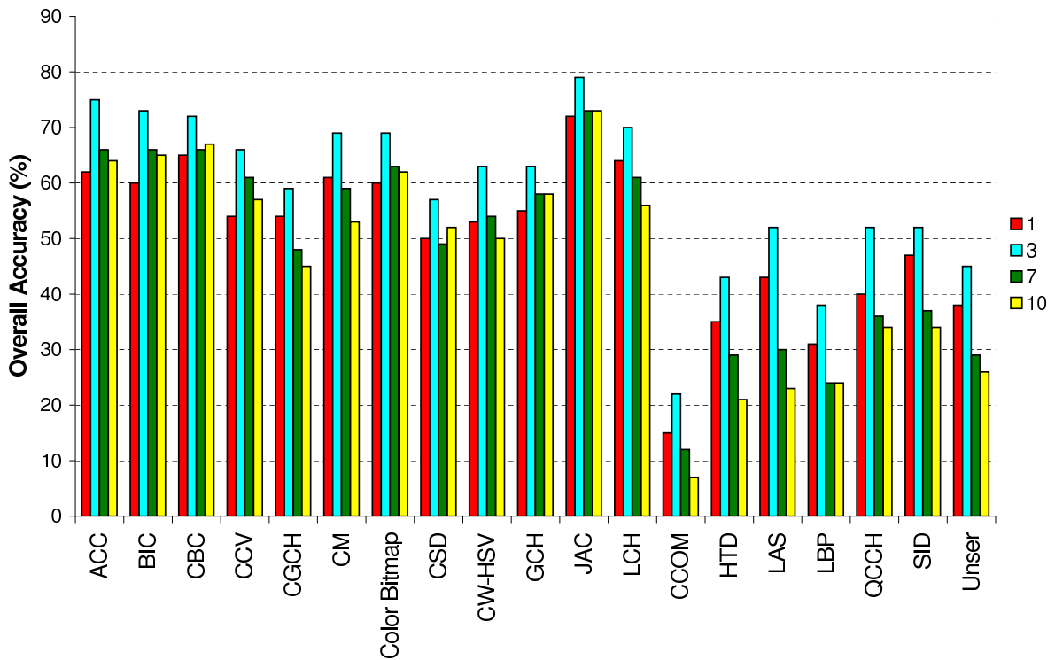
Figure 4.5: Overall accuracy classification of each descriptor for the COFFEE dataset, using KNN with k equal to 1, 3, 7 and 10.
