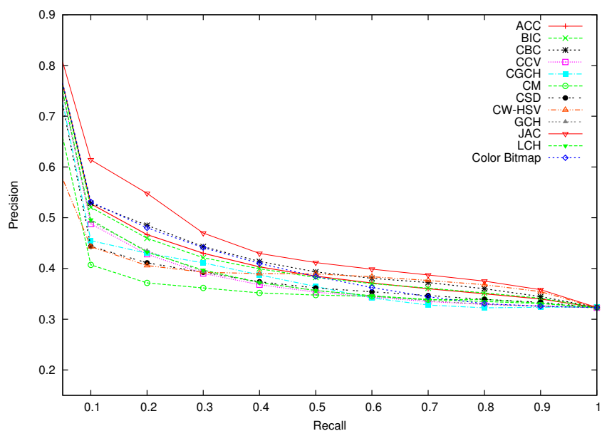
Figure 4.2: Precision \times Recall curves for color descriptors, considering the PASTURE dataset.
