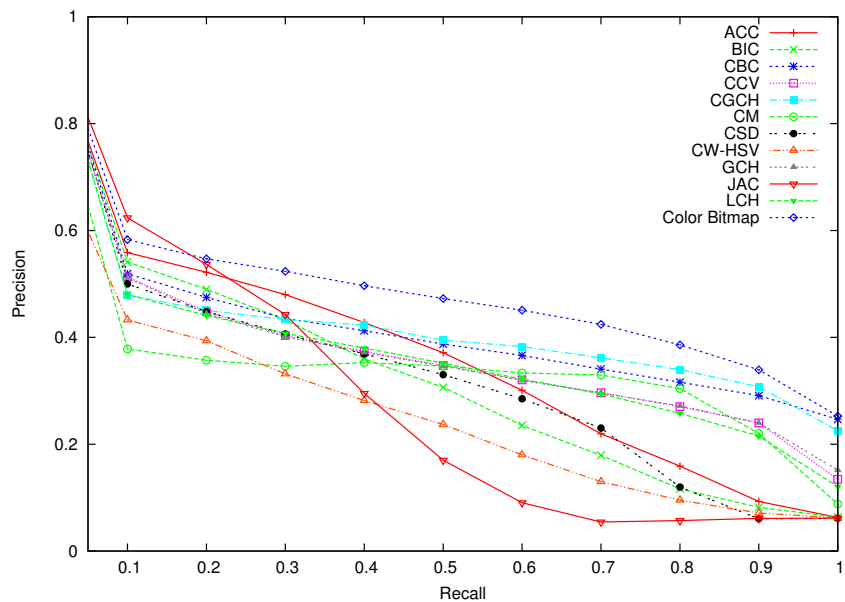
Figure 4.1: Precision \times Recall curves for color descriptors, considering the PASTURE dataset.
