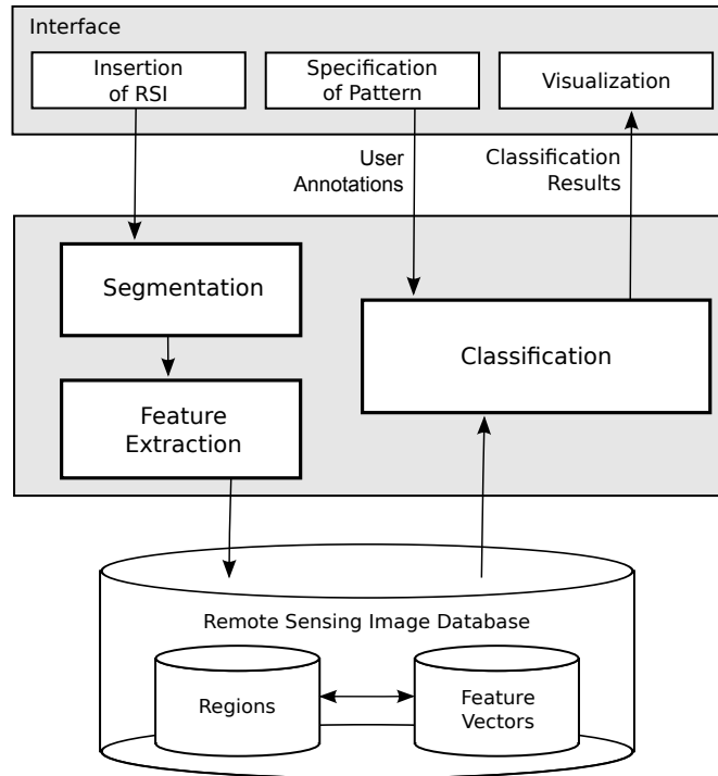
Figure 6.1: Architecture of the interactive classification system.
