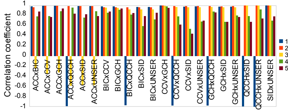
Figure 5.8: Correlation of pairs of classifiers for different segmentation scales.
