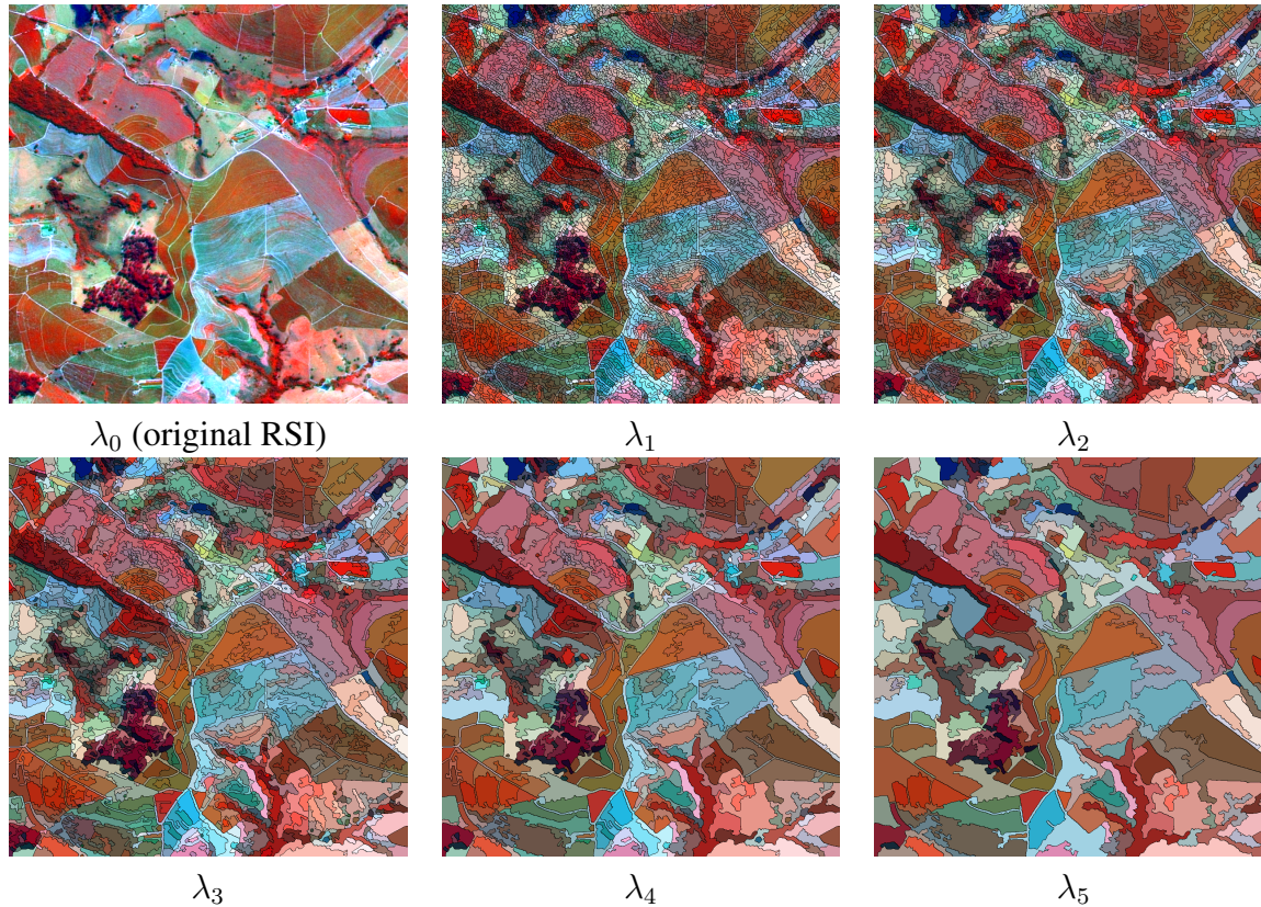
Figure 3.3: One of the tested subimages and the results of segmentation in each of the selected scales for the COFFEE dataset.
