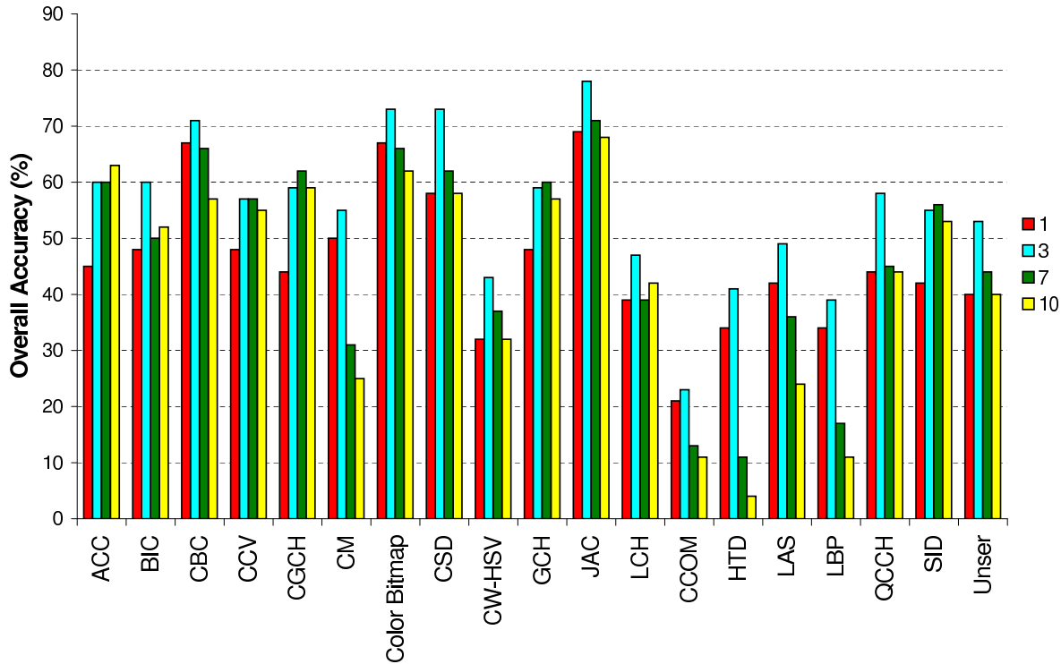
Figure 4.6: Overall accuracy classification of each descriptor for the PASTURE dataset, using KNN with k equal to 1, 3, 7 and 10.
