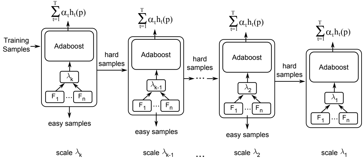
Figure 5.2: The hierarchical multiscale training strategy.
