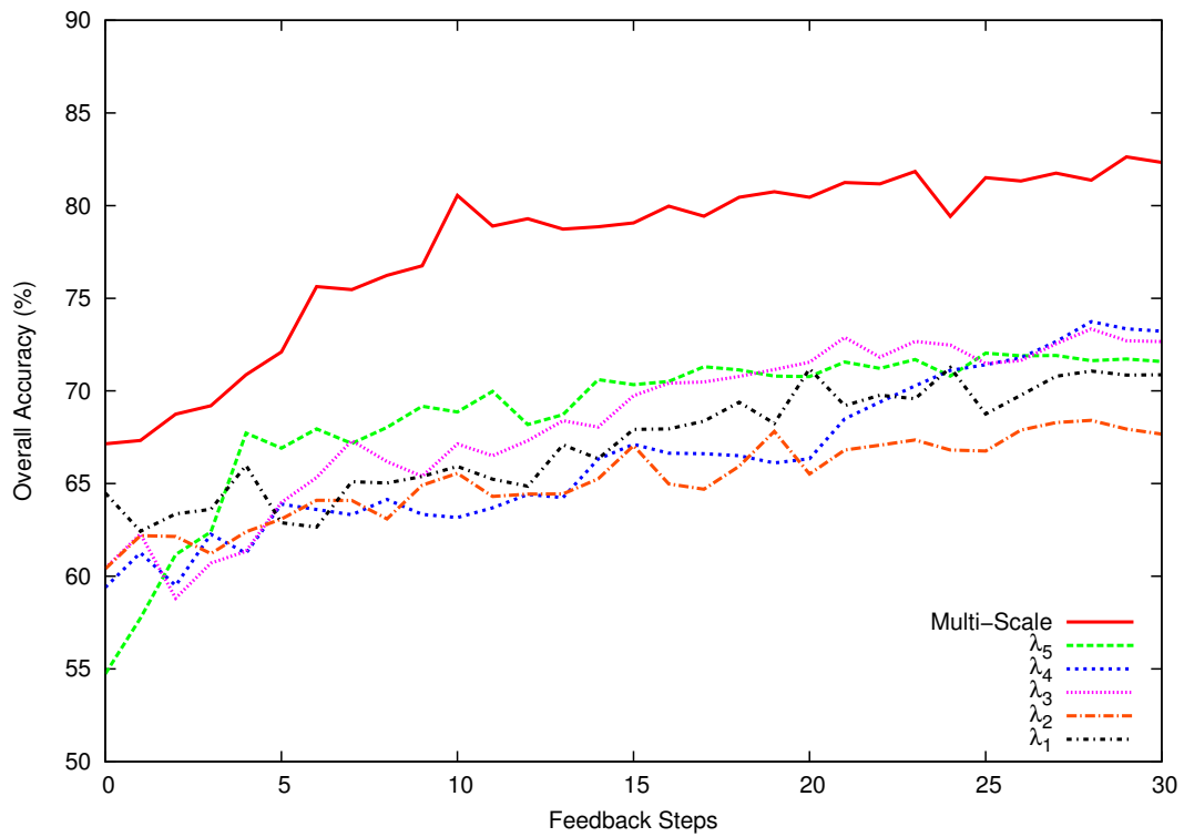
Figure 6.7: Overall accuracy for each iteration of feedback for the COFFEE dataset, considering five scales and the multiscale classification approach.
