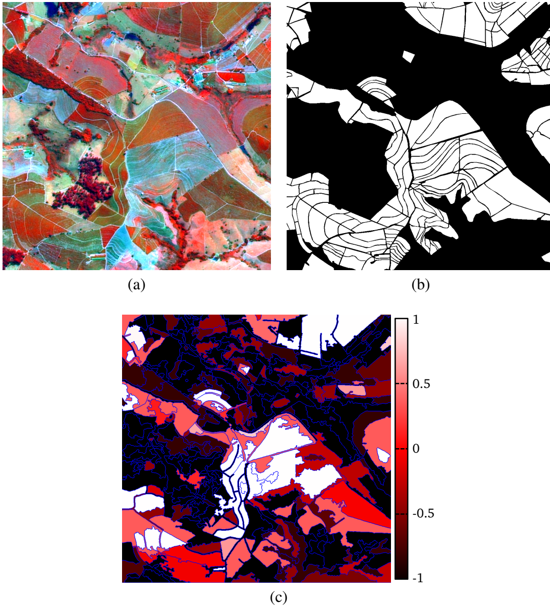
Figure 6.2: Example of classification with different degrees of doubt: (a) original image, (b) ground truth and, (c) regions with different classification levels. In (b) and (c), white and black regions are coffee and non-coffee crops, respectively. The redder the region, the closer to the decision function.
