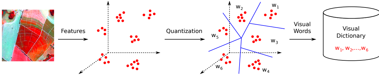
Figure 2.4: Construction of a visual dictionary to describe a remote sensing image. The features are extracted from groups of pixels (e.g., tiles or segmented regions), the feature space is quantized so that each cluster corresponds to a visual word w_i .
