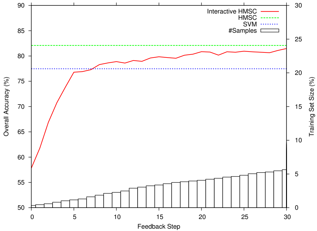
Figure 6.11: Overall Accuracy results for the HMSC and SVM and Overall Accuracy \times Feedback Steps curves for interactive HMSC using the COFFEE dataset. The histogram represents the percentage of the training set used in the interactive method.
