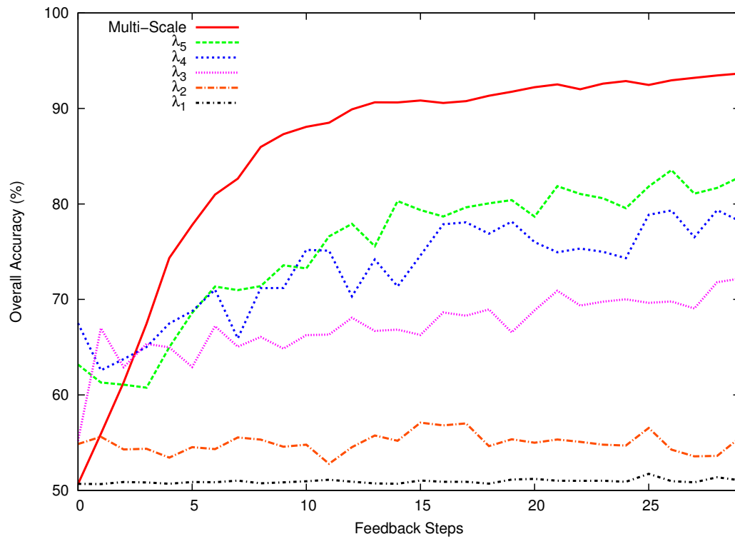
Figure 6.9: Overall accuracy for each iteration of feedback for URBAN dataset, considering five scales and the multiscale classification approach.
