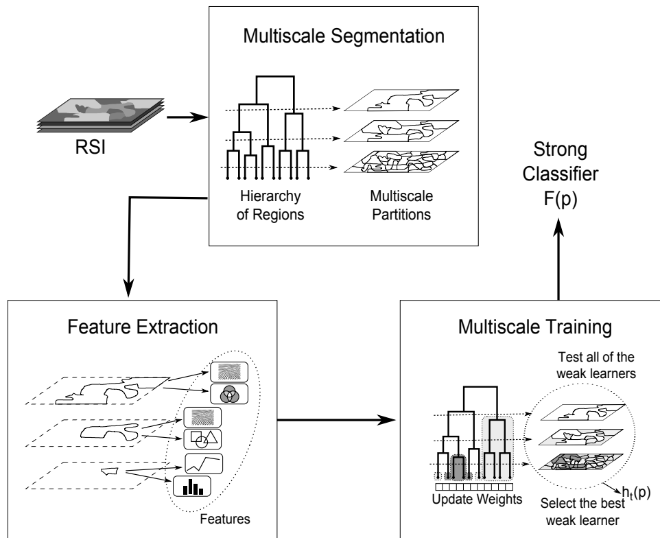
Figure 5.1: Steps of the multiscale training approach. At the beginning, several partitions P_\lambda of hierarchy H at various scales \lambda are selected. Then, at each scale \lambda , a set of features is computed for each region R \in P_\lambda . Finally, a classifier F(p) is built by using the Multiscale Training (Section 5.2.2) or the Hierarchical Multiscale Training (Section 5.2.3).
