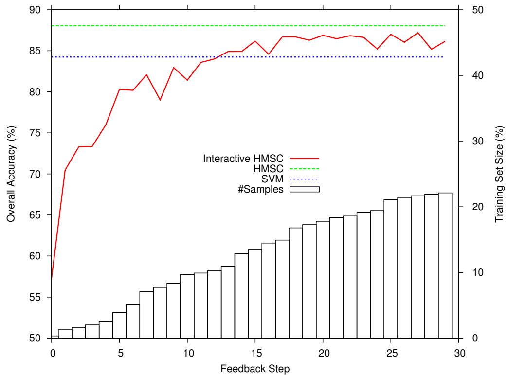
Figure 6.13: Overall Accuracy results for the HMSC and SVM and Overall Accuracy \times Feedback Steps curves for interactive HMSC using the URBAN dataset. The histogram represents the percentage of the training set used in the interactive method.
