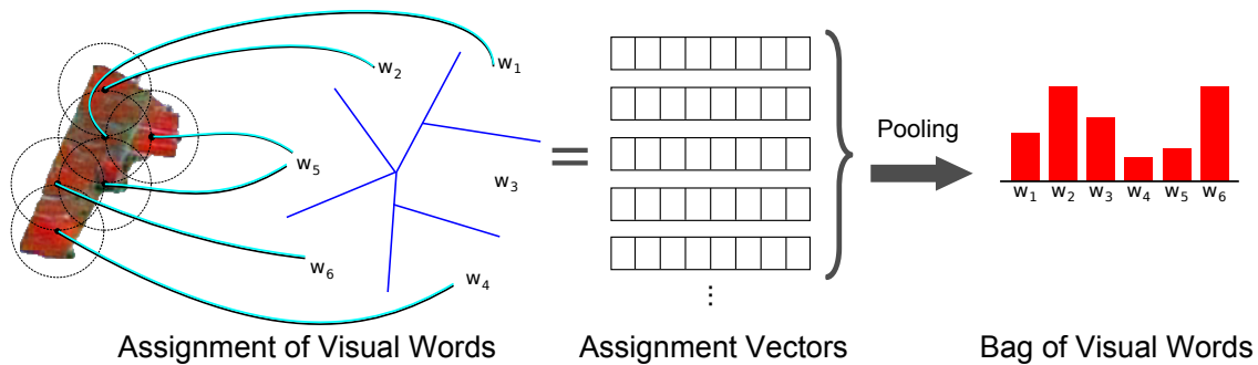
Figure 7.4: Schema to represent a segmented region based on a visual dictionary with dense sampling feature extraction.
