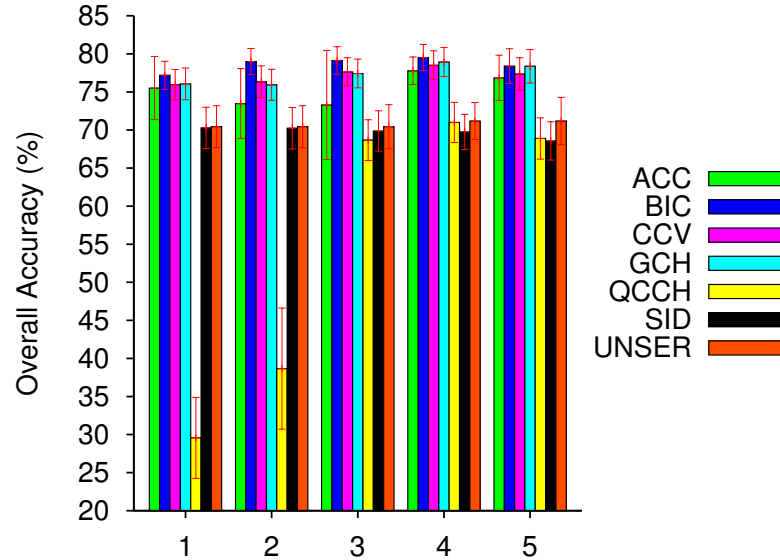
Figure 5.5: Overall accuracy for each descriptor at segmentation scales \lambda_1, \dots, \lambda_5 .
