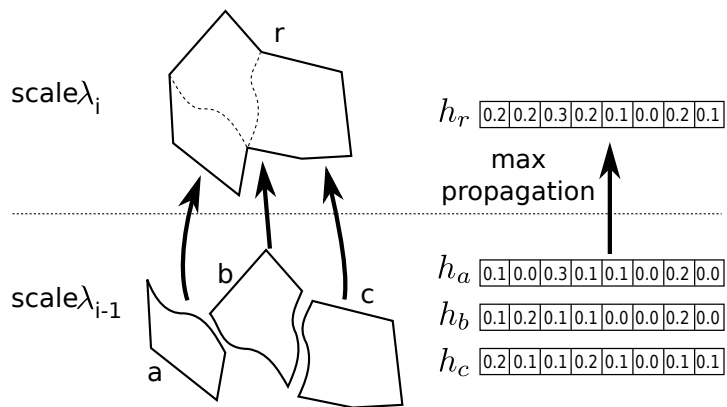
Figure 7.6: Feature propagation example using a max pooling operation.
