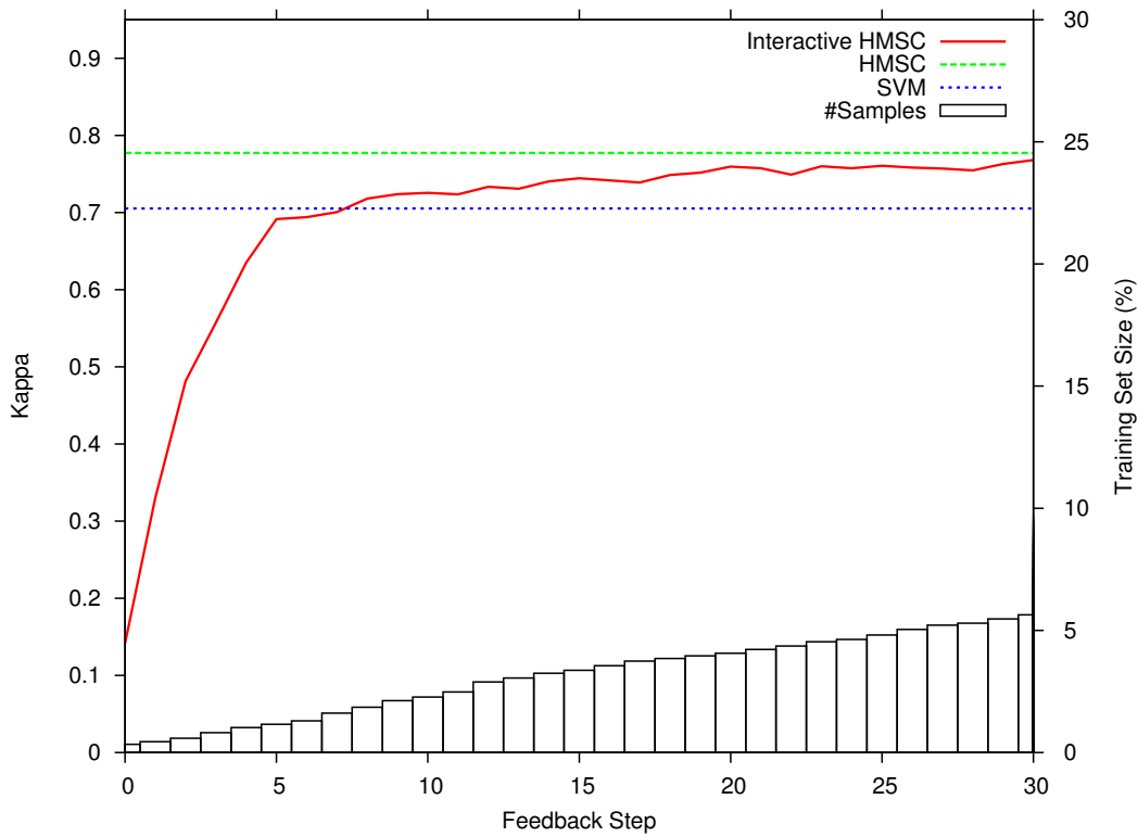
Figure 6.10: Kappa index for the HMSC and SVM and \text{Kappa} \times \text{Feedback Steps} curves for interactive HMSC using the COFFEE dataset. The histogram represents the percentage of the training set used in the interactive method.
