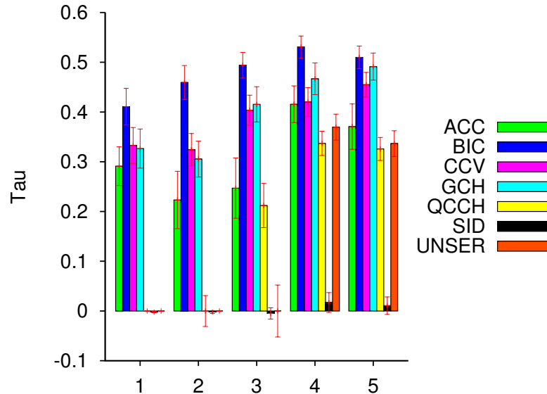
Figure 5.6: Tau index for each descriptor at segmentation scales \lambda_1, \dots, \lambda_5 .
