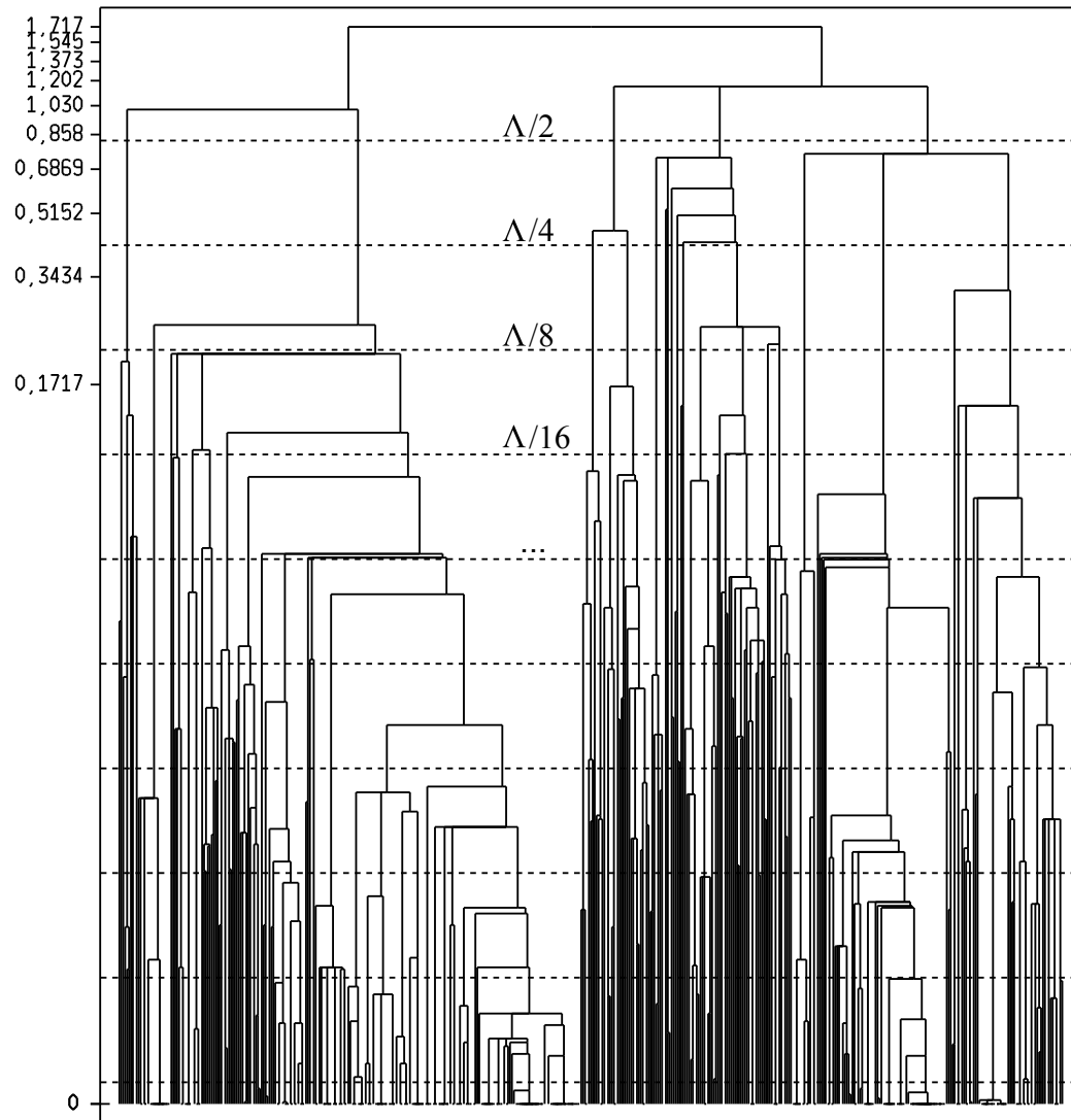
Figure 2.1: A scale-sets image representation. Horizontal axis: the regions. Vertical axis: the scales (logarithmic representation).
