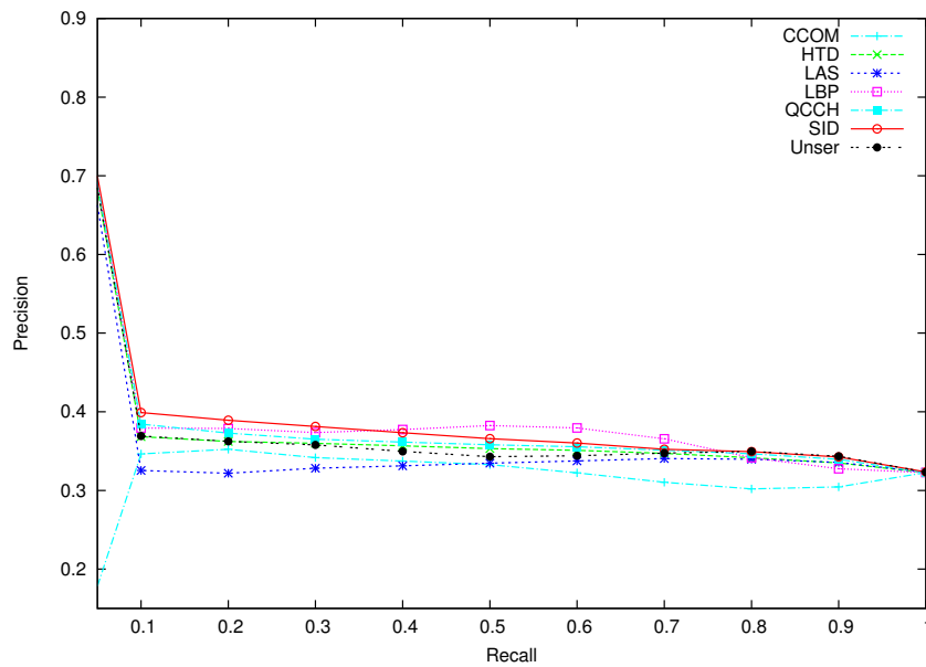
Figure 4.4: Precision \times Recall curves for texture descriptors, considering the PASTURE dataset.
