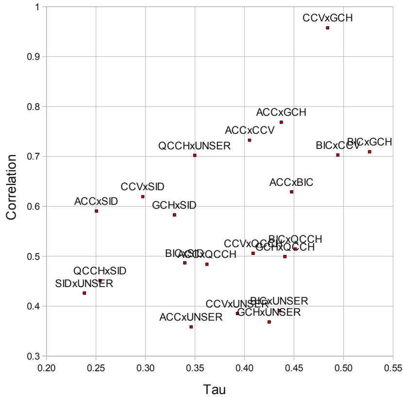
Figure 5.9: Distribution of pairs of classifiers considering the \lambda_5 scale for one of the validation sets.
