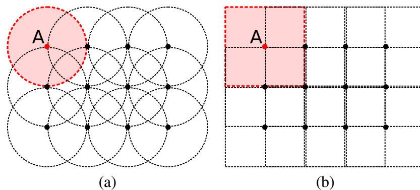
Figure 2.3: Dense sampling using (a) circles and (b) square windows. The highlighted area indicates the region from which the features corresponding to point A are extracted.
