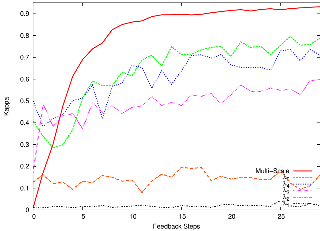
Figure 6.8: Kappa index for each iteration of feedback for the URBAN dataset, considering five scales and the multiscale classification approach.
