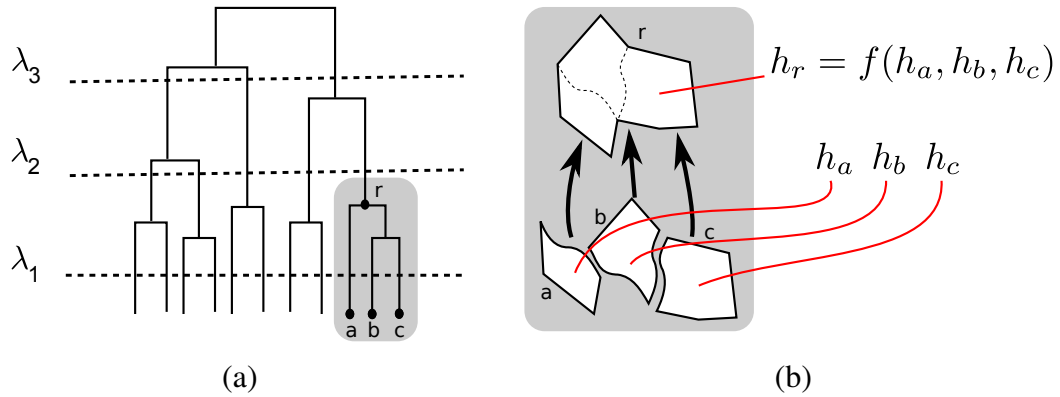
Figure 7.5: Computing the bag h_r of region r by combining the features h_a , h_b , and h_c from the subregions a , b , and c .
