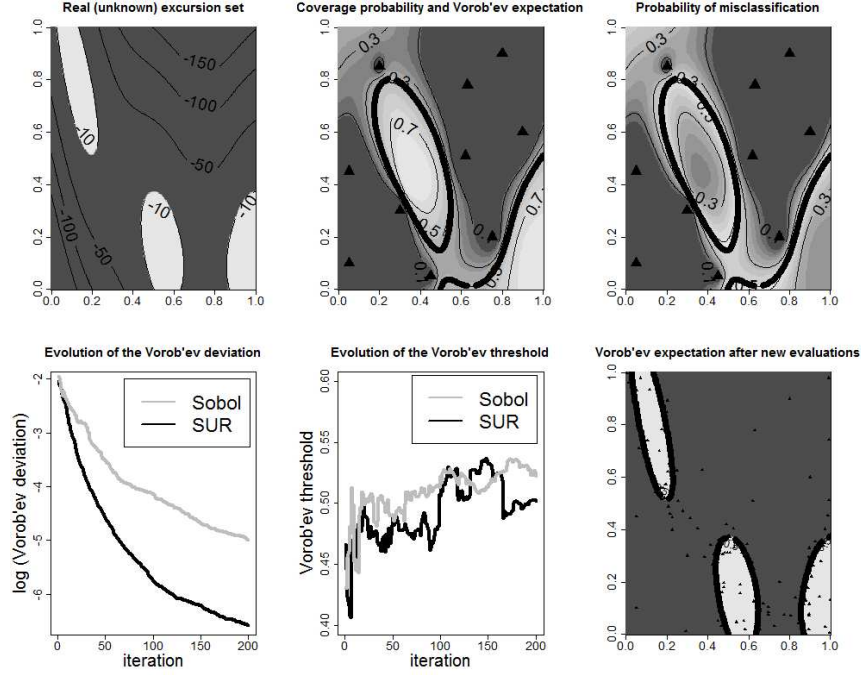
Fig. 2: Top left: Level set of a 2d function. Middle: Coverage probability function after 10 evaluations of f . Top right: \mathbb{E}(\mathbb{1}_{Q_{n,\alpha_n^*}\Delta\Gamma}(\cdot)) function. Bottom left: Decrease of the Vorob'ev deviation when new points are added (2 strategies). Middle: Evolution of \alpha^* . Bottom right: New Vorob'ev expectation (SUR strategy).
