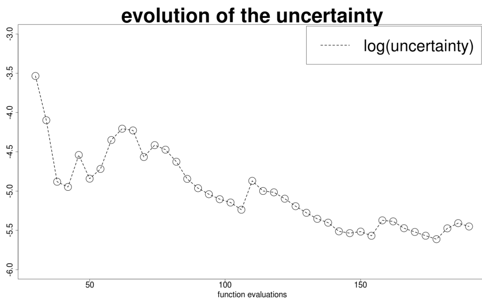
Figure 6.2: Evolution of the uncertainty \hat{H}_n during the sequential sampling strategy.
