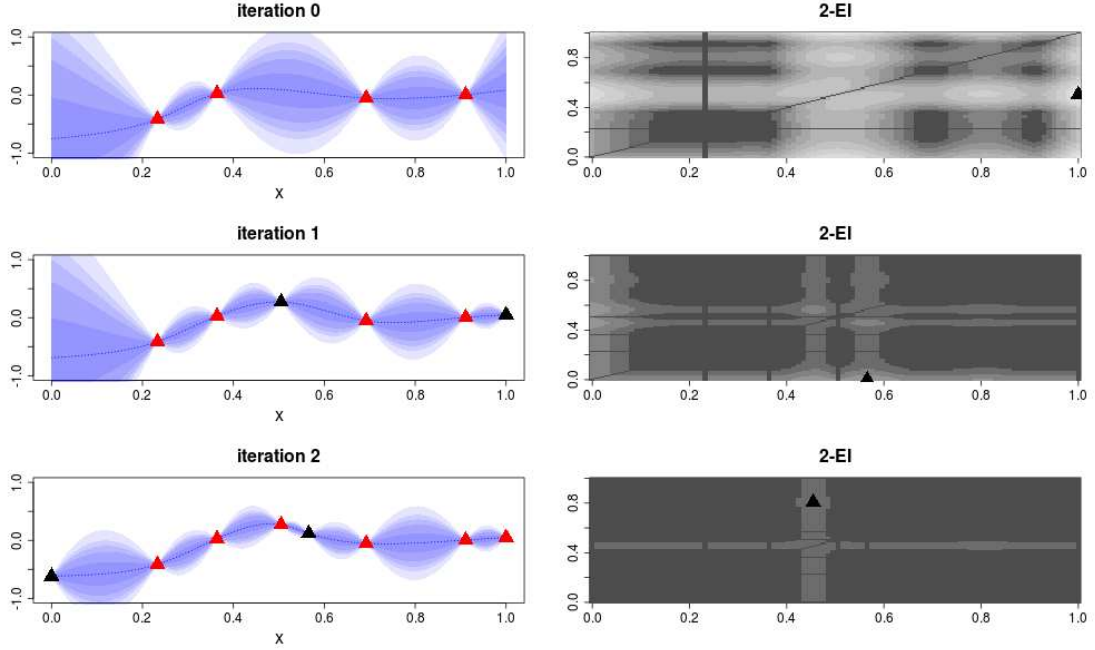
Figure 2.2: 2 iterations of a batch-sequential optimization strategy using the q-EI, for q = 2 , on a 1d-function. Left: kriging mean (blue dotted line) and confidence intervals. Right: function q-EI( \mathbf{x}^{(2)} ) where \mathbf{x}^{(2)} is a batch of two points. At each iteration, the batch evaluated is the black triangle on the right plots.
