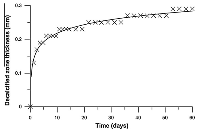
Fig. 9. Modelled decalcified zone thickness vs. time.
