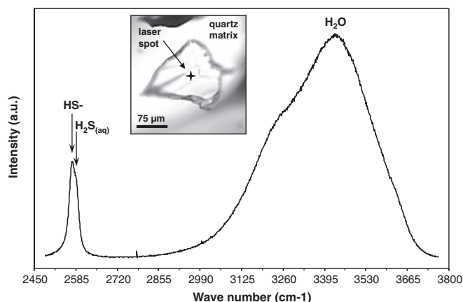
Fig. 4. Raman spectrum of the brine trapped in the synthetic fluid inclusions showing the presence of HS - and H 2 S (aq) species and the predominance of the former. Insert: micro-thermometric observation of fluid inclusion at the experimental temperature.
