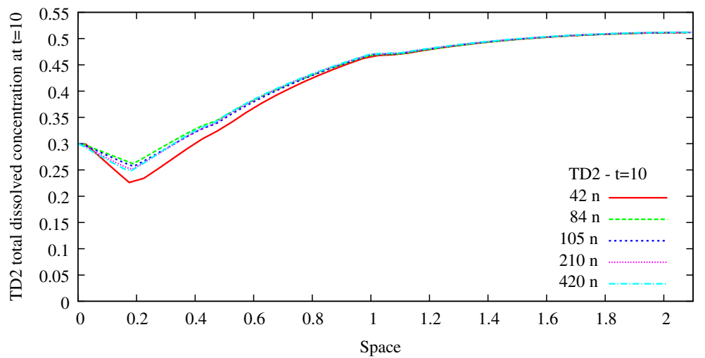
Fig. 11 Concentration profile for the dispersive easy 1D case of the total dissolved TD2 at t = 10
