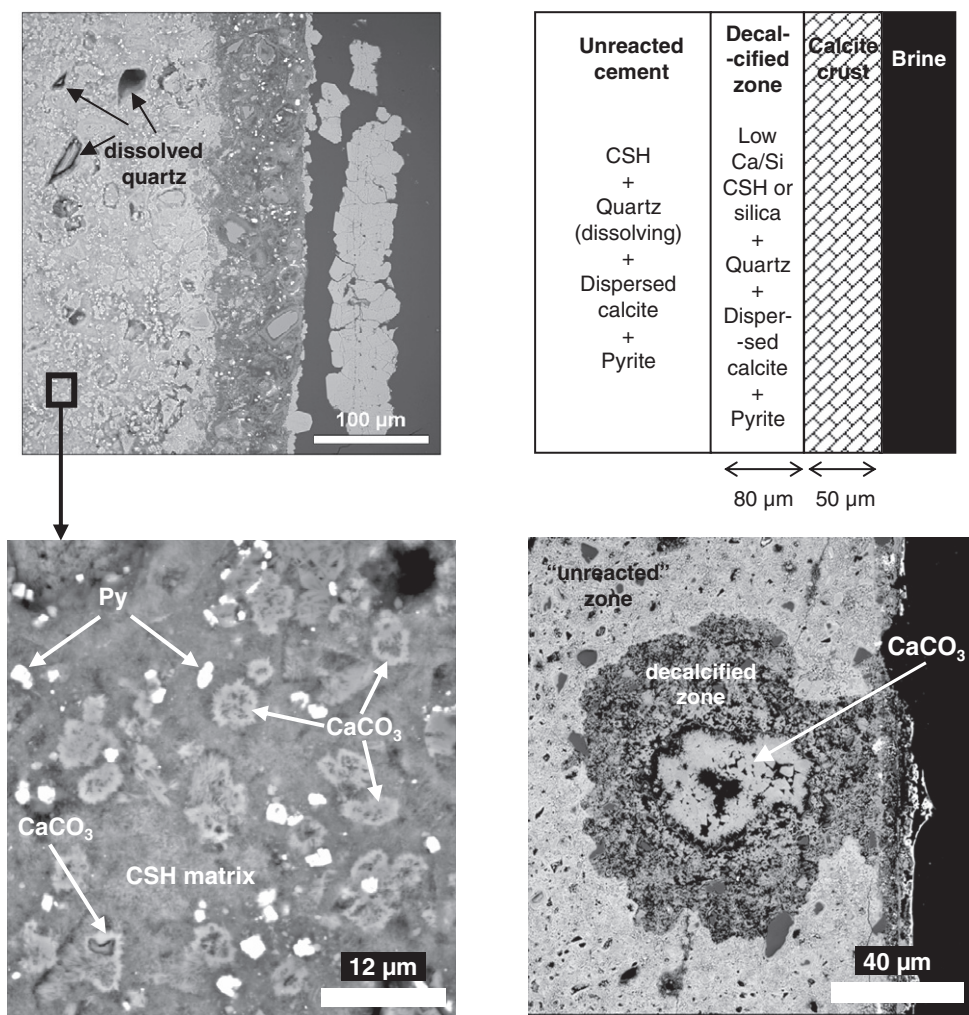
Fig. A1. SEM observation of cement altered at 200 °C (top left) and corresponding mineralogical profile (top right); CaCO 3 micro-crystals within the CSH matrix of cement altered at 200 °C (bottom left); void filled with CaCO 3 euhedral crystals surrounded by decalcified zone (bottom right) within the cement altered at 200 °C.
