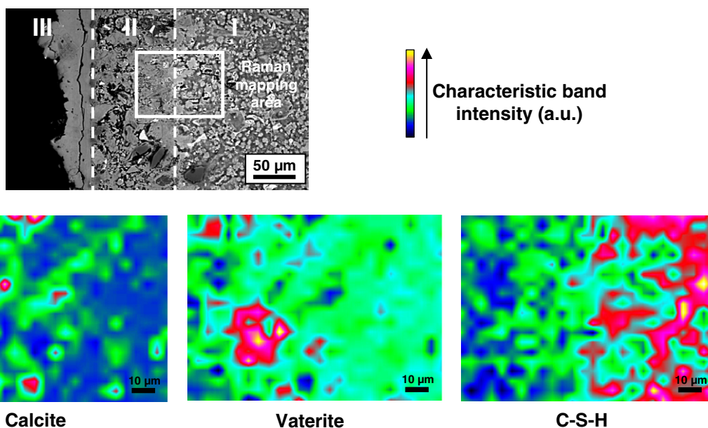
Fig. 5. Cement micro-Raman mineralogical mapping. Notes: The beams space step is 5 µm; the spectral windows chosen to distinguish the minerals are listed in Supplementary Data 5.
