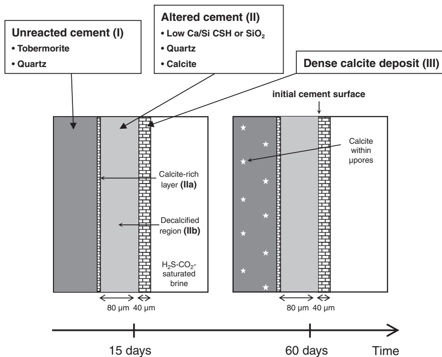
Fig. 6. Interpreted mineralogical profiles of cement at 15 and 60 days.
