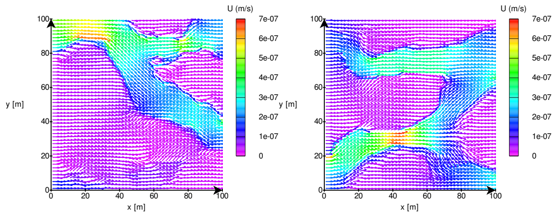
Figure 7: Darcy velocity field for the horizontal sections at z = 5 (left) and z = 35 m (right). Constant head boundary conditions are prescribed at the left (oxidized recharge) and right.
