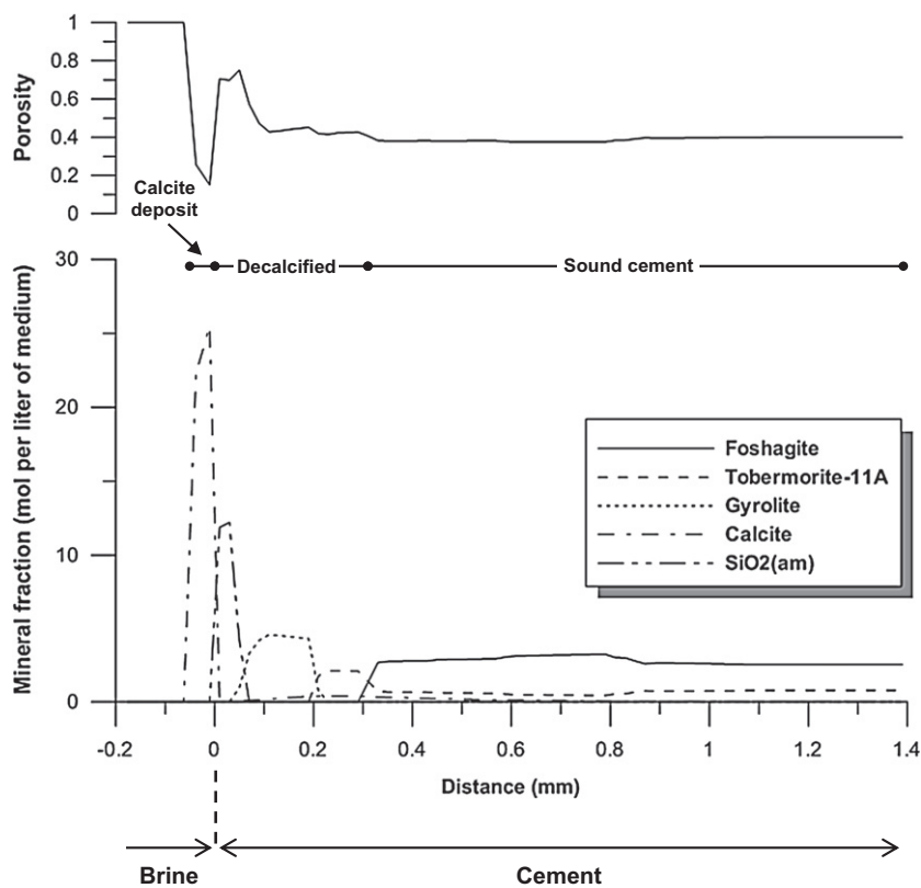
Fig. 7. Modelled mineralogical and porosity profiles of cement after 60 days of simulation. Notes: Foshagite: C_4S_3H_{1.5} ; Tobermorite-11A: C_5S_6H_{5.5} ; Gyrolite: C_2S_2H_{2.5} .
