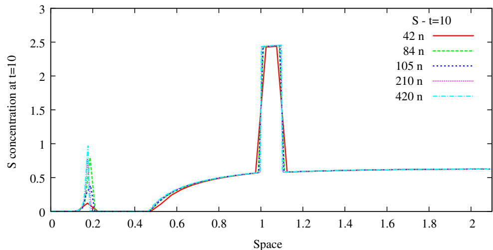
Fig. 12 Concentration profile for the dispersive easy 1D case of the fixed component S at t = 10
