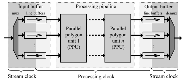
Fig. 11 Overall architecture of parallel ASF application.
