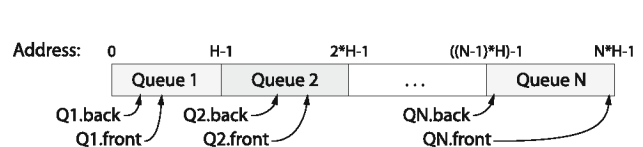
Fig. 6 Vertical queues are mapped into linear memory space side by side. The front and back pointers are stored at separated memory
