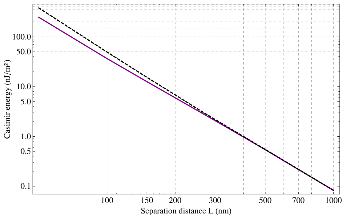
FIG. 41: Log-log dependence of the Casimir energy with the separation distance L , for two gratings of SiC described by the Drude-Lorentz model [65] given in equation (140). This is for a grating period d = 200 nm, filling factor p = 50\% , and groove depth a = 100 nm. These scattering results are compared with the Proximity Approximation (dashed line).
