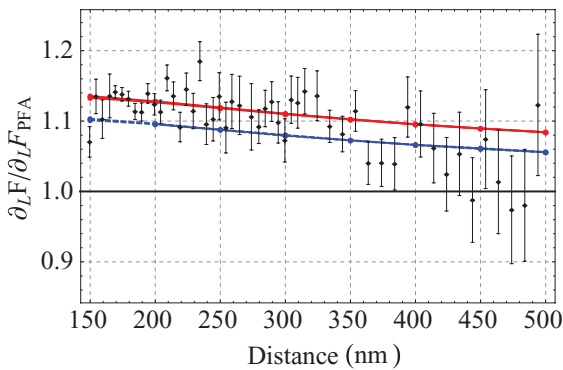
FIG. 7. (Color online) Experimental data for the Casimir force gradient between a gold sphere and a silicon grating with shallow trenches (black dots with error bars). The data are normalized to their PFA expression. This is compared with our calculations both for T = 0 K (blue) and T = 300 K (red).
