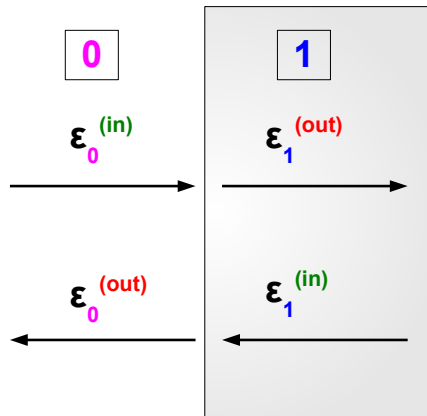
FIG. 15: Notations of the different fields propagating in and out of the interface according to the index of the material in which they travel. If we want to put the emphasis on the material in which the mode travels (as is done in the derivation of the Casimir energy between nanogratings), it is more convenient to use a S-matrix formalism according to equation (149). But if we want to put the emphasis on the direction of the propagation of the mode (as in the case of slabs, or coated materials), it is more convenient to use a T-matrix formalism according to equation (151).
