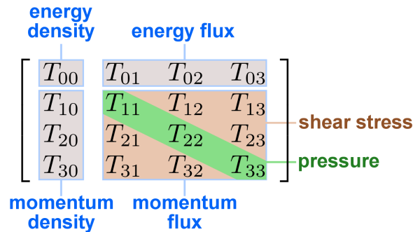
FIG. 19: Components of the general stress-energy tensor, with their physical meaning. The diagonal elements T_{11} , T_{22} , and T_{33} give the pressure responsible for the Casimir force. The shear stress is akin to viscosity.
