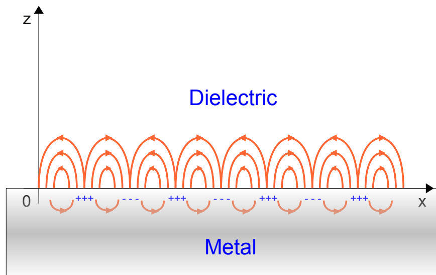
FIG. 28: Electric field lines and distributions of charges for a surface-plasmon located on the interface between a metal and a dielectric.
