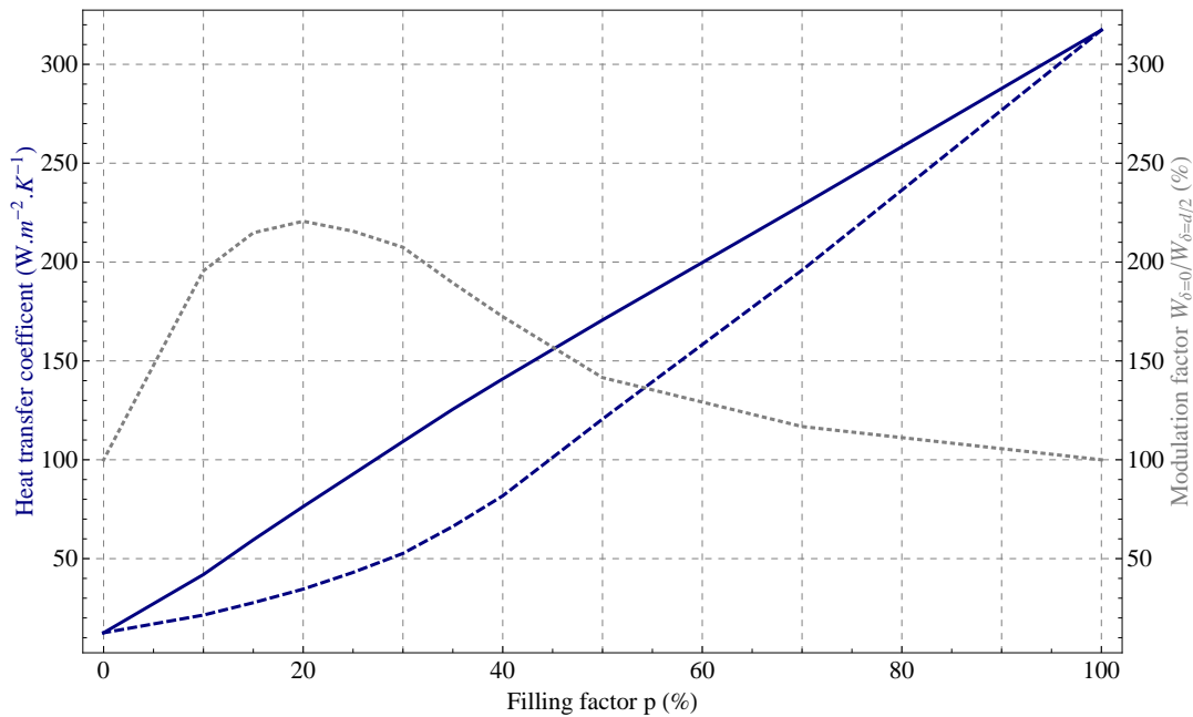
FIG. 118: Radiative heat transfer coefficient as a function of the filling factor p , for two gratings of silicon dioxide \text{SiO}_2 at temperatures T_1 = 310 K and T_2 = 290 K, for a lateral shift \delta/d = 0\% (blue curve) and \delta/d = 50\% (dashed blue curve). The results are plotted together with the percentage of modulation factor W_{\delta/d=0\%}/W_{\delta/d=50\%} (dotted gray line). The gratings have a period d = 500 nm, separation distance L = 100 nm, and groove depth a = 500 nm. The permittivity of \text{SiO}_2 is extrapolated from optical data [111, 112].
