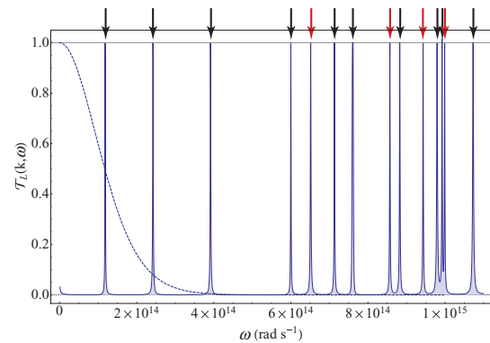
FIG. 4. (Color online) The transmission factor for two gold gratings with corrugation depth a = 1.5 \mu\text{m} as a function of frequency \omega . The arrows indicate the position of the modes in a direct mode calculation [red (gray) for s polarization and black for p polarization]. The dashed curve is the function \frac{eT_1 - eT_2}{k_B(T_1 - T_2)} .
