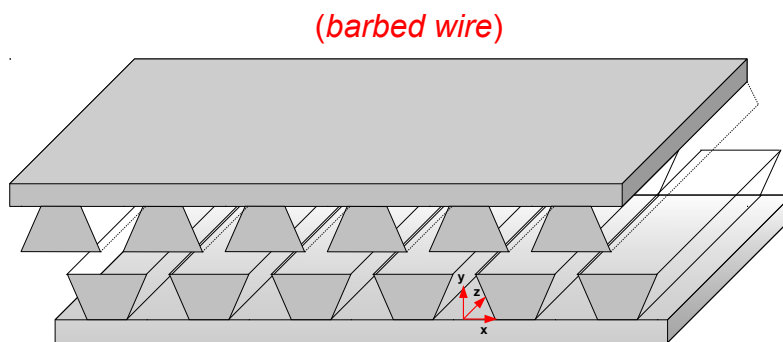
FIG. 76: Two-dimensional perspective on the barbed wire gratings used in FIG. 78, with same color code.
