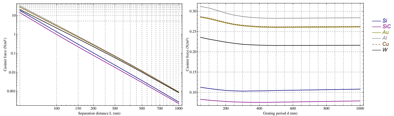
FIG. 64: Log-log dependence of the Casimir force with the separation distance L (left) and grating period d (right), for two gratings of different materials with period d = 200 nm (for left-hand plot), filling factor p = 50\% , groove depth a = 100 nm, and separation distance L = 200 nm (for right-hand plot). Intrinsic silicon appears in blue, and is described by the Drude-Lorentz model [27, 117, 150] given in equation (137). SiC appears in purple, and is described by the Drude-Lorentz model [65] given in equation (140). Gold appears in yellow, aluminum in gray, copper in dashed orange, and tungsten in black. These four metals are described by a Drude model [70] given by equation (135) and FIG. 11.
