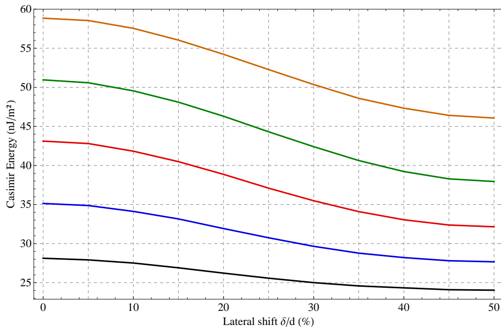
FIG. 74: Casimir energy as a function of the lateral shift \delta/d , for arbitrary periodic gratings of intrinsic silicon with separation distance L = 100 nm, period d = 400 nm, corrugation depth a = 50 nm, and number of slices K = 20 . Sawtooth grating with d_1 = 4y + 200 appear in black, with d_1 = 3y + 200 in blue, with d_1 = 2y + 200 in red, and with d_1 = y + 200 in green. This is compared with similar size rectangular corrugations d_1 = 200 in orange.
