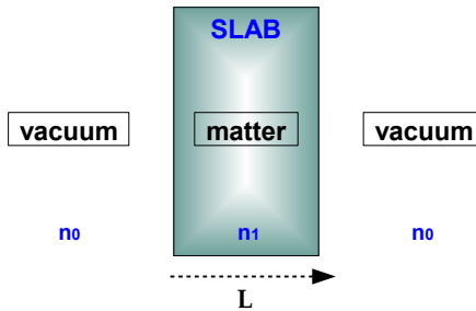
FIG. 16: Slab built by stacking a vacuum-matter interface, a propagation over a length \ell inside matter, and again a matter-vacuum interface.
