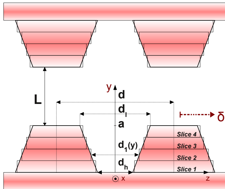
FIG. 35: Arbitrary gratings geometry and parameters in the approximation of vertical stacks of rectangular slices (here for K = 4 ).
