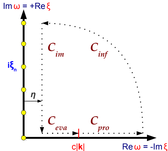
FIG. 23: Complex plane for which the expression of the Casimir force over real frequencies \omega at non zero temperature is switched to imaginary frequencies \xi . The quantities C_{eva} and C_{pro} correspond to the real evanescent and propagative waves, respectively, C_{im} represents imaginary frequencies, and C_{inf} represents the quarter circle with radius going to infinity. The major difference with FIG. 20 is the convergence factor \eta \rightarrow 0 appearing in the series of exponential (229) so that the imaginary frequencies are not on the pure imaginary axis but on z = i\xi + \eta . Also notice the equidistant poles of the Matsubara frequencies along \text{Im } \omega , including the one at \omega = 0 .
