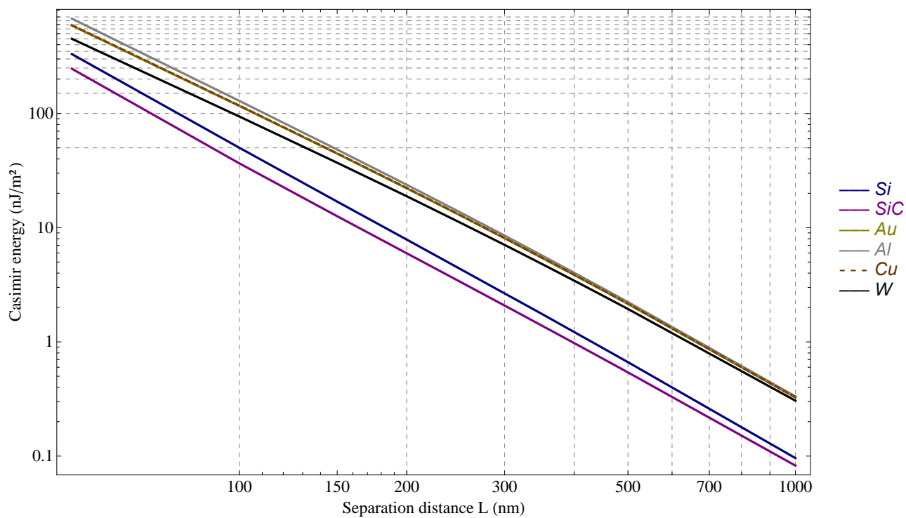
FIG. 44: Log-log dependence of the Casimir energy with the separation distance L , for two gratings of different materials with grating period d = 200 nm, filling factor p = 50\% , and groove depth a = 100 nm. Intrinsic silicon appears in blue, and is described by the Drude-Lorentz model [27, 117, 150] given in equation (137). SiC appears in purple, and is described by the Drude-Lorentz model [65] given in equation (140). Gold appears in yellow, aluminum in gray, copper in dashed orange, and tungsten in black. These four metals are described by a Drude model [70] given by equation (135) and FIG. 11.
