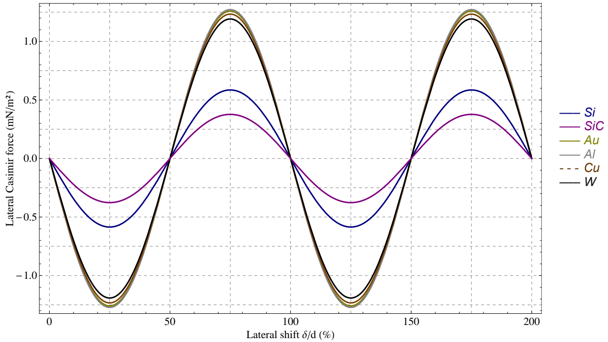
FIG. 69: Casimir lateral force as a function of the lateral displacement \delta/d , for two gratings of different materials with grating period d = 200 nm, filling factor p = 50\% , groove depth a = 100 nm, and separation distance L = 200 nm. Intrinsic silicon appears in blue, and is described by the Drude-Lorentz model [27, 117, 150] given in equation (137). SiC appears in purple, and is described by the Drude-Lorentz model [65] given in equation (140). Gold appears in yellow, aluminum in gray, copper in dashed orange, and tungsten in black. These four metals are described by a Drude model [70] given by equation (135) and FIG. 11.
