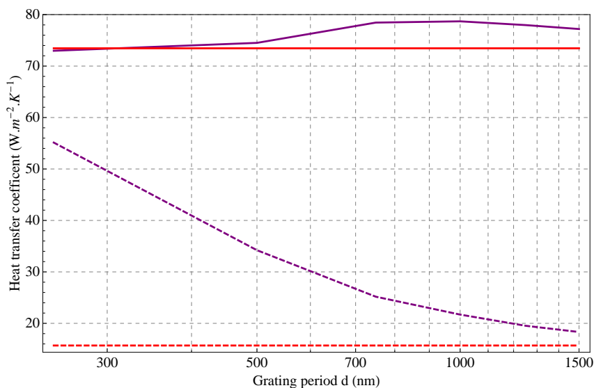
FIG. 114: Radiative heat transfer coefficient as a function of the grating period d , for two gratings of silicon dioxide \text{SiO}_2 at temperatures T_1 = 310 K and T_2 = 290 K, for a lateral shift \delta/d = 0\% (purple curve) and \delta/d = 50\% (dashed purple curve). These two scattering results are compared with the Proximity Approximation (respective red curves). The gratings are at a separation distance L = 100 nm, filling factor p = 20\% , and groove depth a = 500 nm. The permittivity of \text{SiO}_2 is extrapolated from optical data [111, 112].
