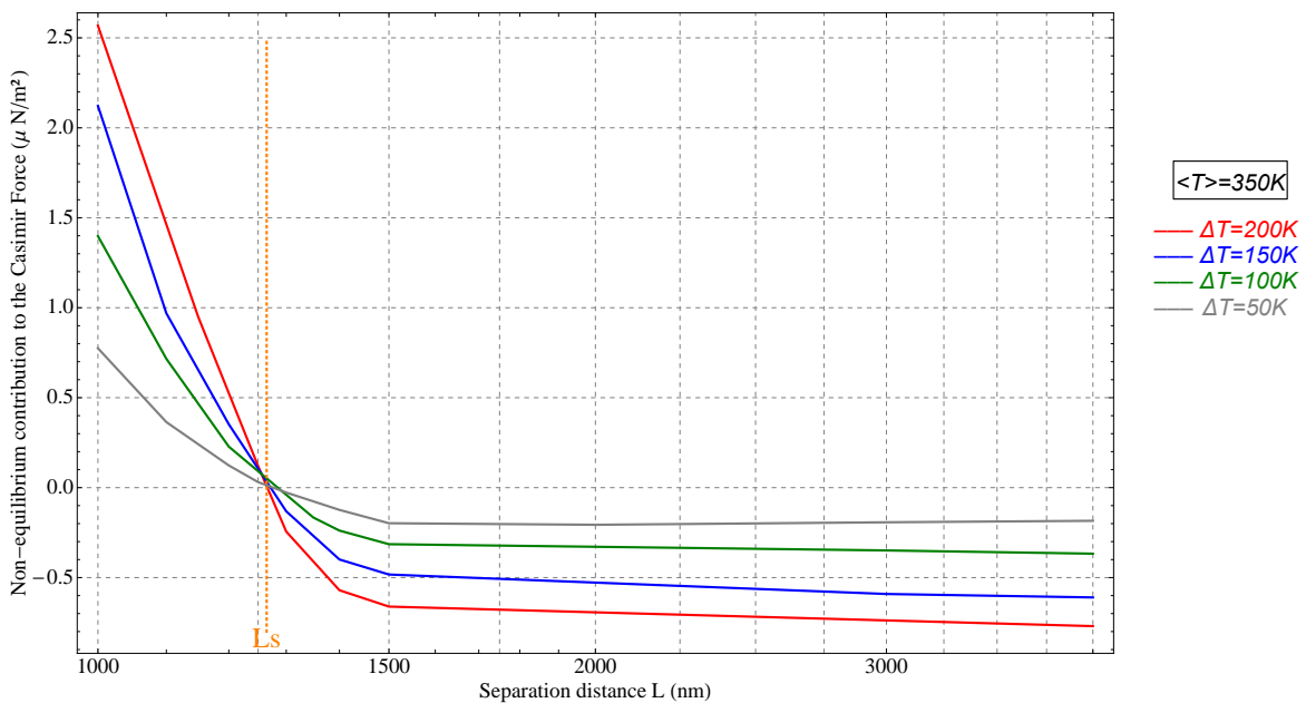
FIG. 106: Log-linear non-equilibrium contribution to the Casimir force \Delta F_z^{(\text{neq})}(T_1, T_2) from equation (376) as a function of the separation distance L , when the temperature average \langle T \rangle = 350 K is kept constant and for different temperature gradients : \Delta T = 200 K (red curve), \Delta T = 150 K (blue curve), \Delta T = 100 K (green curve), and \Delta T = 50 K (gray curve). This is for a Fabry-Pérot cavity formed by a plane of silicon dioxide \text{SiO}_2 at temperature T_1 = 350 - \Delta T/2 K, and a plane of silicon carbide \text{SiC} at temperature T_2 = 350 + \Delta T/2 K. The permittivity of \text{SiO}_2 is extrapolated from optical data [111, 112] and \text{SiC} is described by the Drude-Lorentz model [65] given in equation (140).
