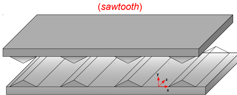
FIG. 73: Three-dimensional perspective on the sawtooth gratings.
