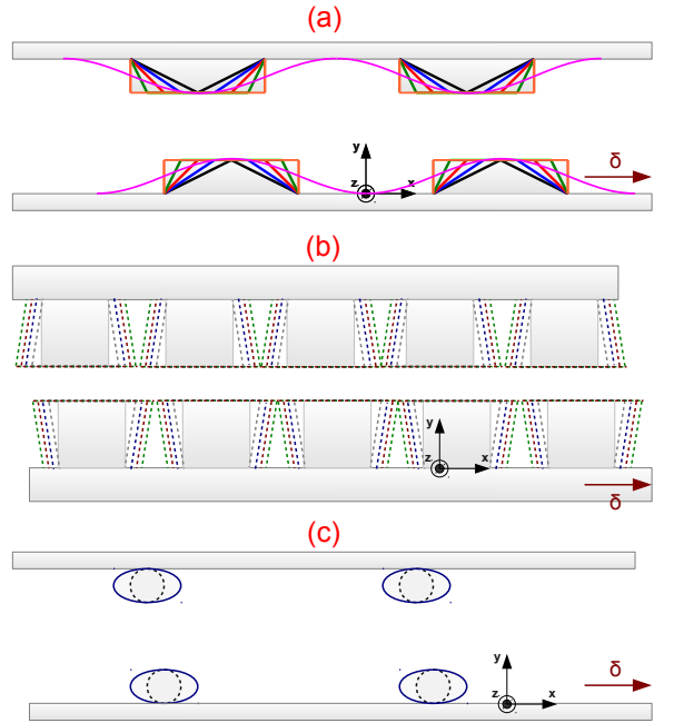
FIG. 2: Two-dimensional perspective on the different considered periodic gratings. (a) and (c) are at the same scale, but the scale of (b) has been increased by a factor two.
