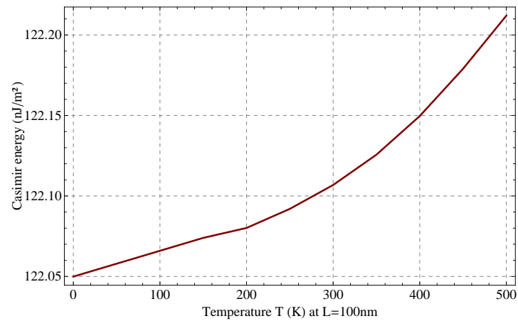
FIG. 90: Casimir energy as a function of the temperature T , for two planes of intrinsic silicon at a separation distance L = 100 nm. The material is described by the Drude-Lorentz model [27, 117, 150] given in equation (137).
