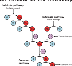
A biochemical system: the clotting cascade
