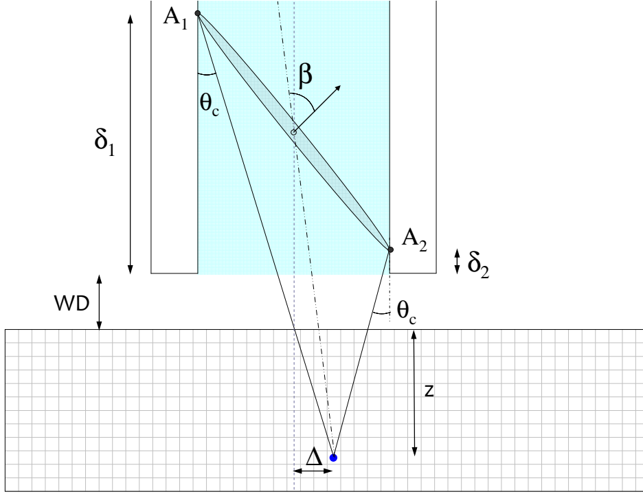
Fig. A2: System cross section presenting the case of fluorescence collection from B-type cells. Here the collection is not limited by the capillary edge (standard conditions).
