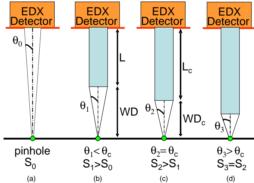
Figure IV.9: Scheme of the XRF detection from point source at various WD from the capillary extremity. (a) Classical XRF collection from a point source through a pinhole, (b) A capillary with identical radius is added, (c) the working distance is reduced to its critical value WD_c , (d) the WD is reduced below WD_c . At the bottom, expected variation of the signal S is reported.
