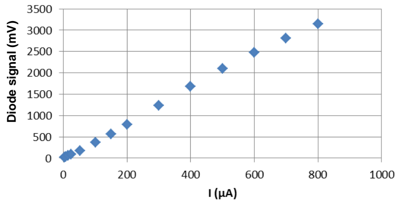
Fig III.3: Pin diode signal (proportional to the X-ray photon flux) variation as a function of the source current. The acceleration voltage is 35 kV.
