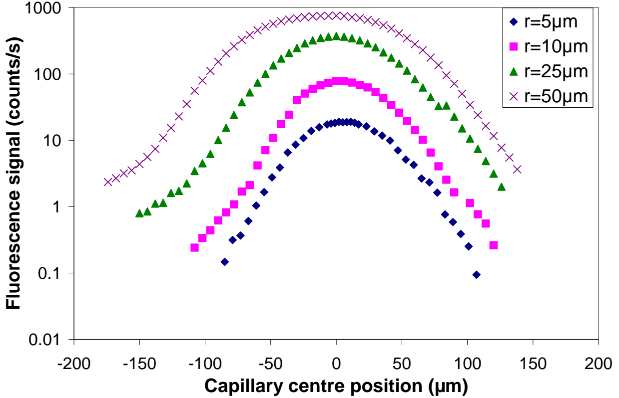
Fig.III.7: Cobalt fluorescence zone lateral profile represented by the K\alpha peak area as a function of the detection capillary position. The capillary radii are 5, 10, 25 \mu\text{m} and 50 \mu\text{m} .
