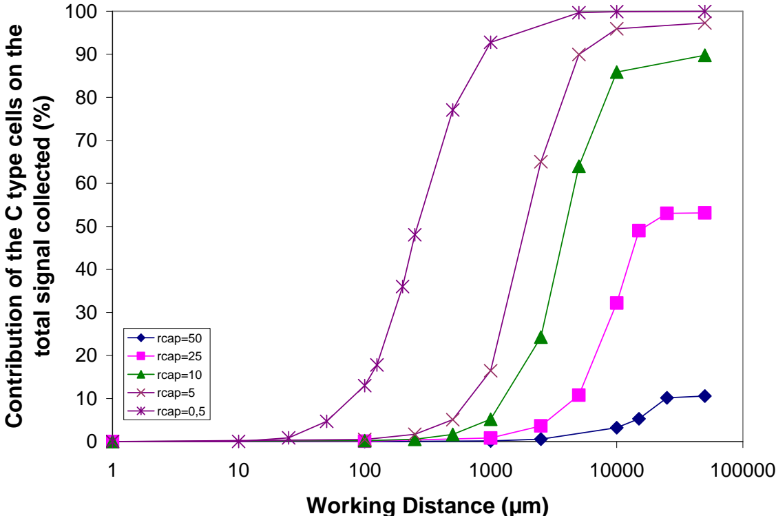
Fig.IV.16: Contribution of the C-type cells on the total signal collected as a function of the working distance. The capillary radius is 0.5, 5, 10, 25 and 50 \mu m . The line is a guide to the eyes
