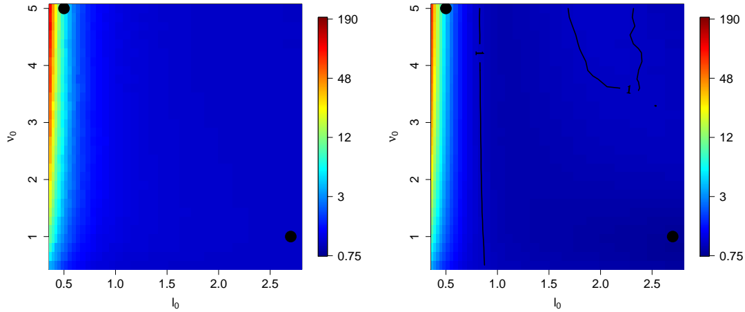
Figure 5.5: Estimation of \ell . Plot of the ratio of the asymptotic variance for \epsilon = 0 over the asymptotic variance for \epsilon = 0.45 for ML (left) and CV (right). The true covariance function is Matérn with varying \ell_0 and \nu_0 . The ML estimation is always improved by perturbing the regular grid, while the CV estimation can be damaged by perturbing the regular grid. We retain the two particular points (\ell_0 = 0.5, \nu_0 = 5) and (\ell_0 = 2.7, \nu_0 = 1) for further investigation below in this subsection 5.4 (these are the black dots).
