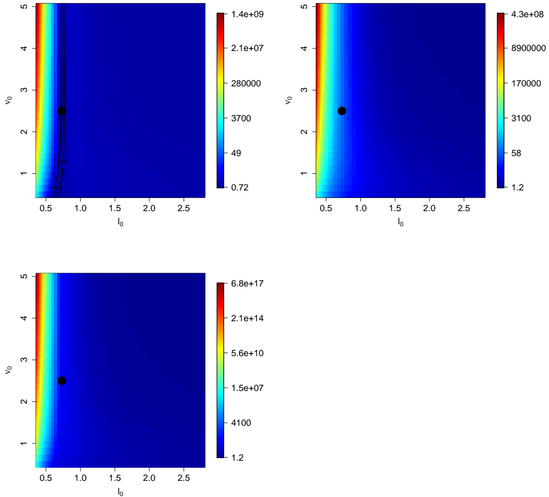
Figure 5.12: For ML, plot of the ratio, between \epsilon = 0 and \epsilon = 0.45 , of V_\ell (top-left), V_\nu (top-right) and D_{\ell, \nu} (bottom). The true covariance function is Matérn with varying l_0 and \nu_0 . We jointly estimate \ell and \nu . The asymptotic variance V_\ell increases with \epsilon for l_0 in a thin band, because this thin bands correspond to the case when, for \epsilon = 0 , the large uncertainty on \nu has no negative impact for the estimation of \ell . The asymptotic variance V_\nu always decreases with \epsilon . Furthermore, when V_\ell increases with \epsilon , V_\nu decreases considerably more. As a consequence, D_{\ell, \nu} always decreases with \epsilon , meaning that the joint estimation of \ell and \nu always benefits from an irregular sampling. We retain the particular point (l_0 = 0.73, \nu_0 = 2.5) for further investigation below in this subsection 5.4.3.
