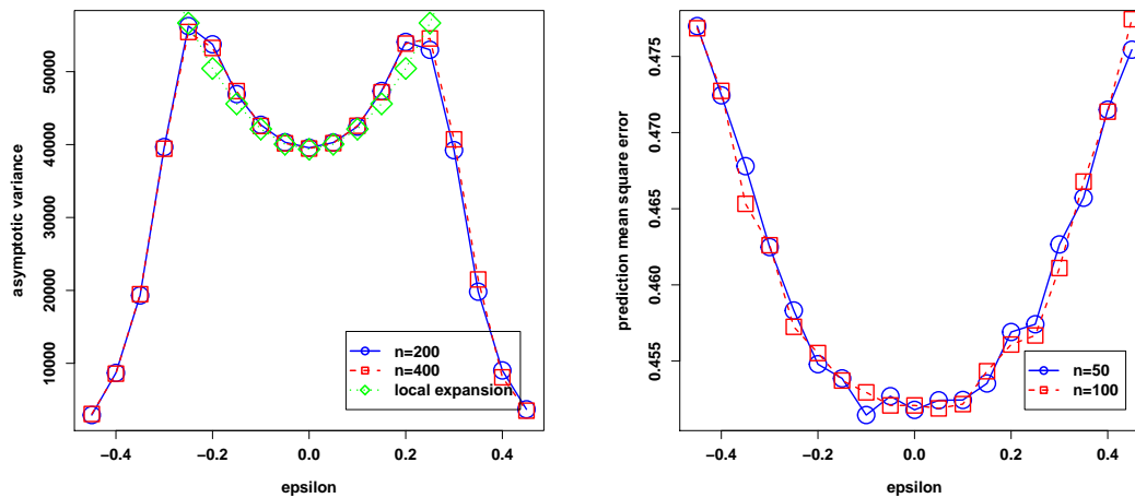
Figure 5.17: \ell_0 = 0.5 , \nu_0 = 2.5 . Left: asymptotic variance for the ML estimation of \nu , when \ell is known, as a function of \epsilon (same setting as in figure 5.9). Right: prediction mean square error \mathbb{E}(E_{\epsilon, \ell_0, \nu_0}) in proposition 5.21 as a function of \epsilon . There is no simple antagonistic relationship between the impact of the irregularity of the spatial sampling on estimation and on prediction
