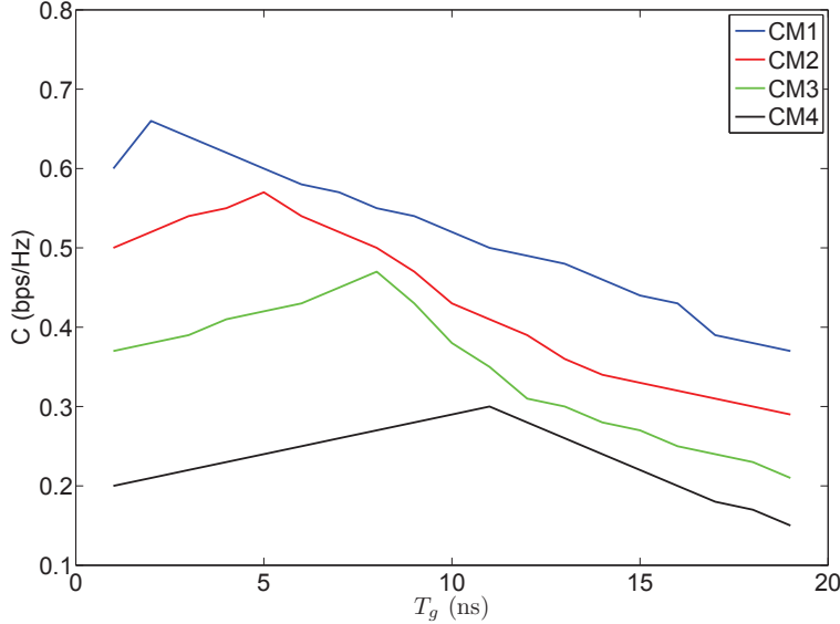
Figure 4.8: Capacity vs guard time
