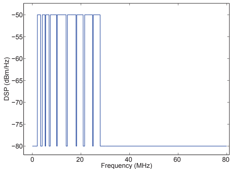
Figure 2.8: DSP mask for PLC systems
