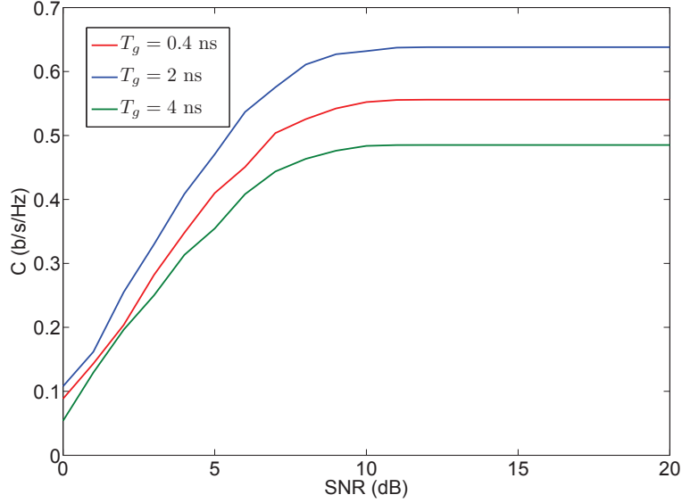
Figure 4.7: Capacity vs SNR over CM1 channel
