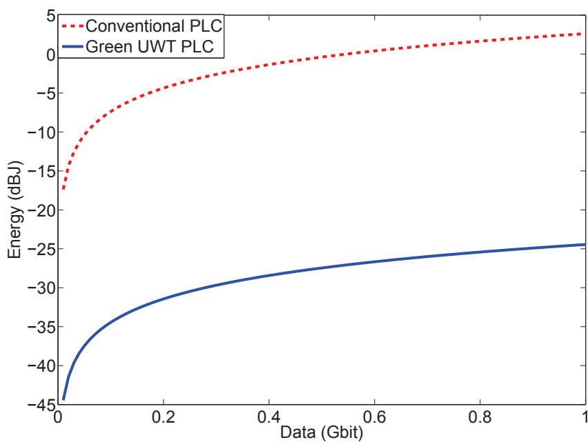
Figure 3.8: Energy consumption in PLC
