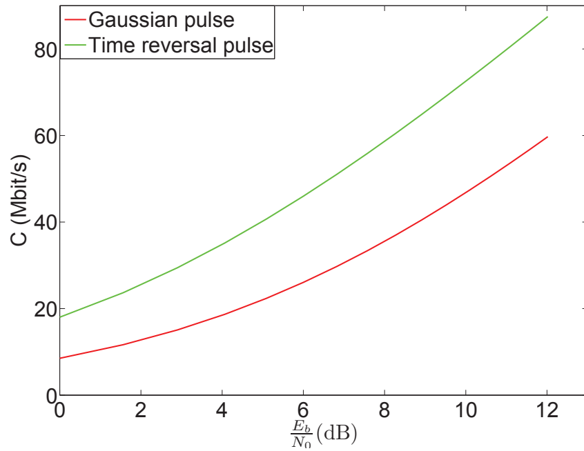
Figure 5.4: System capacity vs E_b/N_0
