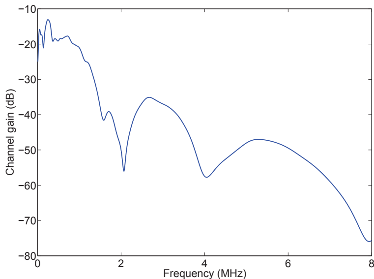
Figure 2.7: Transfer function of the reference model proposed by Zimmermann PLC channel
