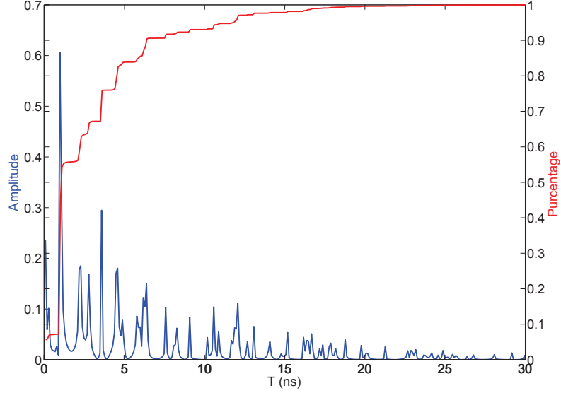
Figure 4.6: An example of multi-path CM1 channel impulse response and the CDF of the received energy
