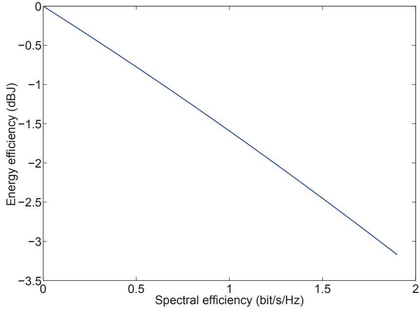
Figure 3.2: Relationship between spectral efficiency and energy efficiency.
