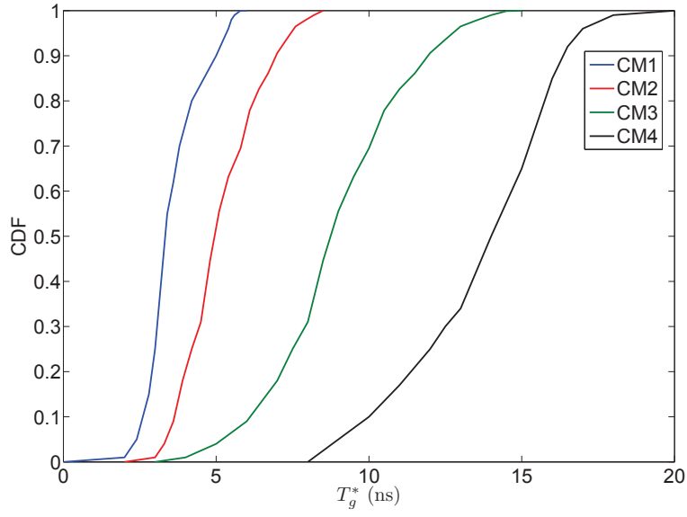
Figure 4.9: CDF of the optimal capacity
