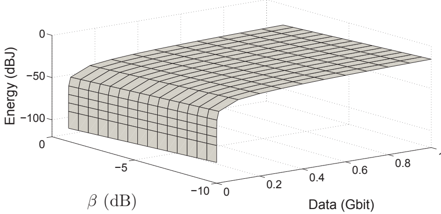
Figure 3.6: Energy vs energy efficiency and quantity of information
