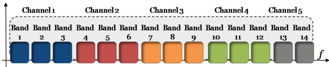
Figure 2.5: UWB spectrum bands in the MB-OFDM system
