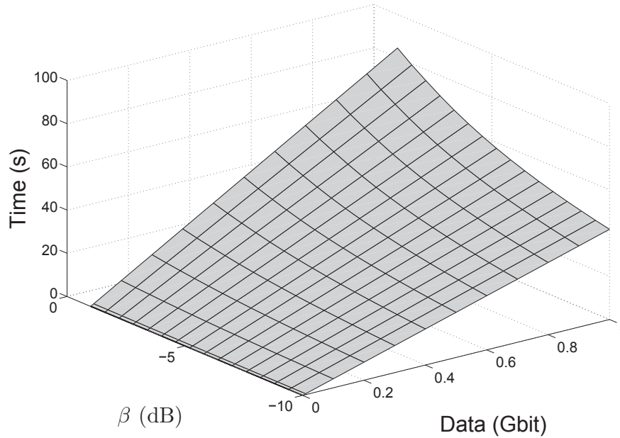
Figure 3.7: Time vs energy efficiency and quantity of information
