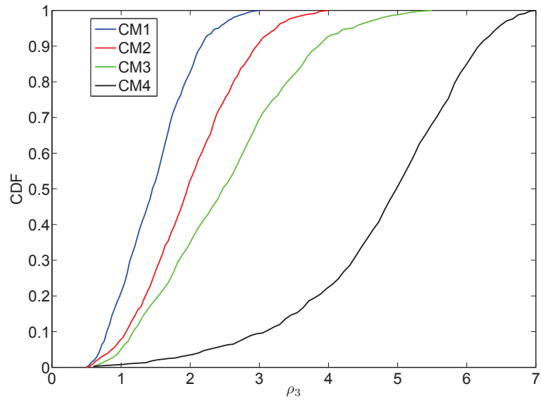
Figure 4.12: CDF of parameter \rho_3
