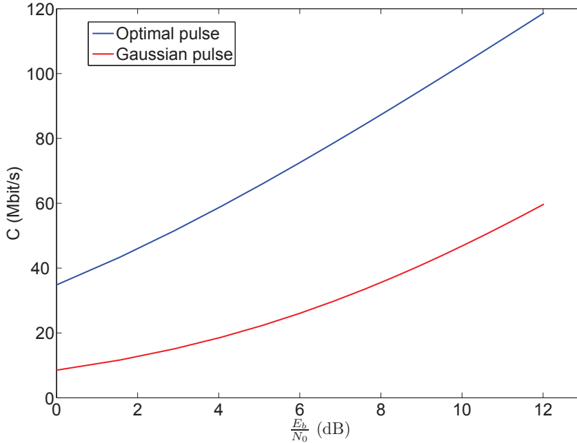
Figure 5.7: System capacity vs \frac{E_b}{N_0}
