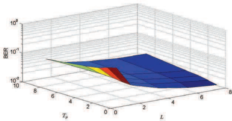
Figure 4.5: BER vs T_p and L
