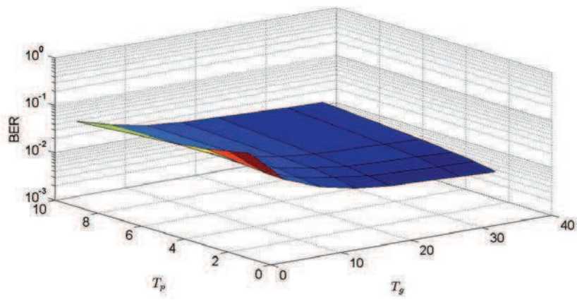
Figure 4.4: BER vs T_p and T_g
