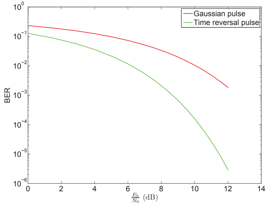
Figure 5.3: BER vs E_b/N_0
