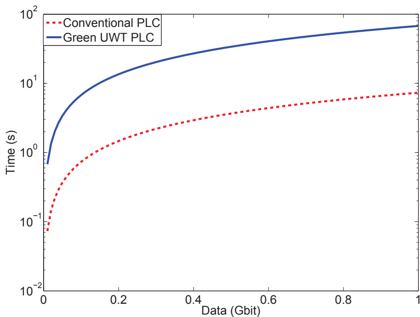
Figure 3.9: Time of transmission in PLC
