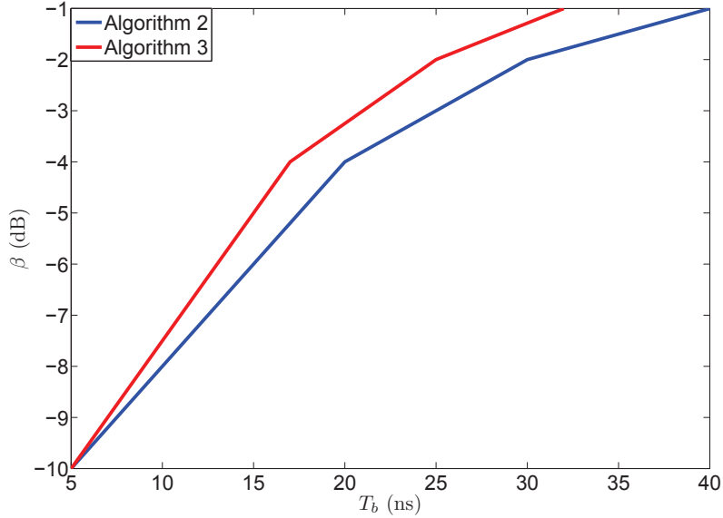
Figure 4.17: Energy efficiency vs the bit duration T_b
