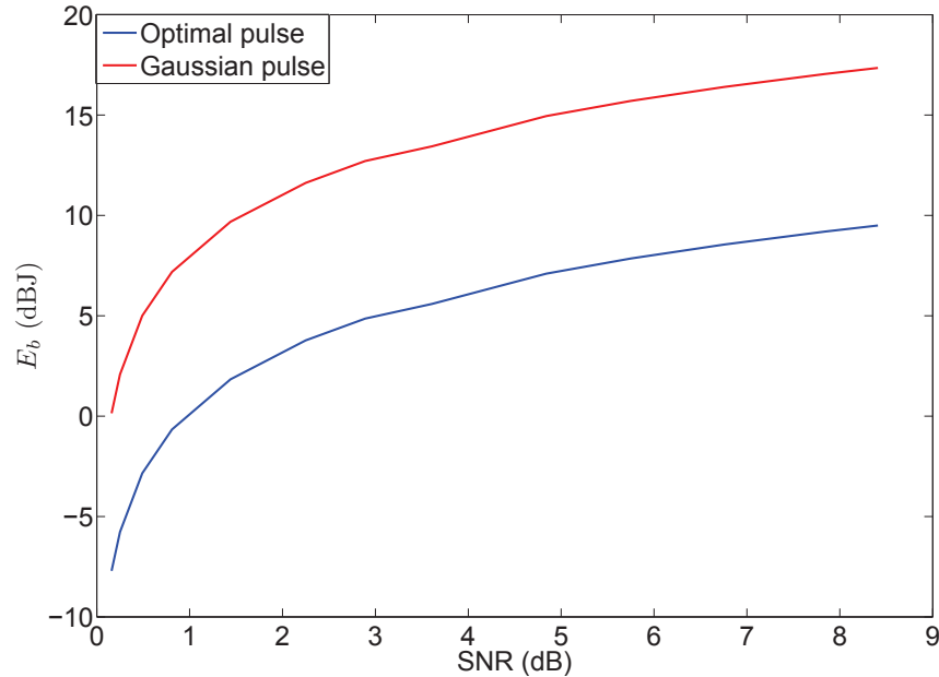
Figure 5.6: SNR vs Energy of bit
