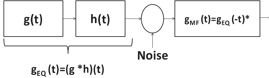
Figure 2.4: The mathematical model
