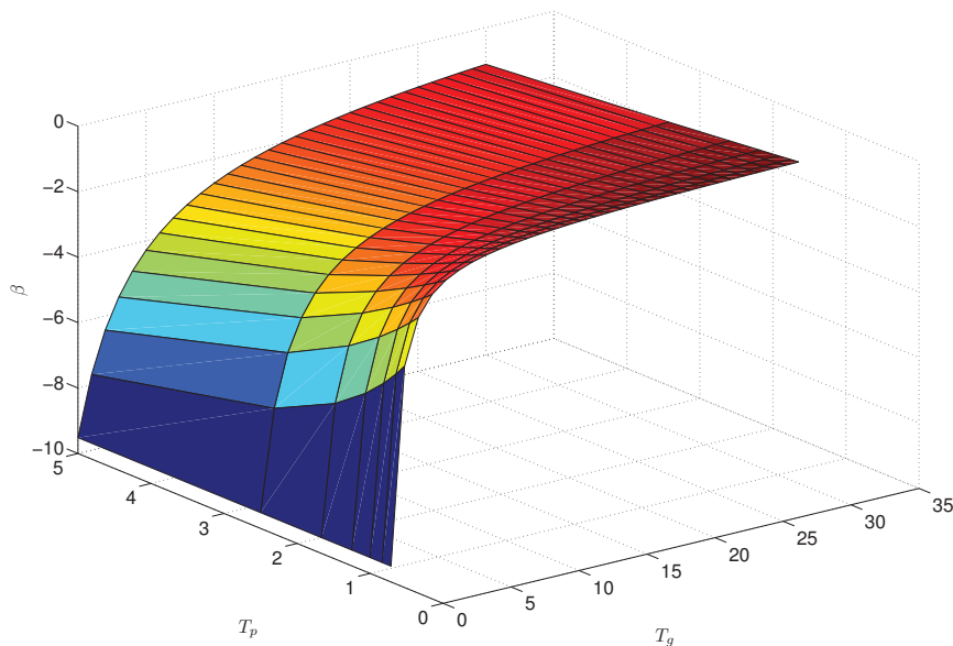
Figure 4.3: Energy efficiency vs the pulse time and guard time
