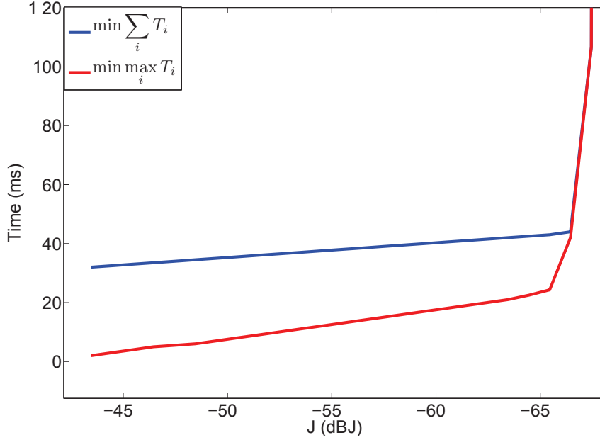
Figure 3.3: Pareto border of energy minimization
