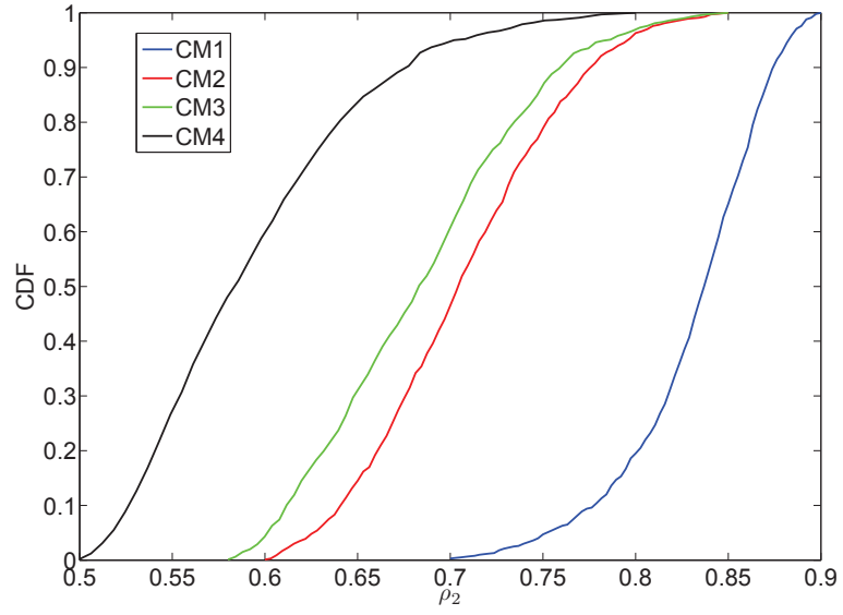
Figure 4.11: CDF of parameter \rho_2
