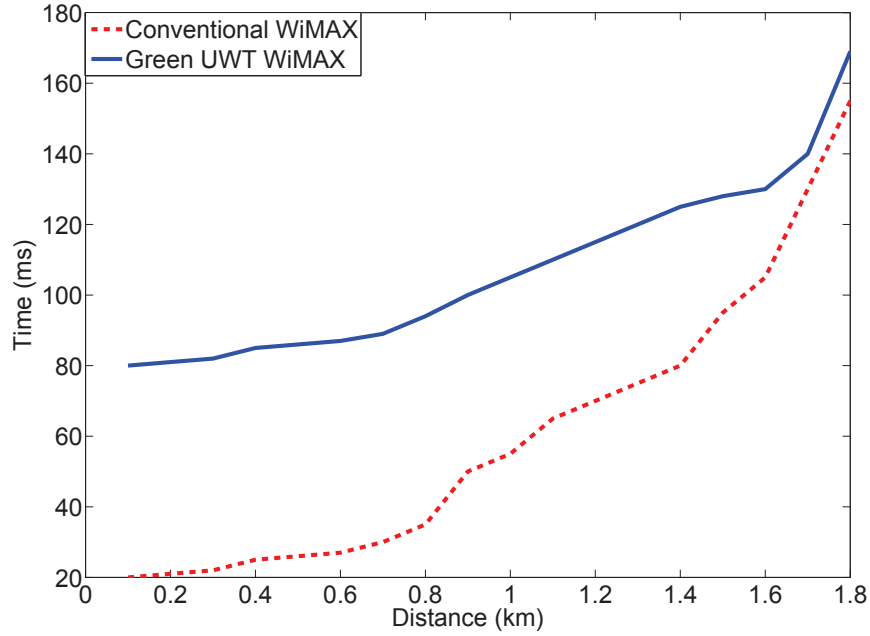
Figure 3.5: Transmission time with WiMAX systems
