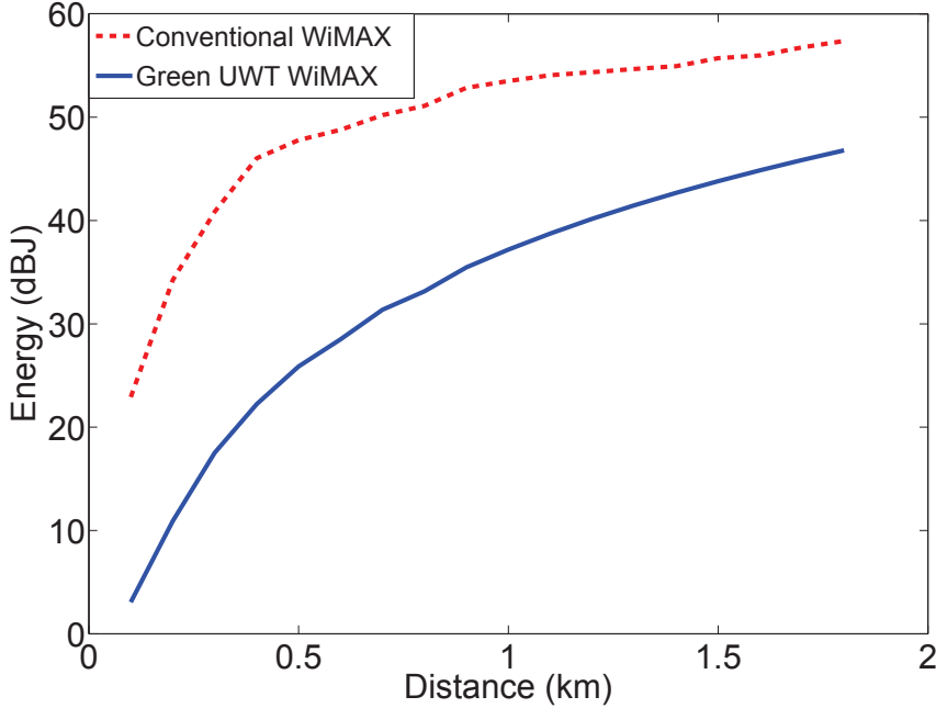
Figure 3.4: Energy consumption of WiMAX systems
