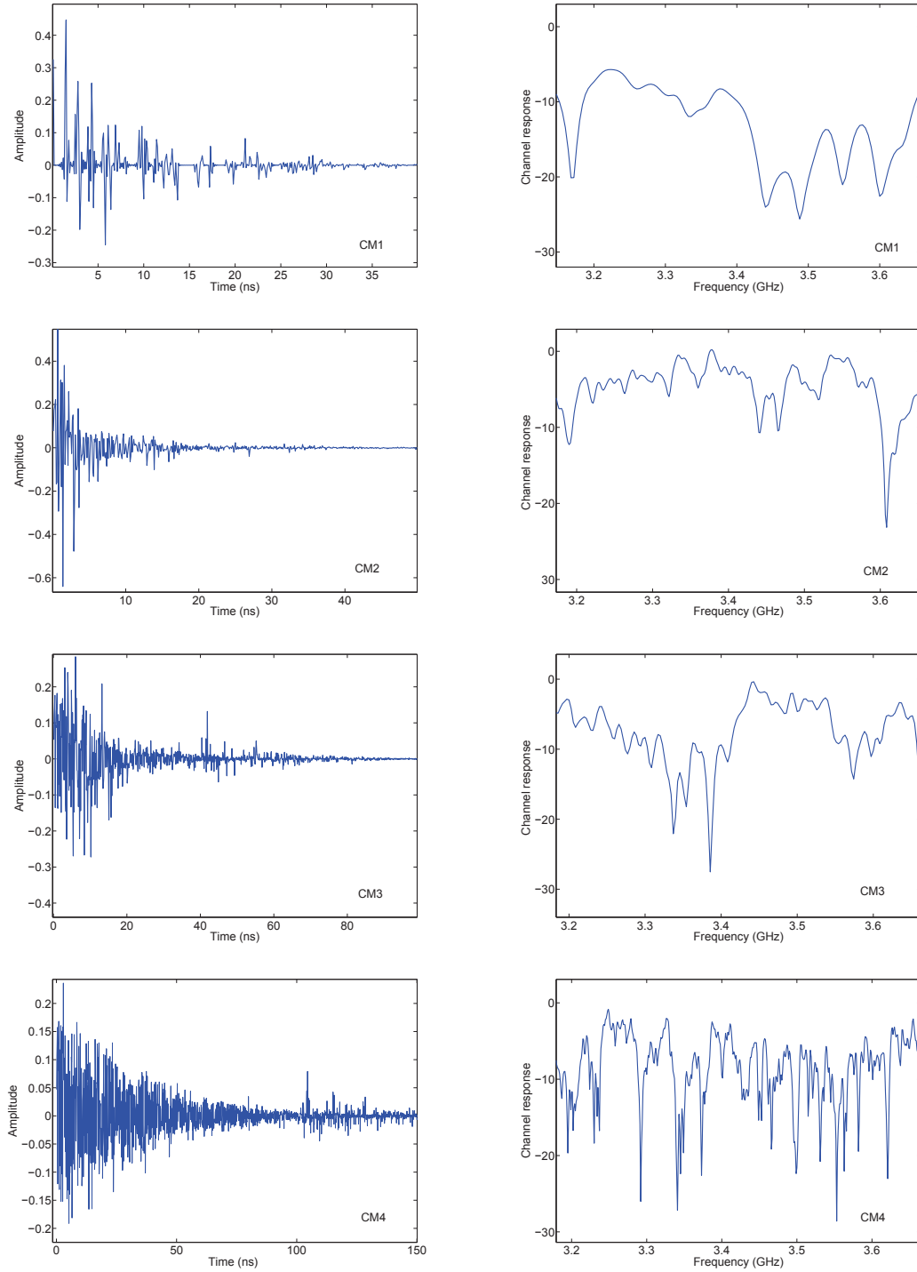
Figure 2.10: Example of UWB channel realizations for models CM1, CM2, CM3, CM4, in time and frequency domains
