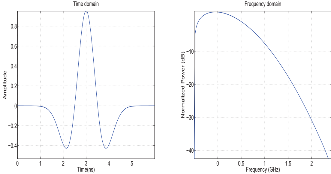
Figure 2.2: Time and Frequency domain for Second-order Gaussian mono cycle
