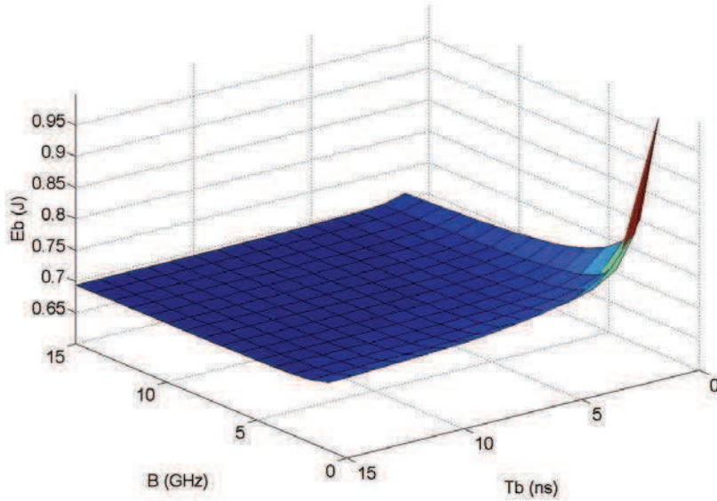
Figure 4.1: Energy vs bandwidth and bit duration
