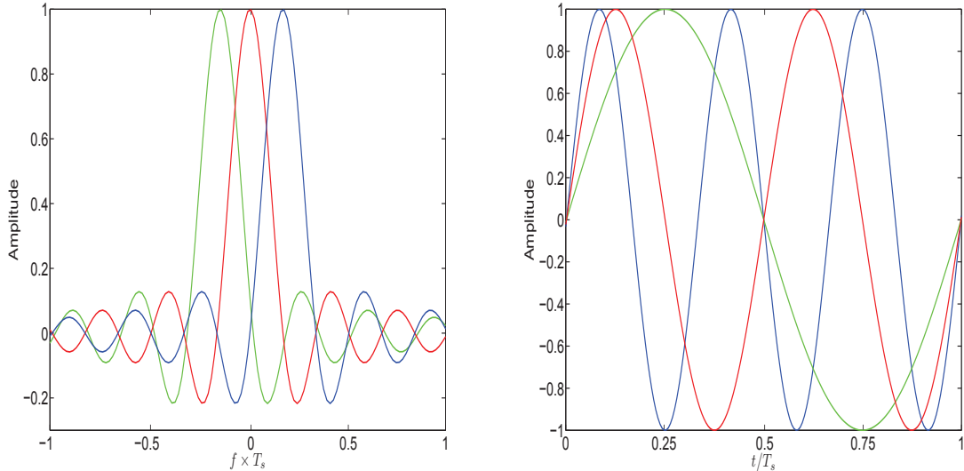
Figure 2.1: Frequency and Time domain representation of an OFDM signal
