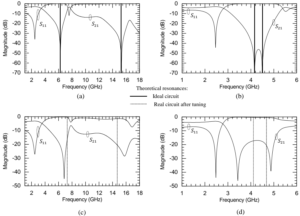
Figure III.16: Electric simulation of the power dividers with (a) R=105 \Omega and (b) R=150 \Omega and electromagnetic simulation on Momentum with (c) R=105 \Omega and (d) R=150 \Omega .
