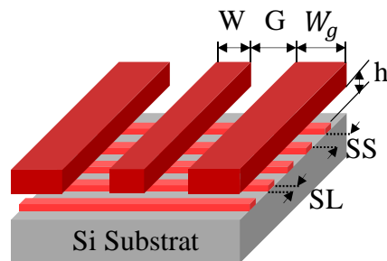
Figure I.24 : S-CPW topology.
