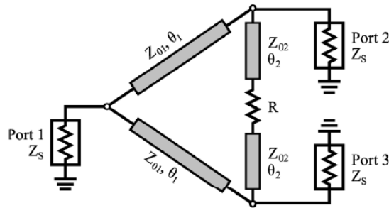
Figure III.1: Modified power divider with resistance access proposed in [80].
