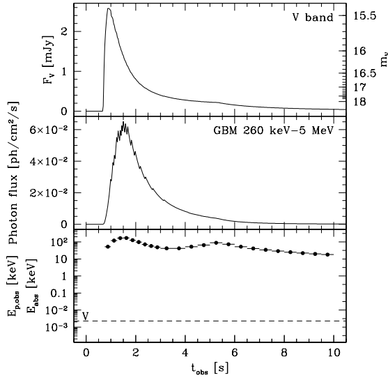
Fig. 5. Comparison between the temporal evolution of the optical and gamma-ray emission in internal shocks: case C. Same as in the left panel of Fig. 3 for the third example of GRB pulse discussed in Daigne et al. (2011) (Case C). E_{\text{obs}} is much lower than the optical frequency and does not appear in the bottom panel.
