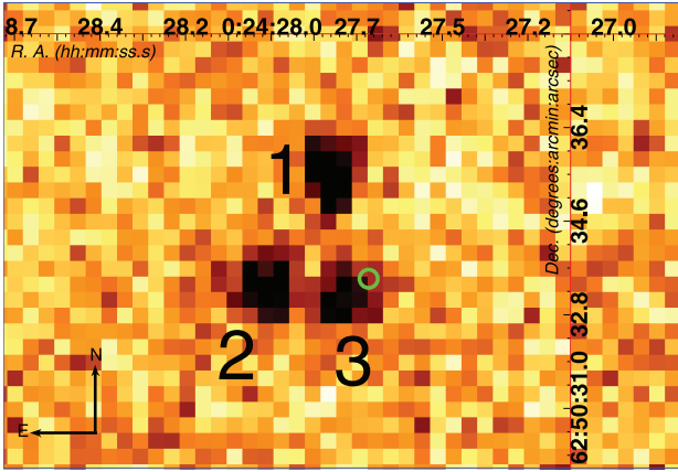
Figure 5. CFHT/WIRCcam K_s -band image of the region around GRB 041219A. The circle represents the position of the GRB infrared flash, as derived by Blake et al. (2005). The black labels correspond to the three objects discussed in the text.
