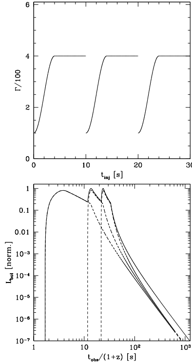
Fig. 2. Early steep decay from high latitude emission in the internal shock framework: a multi-pulse burst. Top: initial distribution of the Lorentz factor; Bottom: bolometric light curve on a logarithmic scale (solid line). The contribution of each individual pulse is plotted as a dashed line.
