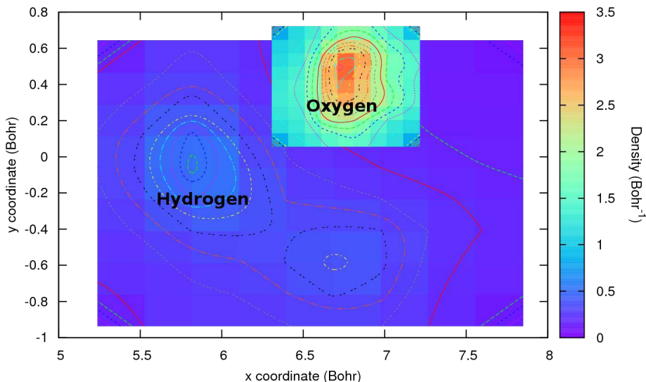
Figure 6.2: Density of presence (per Bohr) of one oxygen and one proton in a plane ( xOy ).
