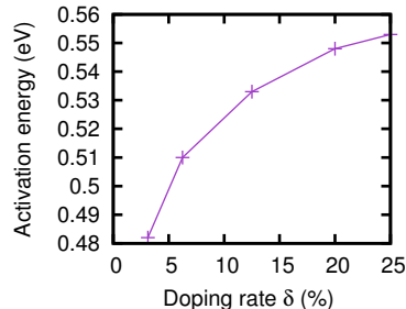
Figure 5.6: Activation energy of oxygen vacancy as a function of the dopant concentration.
