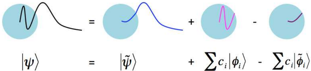
Figure 1.2: PAW transformation.
