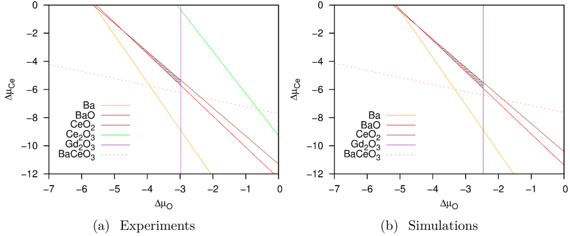
Figure B.1: Thermodynamics stability diagram as a function of O and Ce chemical potentials, in the plane \Delta\mu_{Gd} = -5 eV. Hatched area corresponds to the stable zone of BCGO (without considering the precipitation of \text{BaCeO}_3 ).
