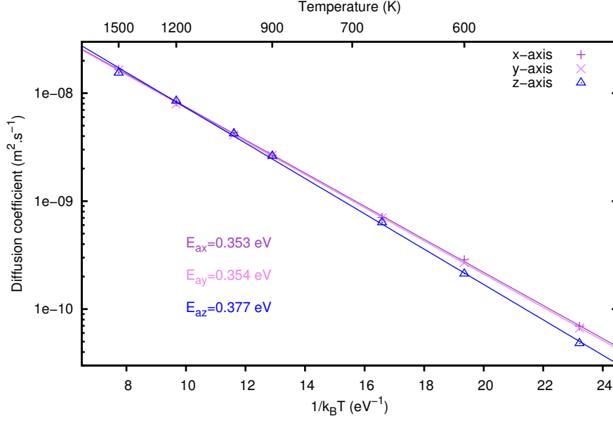
Figure 5.9: Diffusion coefficient, calculated from protonic mobility, along the a, b and c-axis as a function of temperature.
