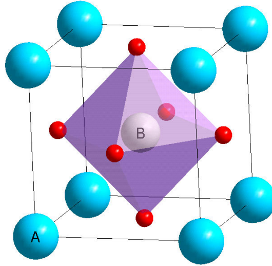
Figure 0.3: Primitive cell of an ideal (cubic) perovskite structure (5 atoms).
