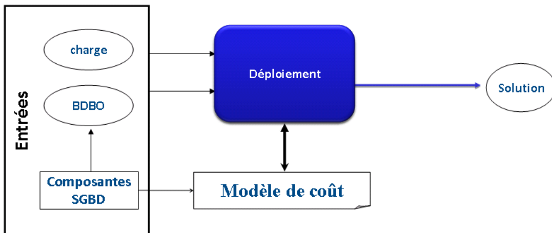
FIGURE 6.6 – Solution exhaustive
