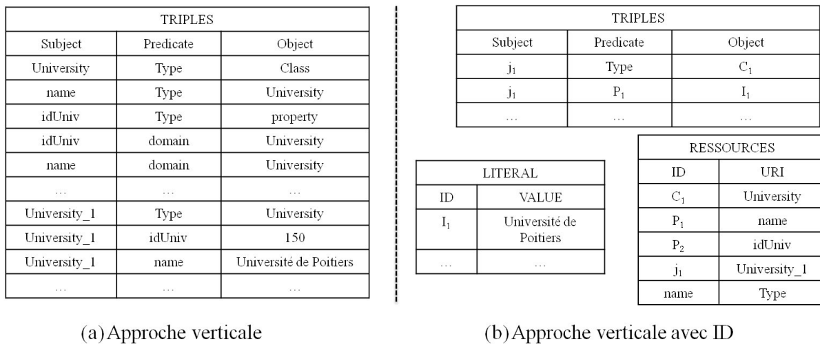
FIGURE 2.2 – Illustration de l'approche verticale.
