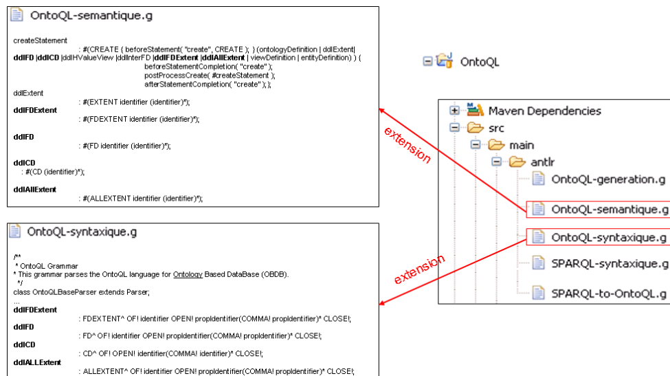
FIGURE 7.22 – Extension du langage OntoQL
