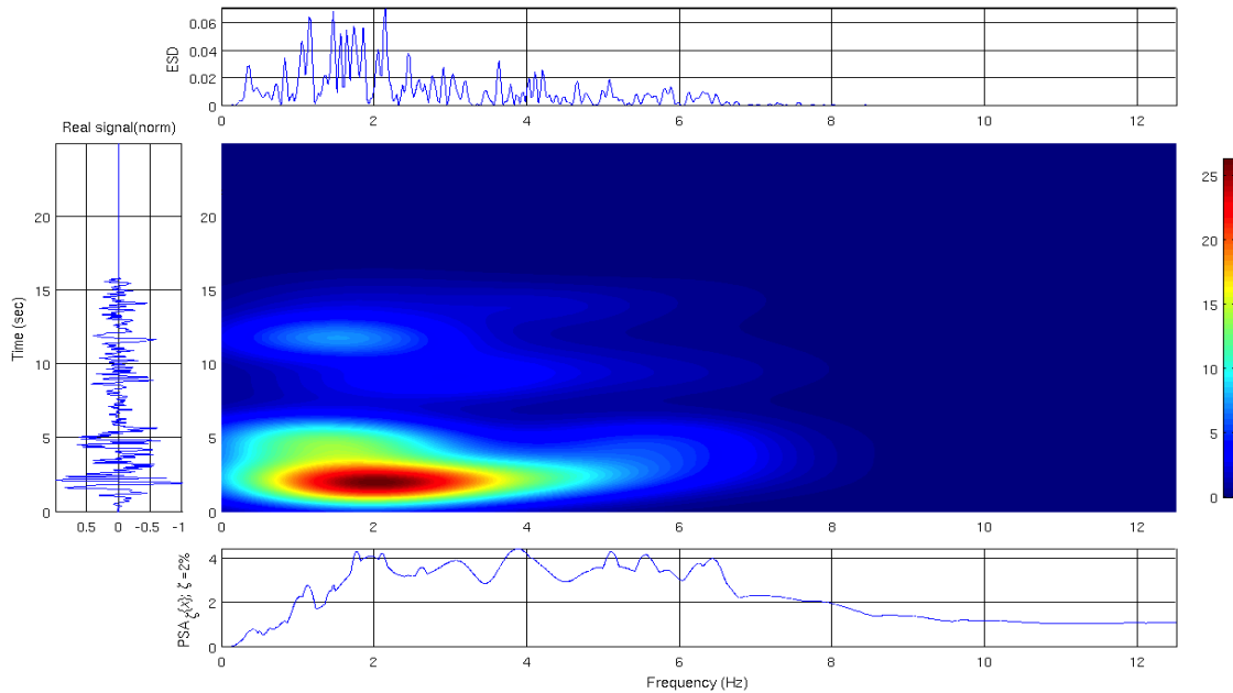
Figure 2.7 – DWVLsa du signal sismique (normalisé) El Centro. T = \sqrt{2} , \Omega = 2\sqrt{2}\pi
