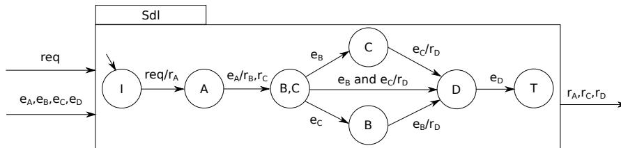
Figure 5.5: Scheduler automaton Sdl capturing application execution behaviours.
