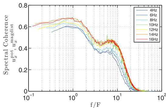
FIG. 8. (Color online) Spectral coherence between the reference potential probe u_x^{\text{pot}} and the magnetic-distortion probe u_x^{\text{mag dist}} as a function of frequency f normalized to the impellers rotation rate F in the counter-rotating regime. Increasing rotation rate F are referred in the inset.
